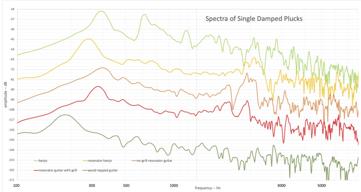
FIG. 7: spectra of the five damped-string plucks at four times lower resolution and successively offset by 20 dB
