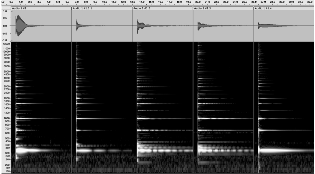
FIG. 8: wave forms and spectrograms of the five mid-string plucks – no strings damped
