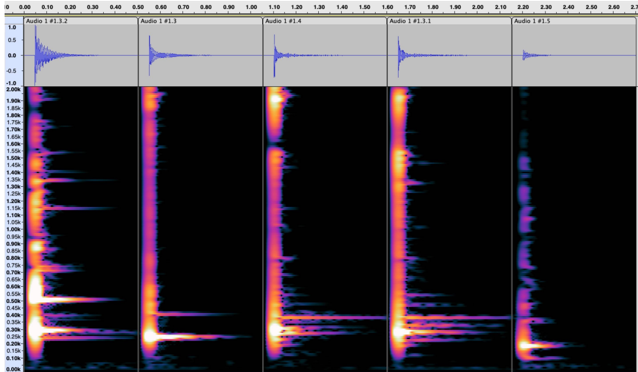
FIG. 5: wave forms and spectrograms of the five damped-string plucks at the bridge
