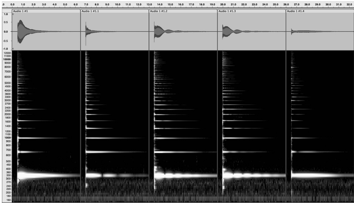
FIG. 10: 1 st string pluck at 12th fret, tailstrings & all other strings damped, mic at 4'
