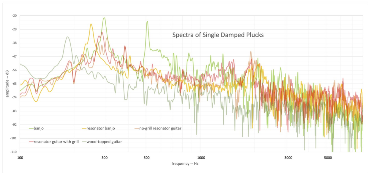
FIG. 6: spectra of the five damped-string plucks at the lowest resolution that represents actual individual peaks
