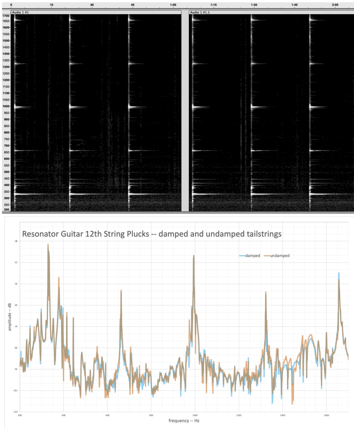
FIG. 9: spectrogram and spectra for plucks on the resonator guitar with cone cover grill and all tailstrings damped on the left and undamped on the right
