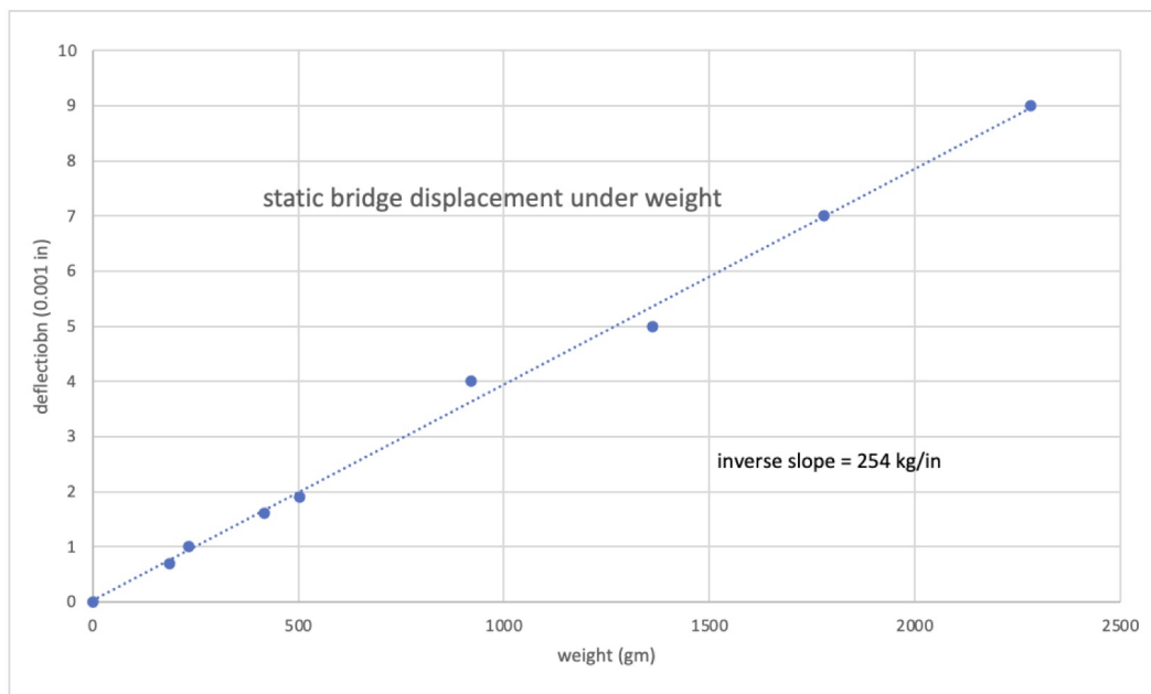
FIG. 14: measurements of static bridge displacement on the resonator banjo
