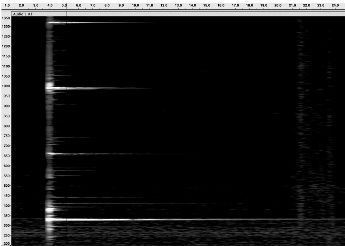
FIG. 13: covered resonator guitar, all open strings, pluck at 12th fret, mic at 4'
