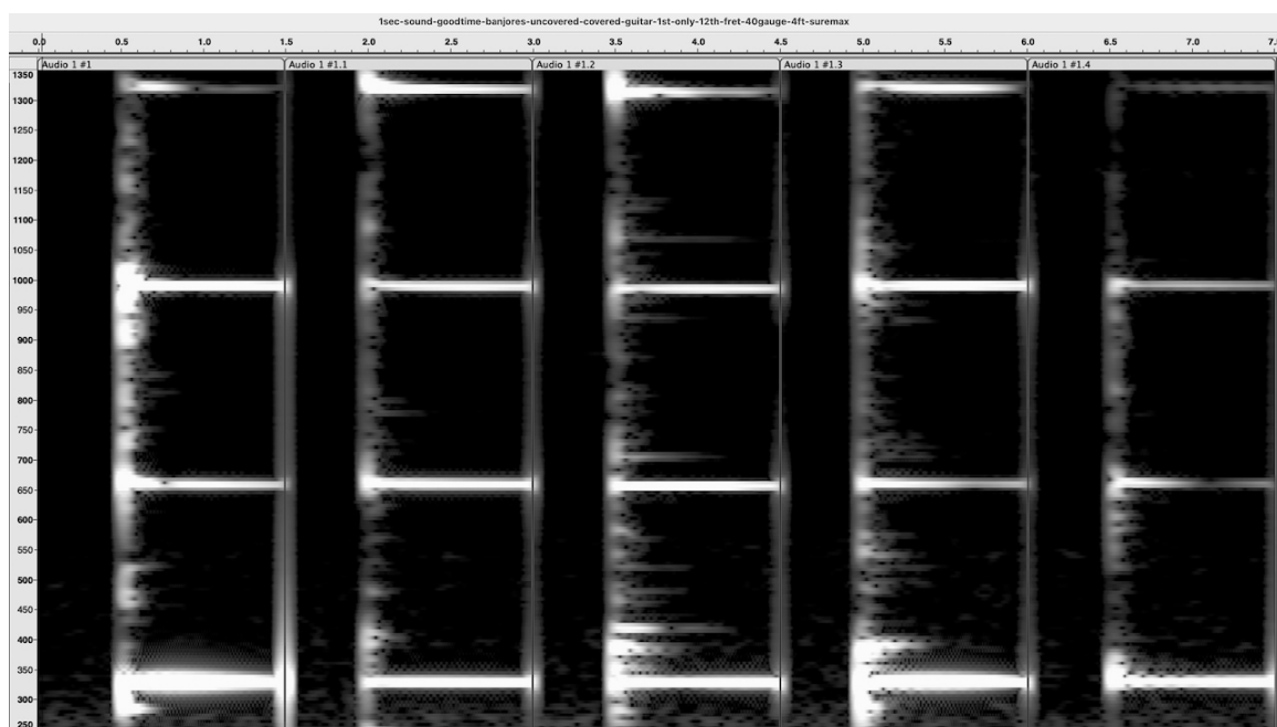
FIG. 11: 1 st string pluck at 12th fret, tailstrings & all other strings damped, mic at 4'
