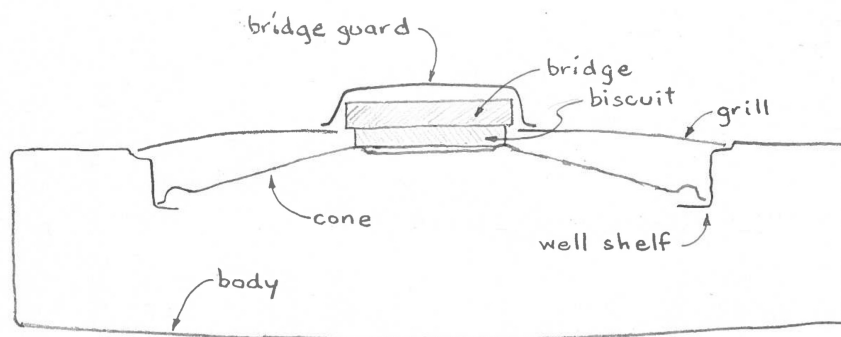
FIG. 3: single-cone (& biscuit) resonator guitar cross section – to scale
