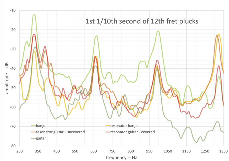
FIG. 12: 1 st string pluck at 12th fret, tailstrings & all other strings damped, mic at 4'
