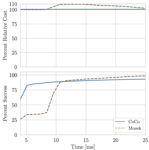
Fig. 8: We compare the performance of CoCo (blue) and Mosek (brown) after timing out both on a test set of MIQCQPs. We see in the bottom plot that timing out Mosek leads to a reduced number of feasible solutions found compared with CoCo. As the cutoff time increases, we see in the top plot that if Mosek finds a feasible solution, then these feasible solutions are suboptimal compared to CoCo, which generally finds the globally optimal solution even when timed out early.
