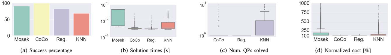
Fig. 3: For the cart-pole system, CoCo finds near-global solutions for a majority of problems.
