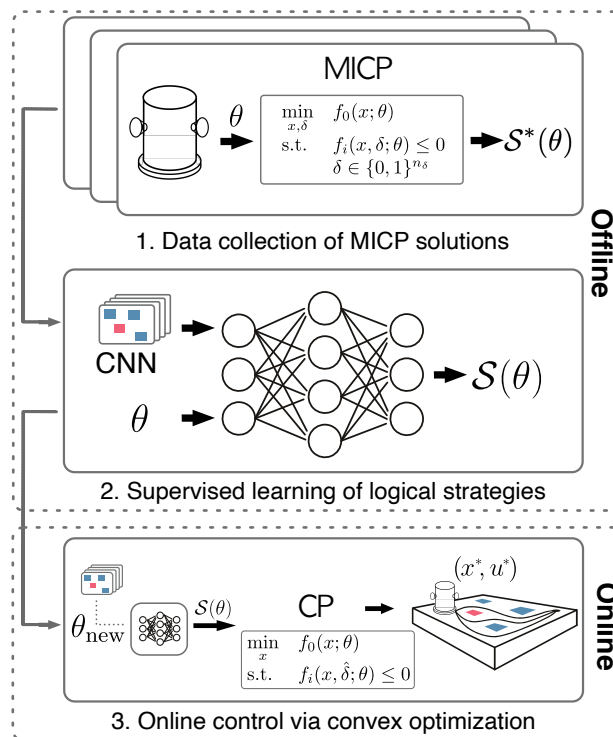
Fig. 1: Our algorithm CoCo is a data-driven approach that seeks to accelerate finding high-quality solutions to parametrized MICPs. The approach proposes a logical strategy \hat{S}(\theta) , which is a candidate discrete solution \hat{\delta} satisfying the logical constraints of the system. Given \hat{\delta} , the MICP can be approximately solved as a convex optimization problem. Here, we show CoCo applied to the free-flying spacecraft robot motion planning problem. (1) Offline, CoCo solves a set of MICPs for a representative set of planning problems and constructs the optimal logical strategy S^*(\theta) using the discrete optimizer \delta^* and set of relaxed constraints \mathcal{T}_M(\theta) . (2) Thereafter, a convolutional neural network classifier is trained to learn a mapping between problem parameters \theta and the logical strategy S^*(\theta) . (3) Online, this classifier predicts the logical strategy \hat{S}(\theta) associated with new parameters \theta and uses the candidate discrete solution \hat{\delta} to solve convex optimization problems until a feasible solution is found.
