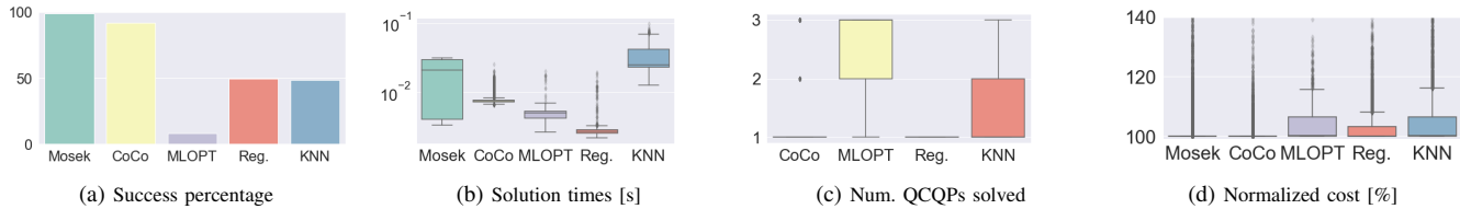
Fig. 6: Simulation results for the free-flyer show how task-specific strategies are necessary for using CoCo.
