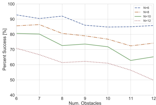
Fig. 7: Generalization results for a CoCo strategy classifier network demonstrates roughly linear dropoff in performance as obstacles are added. The strategy classifier network was trained on an environment with N_{\text{obs}} = 8 for various horizons N .
