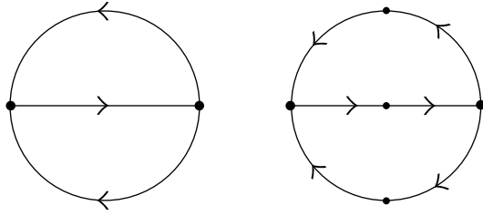
Figure 5.1 The effect of a field extension with e_{L/K} = 2 .
