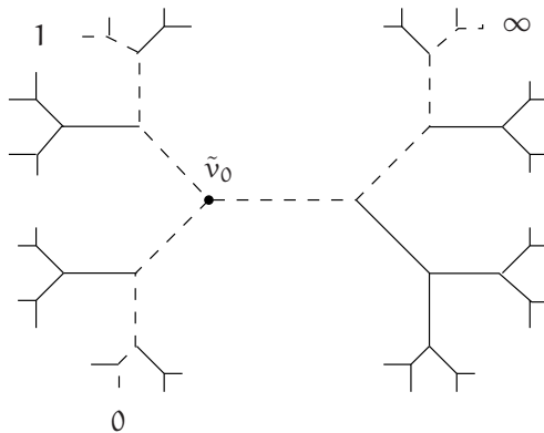
Figure 3.3 The crossroad \tilde{v}_0 of the points \{0, 1, \infty\} .
