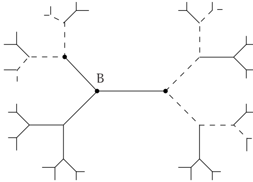
Figure 3.1 Two axes and the bridge B between them.
