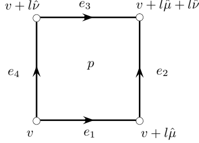
FIGURE 12. A plaquette in the lattice; the vectors \hat{\mu} and \hat{\nu} correspond to the edges along the plaquette p .
