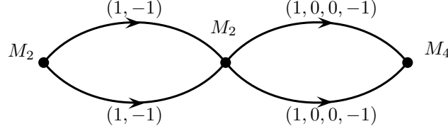
FIGURE 11. A gauge network for the algebra maps M_2(\mathbb{C}) \rightarrow M_2(\mathbb{C}) \rightarrow M_4(\mathbb{C}) .
