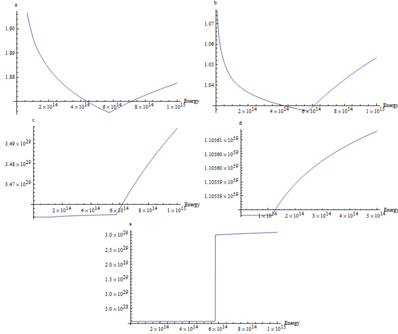
Figure 1. The running coefficients with default boundary conditions near top see-saw scale
