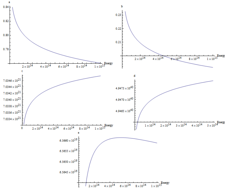
Figure 2. The running coefficients with maximal mixing boundary conditions near top see-saw scale
