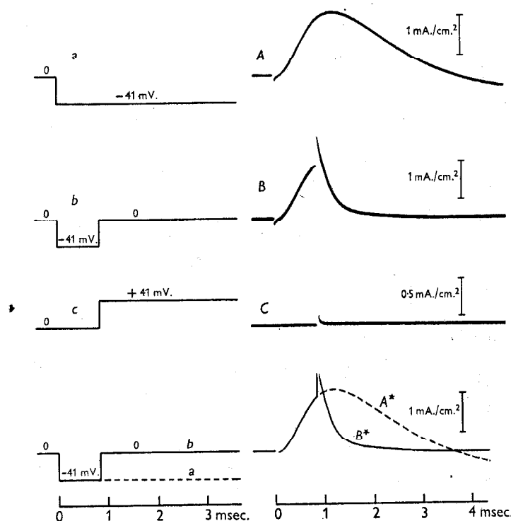
Fig. 1. Left-hand column: a , b , c , time course of potential difference between external and internal electrode. Right-hand column: A , B , C , records of membrane current associated with changes in membrane potential shown in left-hand column. (The amplification in C was 90% greater than that in A and B .) A* , B* , time course of ionic currents obtained by subtracting capacity current in C from A and B . Axon 25; temperature 5^\circ \text{C} .; uncompensated feed-back. Inward current is shown upward in this and all other figures except Fig. 13.
