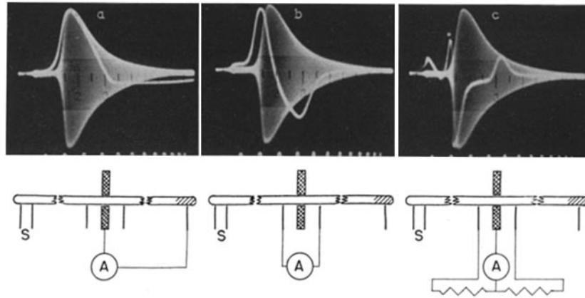
FIG. 9. Double exposures of the impedance change at 10 kc. on each with the action potential in each picture from the circuit shown below it. (a) is V , the monophasic potential, (b) is V_t , the first derivative or axial current, and (c) is V_{tt} , the second derivative or membrane current. The time marks at the bottom are 1 millisecond apart.
