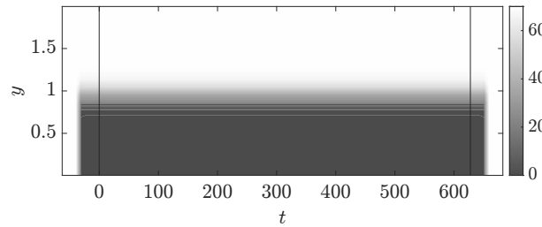
Figure 2: Temporal and spatial sponge enforcing decay near the extended-window boundaries and focusing the analysis on the near-wall region; vertical lines mark the physical interval where DNS data define the base flow. The sponge intensity increase toward white, while the non-sponge region is shown in gray. The total duration of the simulation is T = 620 with a temporal buffer region of T_{\text{buf}} = 63 . Sponge function parameters: \delta_y^{\text{off}} = -0.0045 , \delta_y^{\text{trans}} = 0.1 , \delta_{t,\text{up}}^{\text{off}} = -30 , \delta_{t,\text{down}}^{\text{off}} = 715.38 , and \delta_t^{\text{trans}} = 0.5 .
