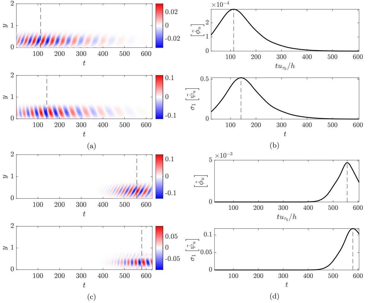
Figure 5: (a, c) Leading wavelet-based resolvent forcing and response modes \Re(\mathcal{W}^{-1}\widetilde{\phi}_{u_1}) (top) and \Re(\mathcal{W}^{-1}\widetilde{\psi}_{u_1}) (bottom) in the y - t plane at spatial scales (a) (\lambda_x, \lambda_z)_1 and (c) (\lambda_x, \lambda_z)_3 . (b, d) The y -integrated kinetic energy of the forcing (top) and response (bottom) mode at spatial scales (b) (\lambda_x, \lambda_z)_1 and (d) (\lambda_x, \lambda_z)_3 .
