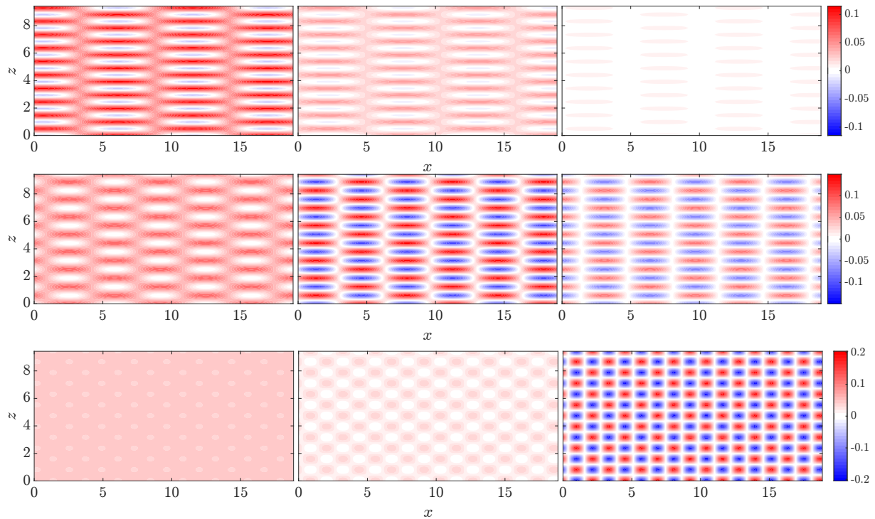
Figure 12: Instantaneous streamwise velocity from the model consisting only mean flow and the response modes at a single length scales, visualized on the (x, z) plane. Each row corresponds to a different length scale (\lambda_x, \lambda_z)_1 , (\lambda_x, \lambda_z)_2 , and (\lambda_x, \lambda_z)_3 , while the columns (from left to right) represent the temporal evolution at t_1 , t_2 , and t_3 , respectively, consistent with Figure 11.
