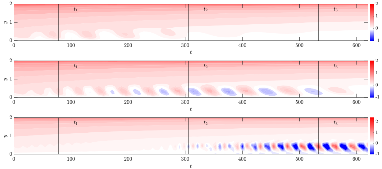
Figure 11: Instantaneous streamwise velocity from the model combining only mean flow and the response modes at a single length scales, visualized on the (y, t) plane. Each row corresponds to a representative wavelength pair (\lambda_x, \lambda_z)_1 , (\lambda_x, \lambda_z)_2 , and (\lambda_x, \lambda_z)_3 . Vertical lines denote three selected time instants t_1 , t_2 , and t_3 .
