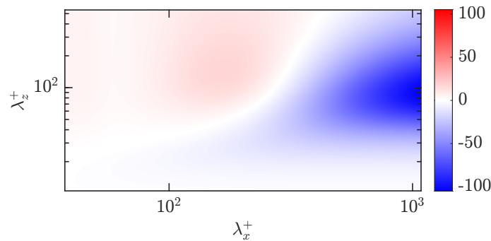
Figure 9: Distribution of the difference in the resolvent amplification \Delta\sigma_1 with time windowing at later times ( t_{\text{window}} = 550 ) and at earlier times ( t_{\text{window}} = 78.5 ), for different streamwise and spanwise wavelength combinations.
