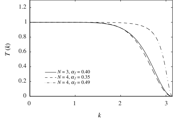
Fig. 1 Transfer function of commonly used explicit filters from Eq. (10).
