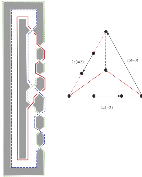
Fig. 6. The closure of the pure braid \sigma = \sigma_1 \sigma_2^{-2a-1} \sigma_1 \sigma_2^{-2b-1} \sigma_1 \sigma_2^{-2c-1} ( a = 1, b = 0, c = 1 here) and its black graph on the right. The graph is supported in a triangle P with 2a , 2b and 2c interior dots on each side, and there is an edge connecting the center of P with each corner vertex of P . The maximal tree T is obtained by removing an edge from each side of P .
