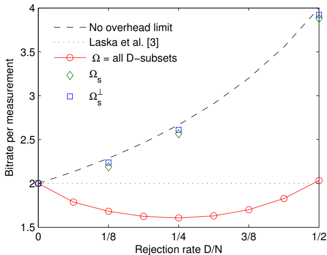
Fig. 2: Bitrate per surviving measurement versus D/N for the total bit budget B = 2N bits. DGF(7, 0) .
