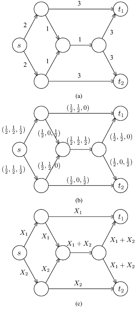
Fig. 1. A network with multicast from s to T = \{t_1, t_2\} . (a) Each arc is marked with its cost per unit rate. (b) Each arc is marked with the triple (z_{ij}, x_{ij}^{(1)}, x_{ij}^{(2)}) . (c) Each arc is marked with its code.
