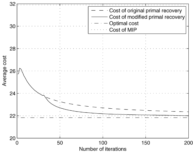
Fig. 2. Average energy of a random four-terminal multicast of unit rate in a 30-node wireless network using the subgradient method of Section II-B. Nodes were placed randomly within a 10 \times 10 square with a radius of connectivity of 3. The energy required to transmit at rate z to a distance d was taken to be d^2 z . Source and sink nodes were selected according to a uniform distribution over all possible selections.
