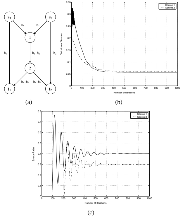
Fig. 1. (a) The butterfly network; (b) The evolution of source distortions versus the number of iterations; (c) The evolution of source rates versus the number of iterations.
