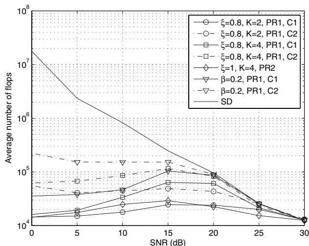
Fig. 2. Complexity comparison of SD with different statistical pruning rules for an 8 \times 8 MIMO system with 16QAM.
