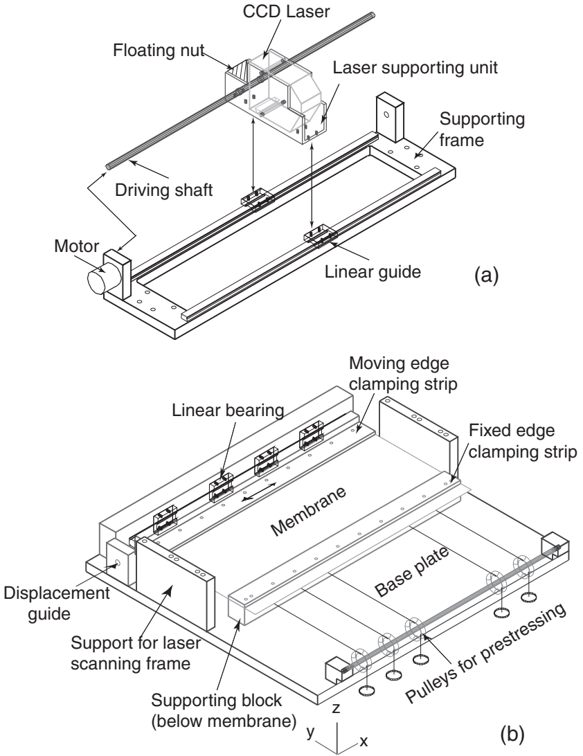
Figure 1. (a) Laser scanning frame, (b) Shear-rig.
