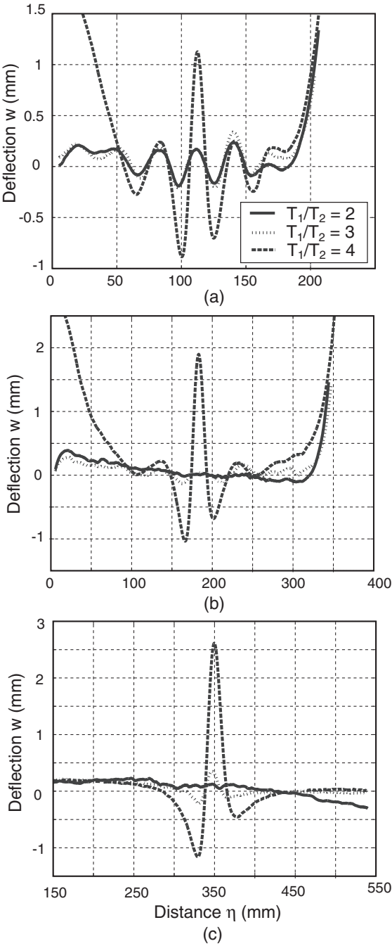
Figure 11. Wrinkle profiles for 0.025 mm thick, square Kapton ® membrane at (a) \xi = 105 , (b) \xi = 177 and (c) \xi = 355 mm for different load ratios.
