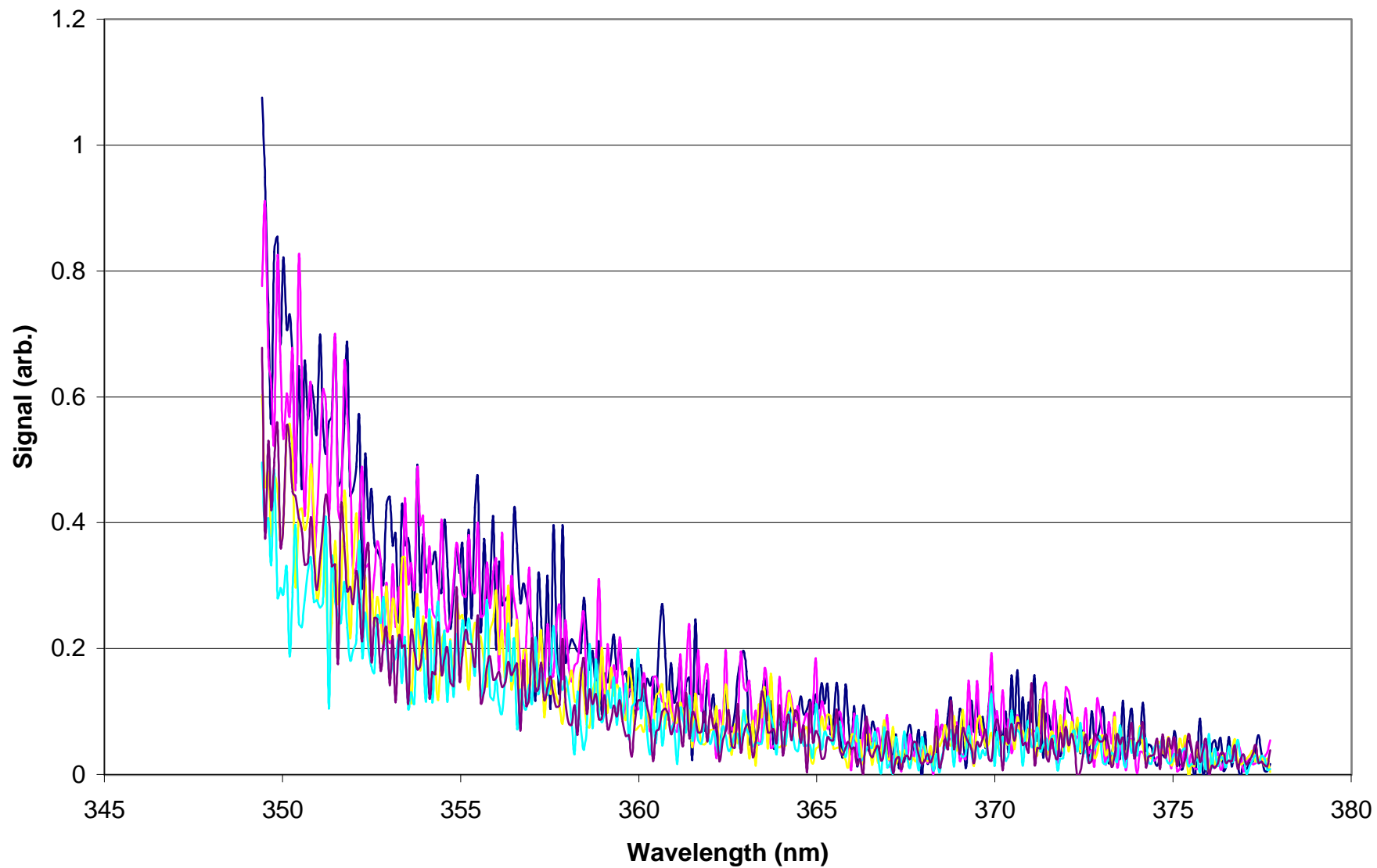
PIE Spectra of K(H_2O)_n , n=7,8,9,10,11
