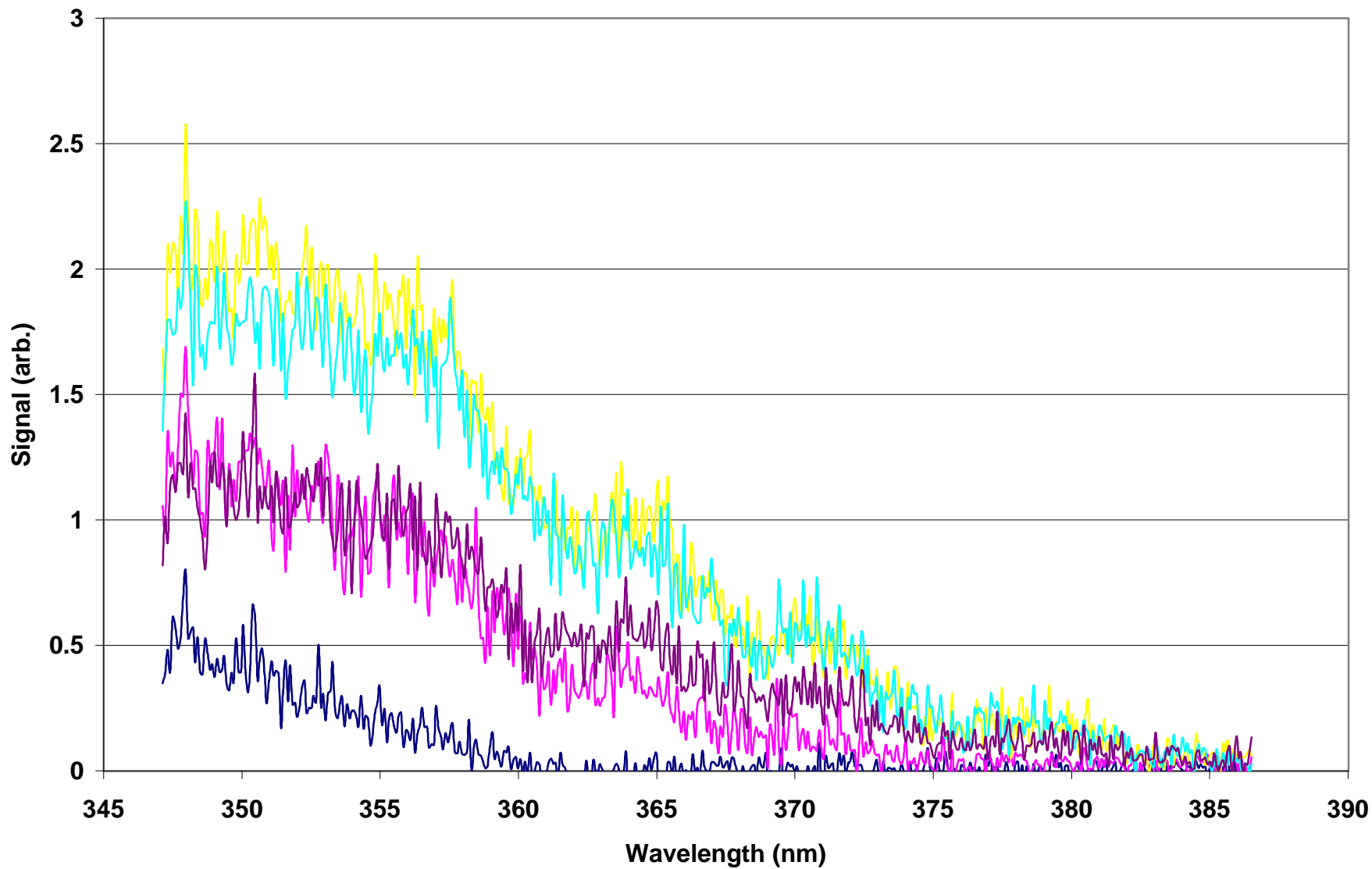
PIE spectra of K(H_2O)_n , n=2,3,4,5,6
