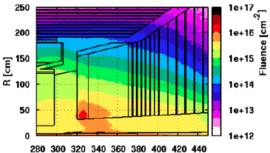
neutral hadrons, Shashlik LYSO, 3000fb -1
