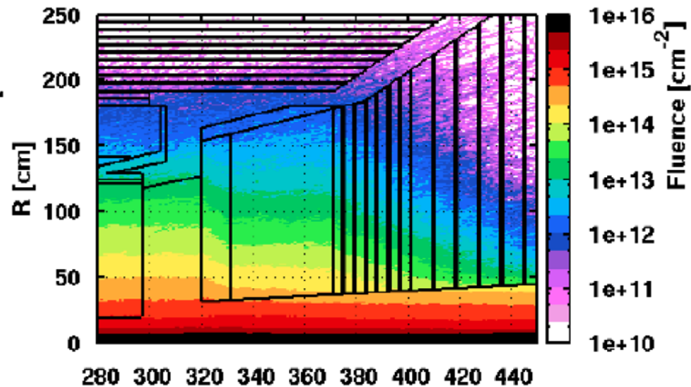
charged hadrons, Shashlik LYSO, 3000fb -1
