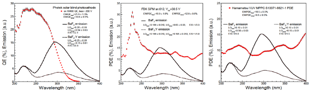
Figure 6. The QE of a Photek solar-blind cathode (Left), the PDE of a FBK solar-blind SiPM (Middle) and the PDE of a Hamamatsu VUV SiPM (Right) are shown as a function of wavelength.
