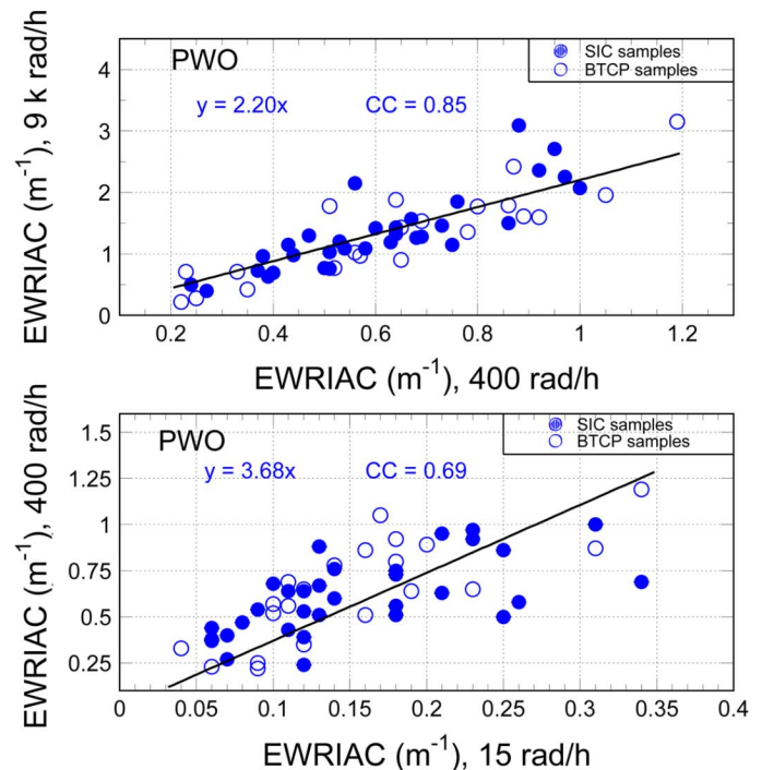
Fig. 13. Correlations between the EWRIAC values measured for all BTCP and SIC samples in the equilibrium under irradiations of different dose rates.
