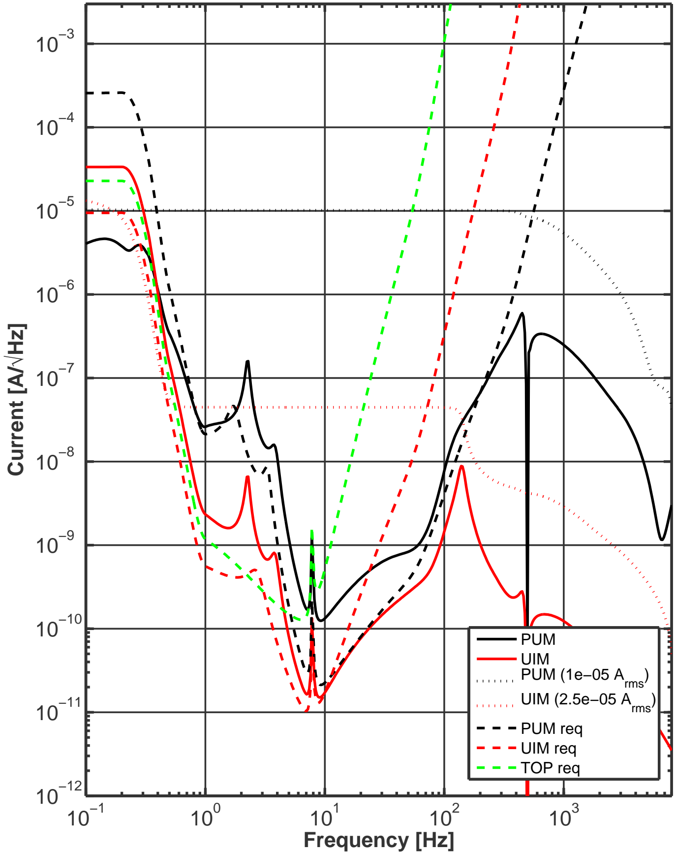
Current Noise Spectra for the LSC (SRD state)
