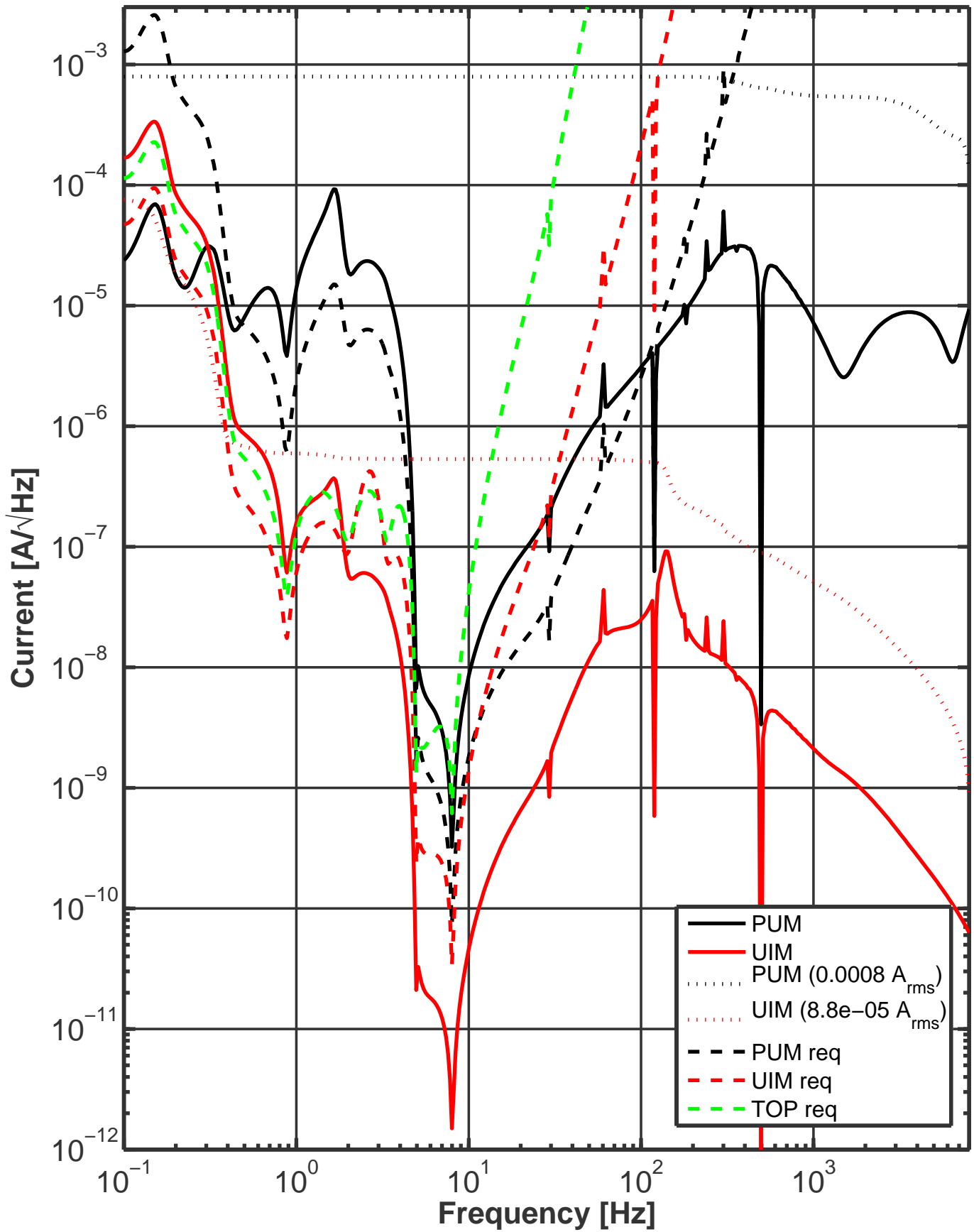
Current Noise Spectra for the LSC (NOISY state)
