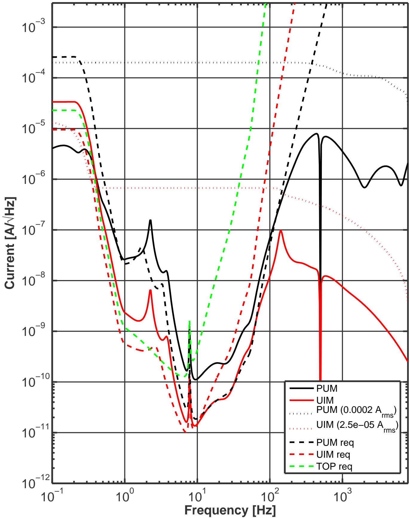
Current Noise Spectra for the LSC (LOW state)
