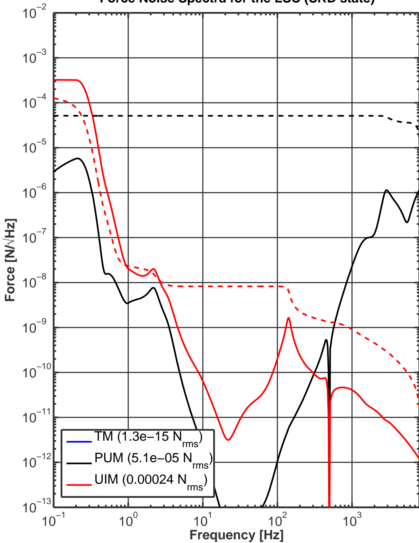
Force Noise Spectra for the LSC (SRD state)
