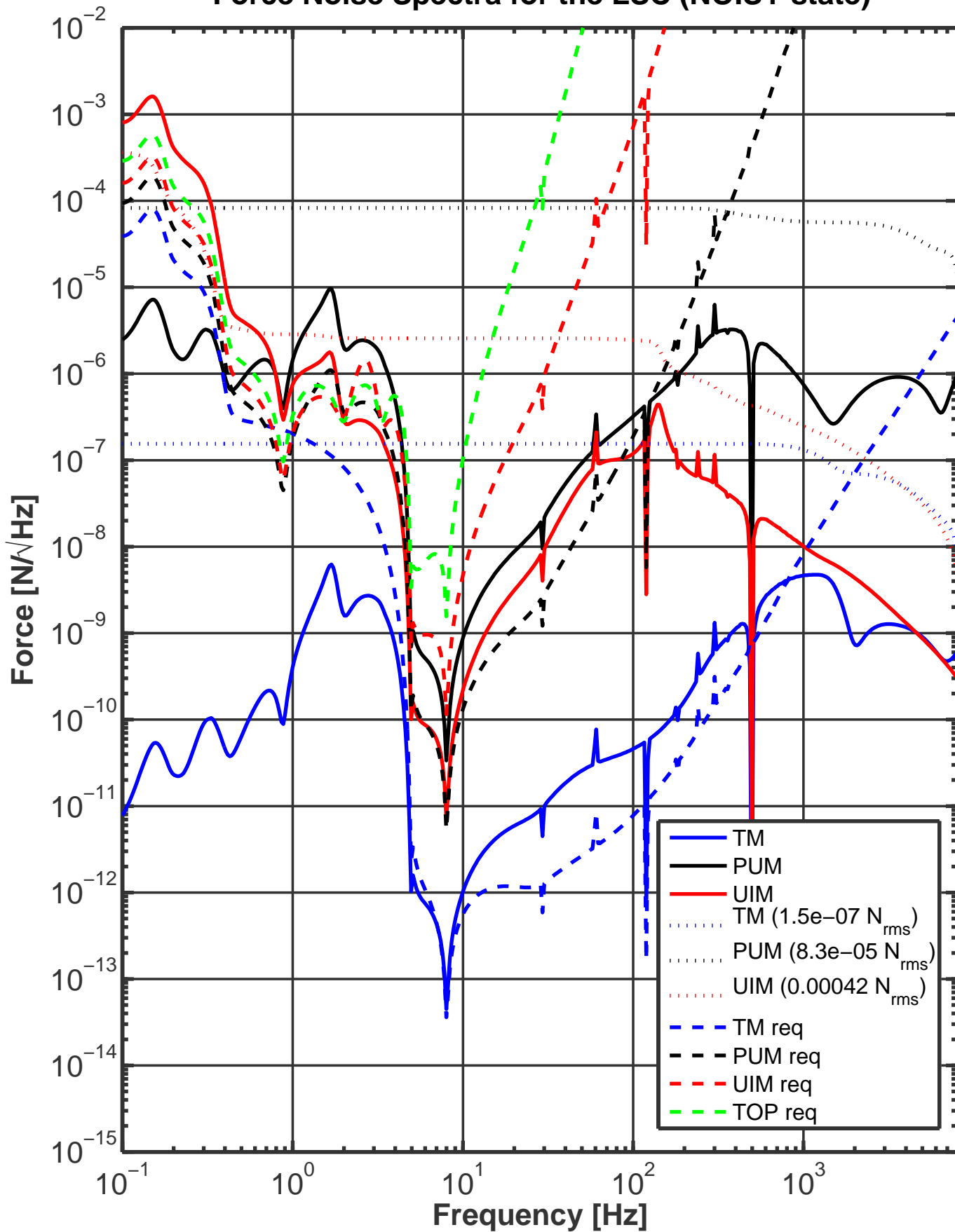
Force Noise Spectra for the LSC (NOISY state)
