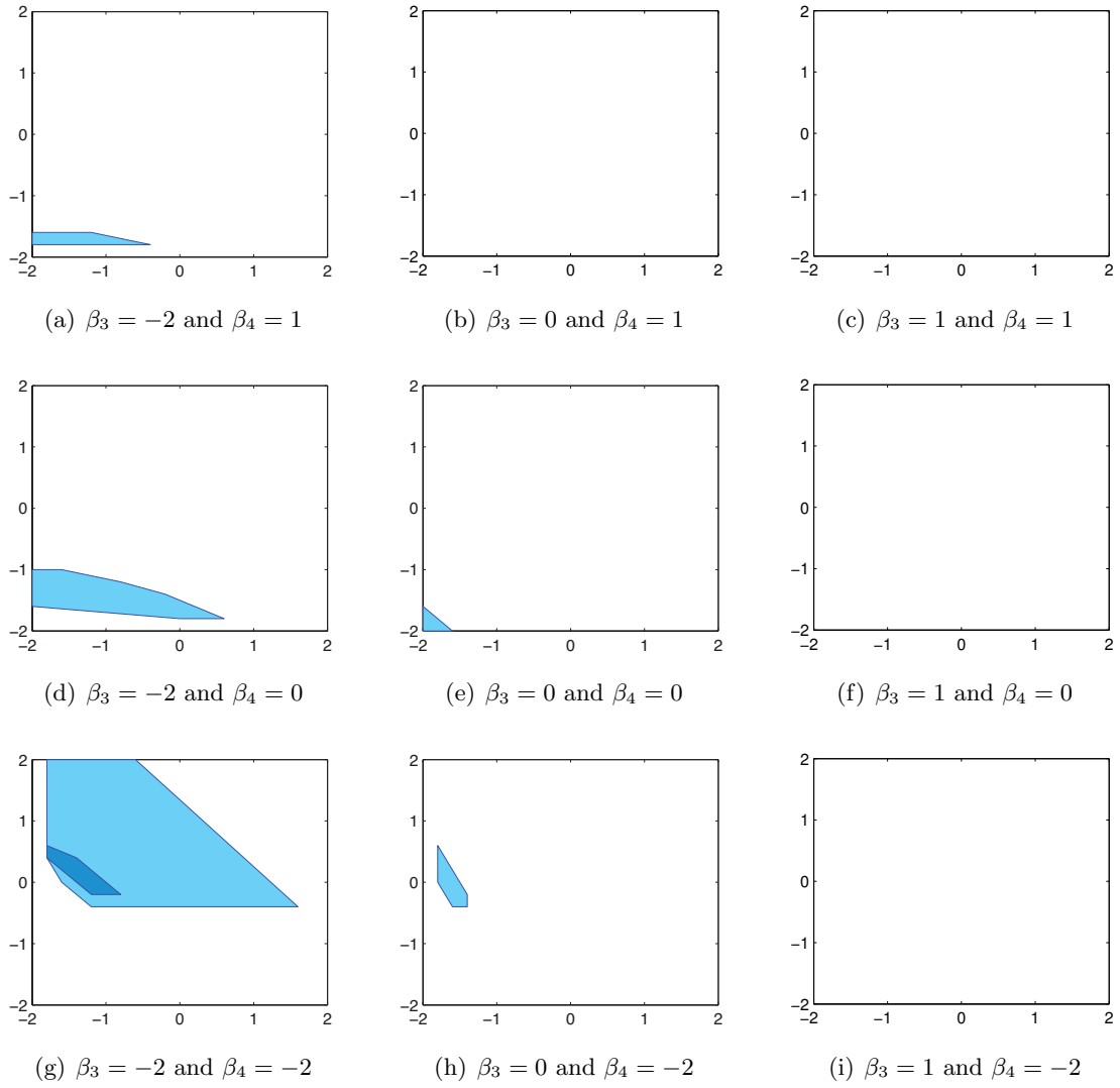
Figure 2: 95% confidence sets of (\beta_1, \beta_2) given (\beta_3, \beta_4) and \gamma = 32 (shaded lightly) and 35 (shaded darkly).
