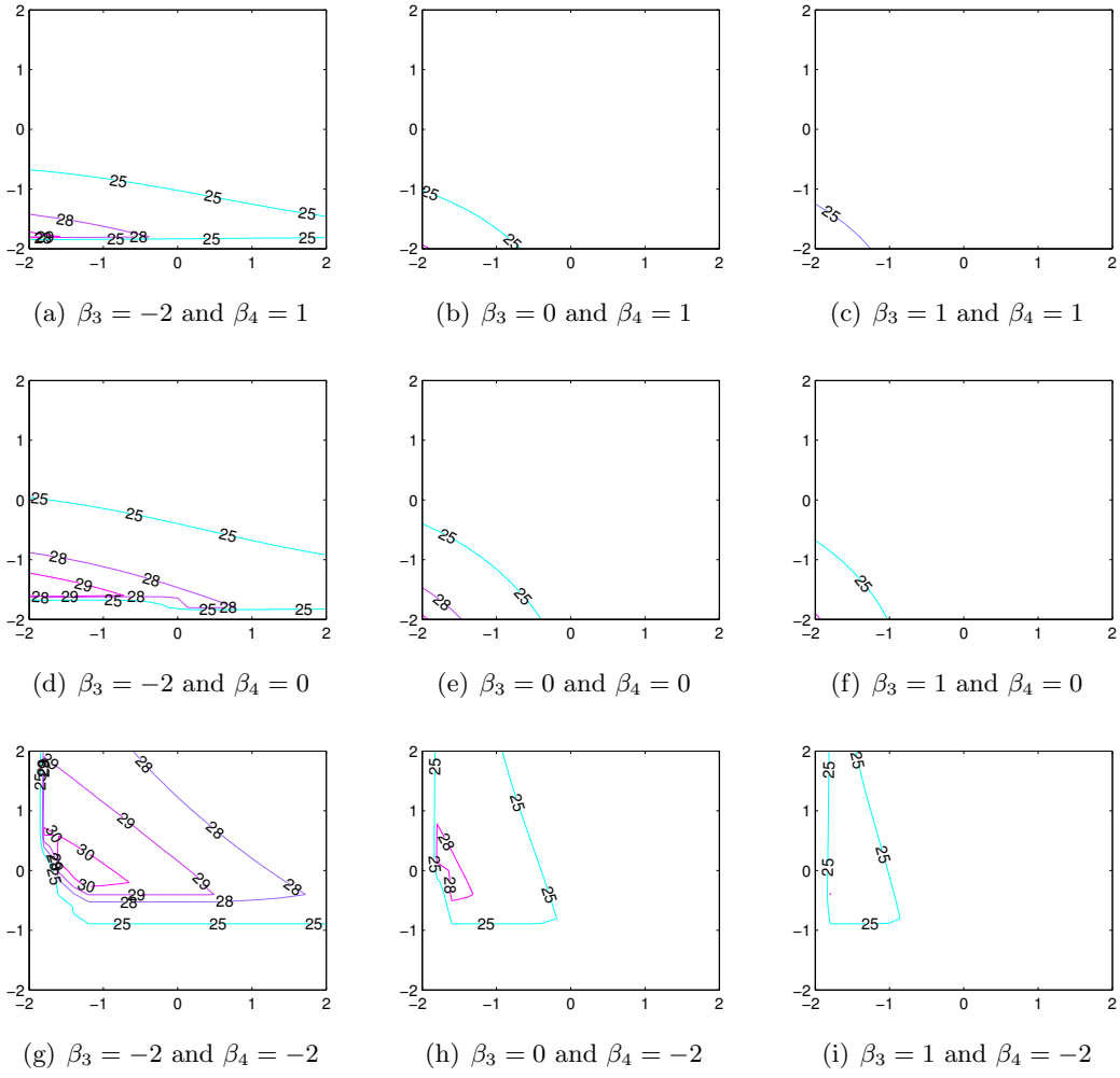
Figure 1: Identified sets of (\beta_1, \beta_2) given (\beta_3, \beta_4) and \gamma .
