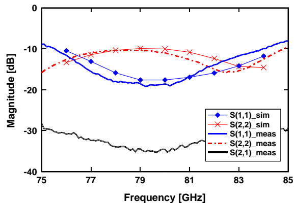
Fig. 3. Measured ( S_{meas} ) and HFSS-simulated ( S_{sim} ) S-parameters of the OMT in conjunction with mode converter over 75 to 85 GHz.
