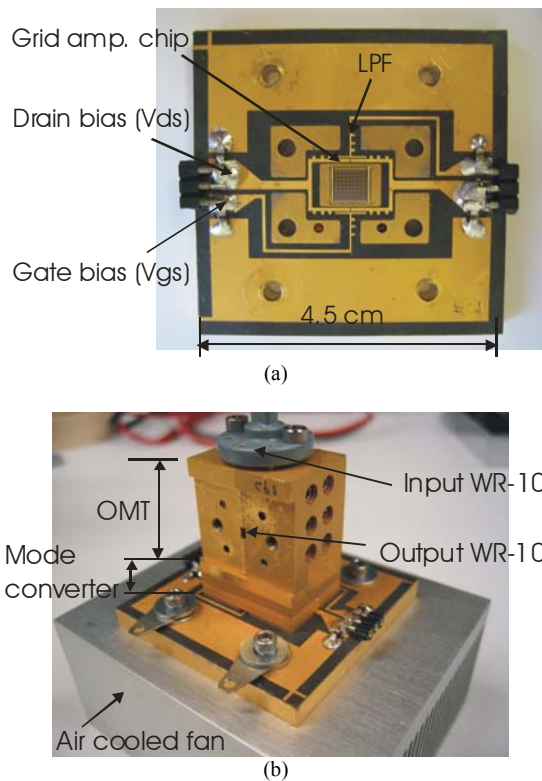
Fig. 4. Photographs of (a) mounted grid chip (b) assembled grid amplifier
