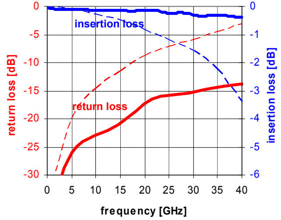
Fig. 7. S-Parameters for a single transition, corrected for multiple reflections and the loss of the microstrip line. For comparison, the dashed lines show simulated results for a perpendicular transition without the ground aperture compensation described in this paper.
