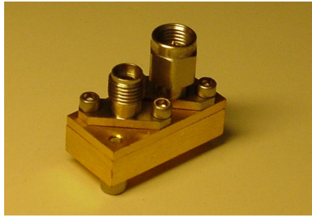
Fig. 4. Photograph of the back-to-back transition test block.
