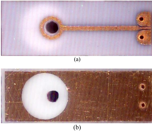
Fig. 2. Top (a) and bottom (b) views of the transition adapter. The hole in the center of the 100 \mu\text{m} -thick Alumina substrate fits over the center pin of a standard K-connector coaxial glass bead. The substrate dimensions are 3.75 x 1.35 mm.
