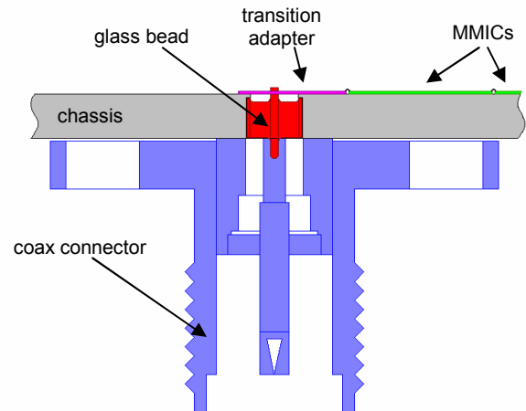
Fig. 1. Assembly diagram of the perpendicular coax-microstrip transition. A K flange launcher is shown, but threaded "sparkplug" launchers can be used as well.
