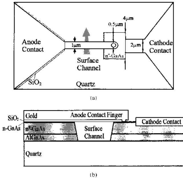
Fig. 2. Schottky-diode layout. (a) Top view. (b) Cross section. The n-GaAs layer is 0.1\text{-}\mu\text{m} thick and has a doping concentration of 4 \times 10^{17}\text{ cm}^{-3} . The n^+\text{-GaAs} layer has a thickness of 3\text{ }\mu\text{m} and a doping of 5 \times 10^{18}\text{ cm}^{-3} . The AlGaAs layer has a thickness of 1.5\text{ }\mu\text{m} .
