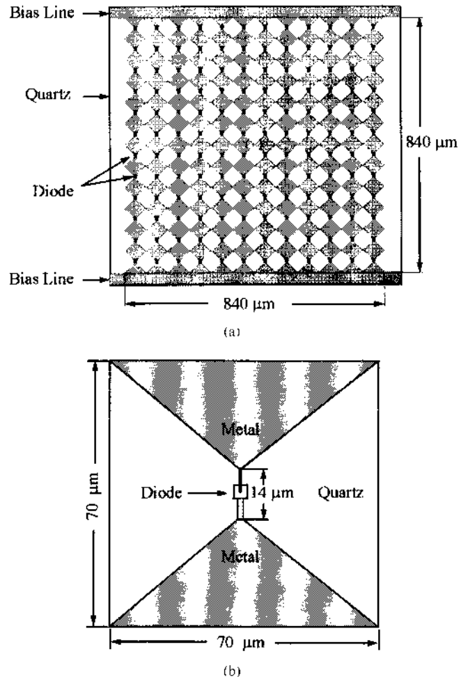
Fig. 3. The multiplier grid. (a) Entire 12 \times 12 array. The diodes are in series from top to bottom. The grid can be biased through the bias lines at the top and bottom of the grid. The metal contacts in a row are all electrically connected. (b) Unit cell. The diode is located at the center of the cell.
