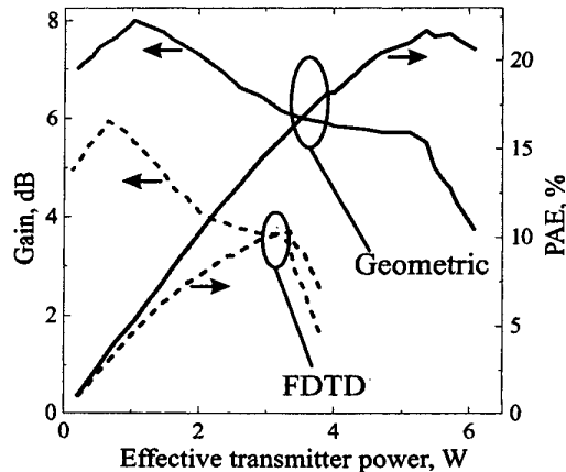
Fig. 5. Measured gain and power-added efficiency (PAE) versus output effective transmitter power (ETP) at 34.4GHz. Solid lines are normalized by the geometric area and dotted lines are normalized by the effective area predicted by finite-difference time-domain simulation.
