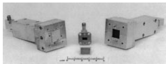
Fig. 5. (a) Quasi-optical amplifier in a waveguide fixture. Smaller arrays could be put into a single-mode waveguide; larger arrays must be put into an oversized structure, possibly with sidewall loading to insure a flat field. (b) Rockwell array amplifier in a tapered waveguide fixture [35].
