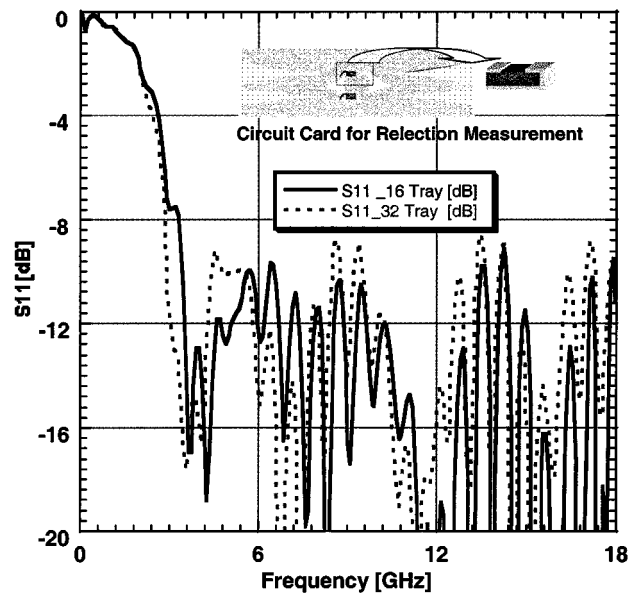
Fig. 7. Return loss measurement for 16- and 32-tray combiner with 50-Ω terminations on the finline structures. Inset shows circuit configuration.
