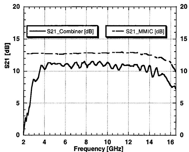
Fig. 12. Measured small-signal gain of the active combiner and individual MMIC amplifier.
