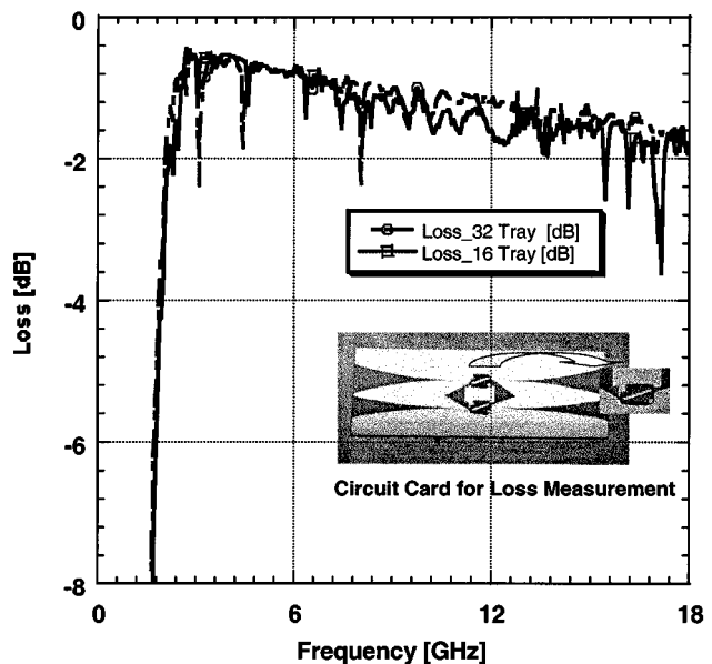
Fig. 8. Dissipative loss for 16- and 32-tray combiners with 50-Ω microstrip through line in place of the active device. Inset shows circuit configuration.
