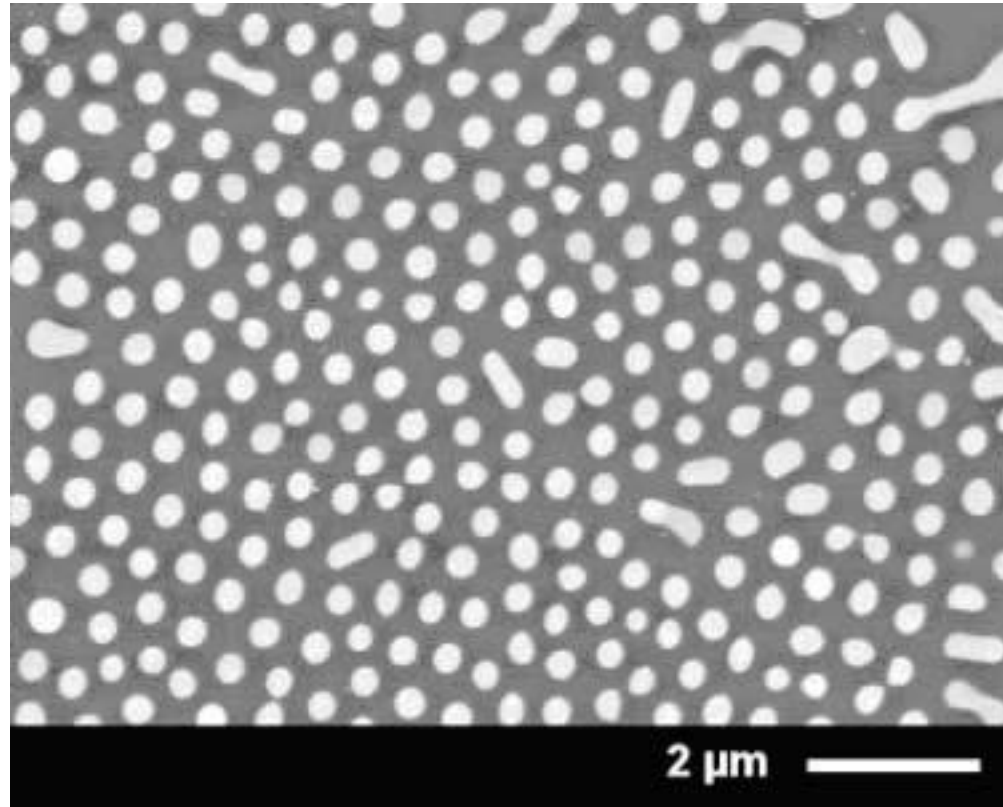
Nb precipitates in Nb 3 Si, ONERA
