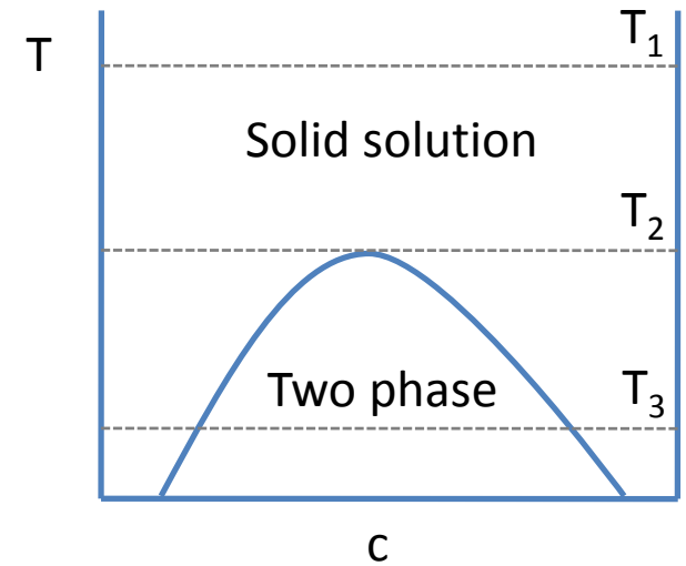
Phase diagram
