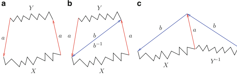
Fig. 1.19 Grouping the cross-caps
