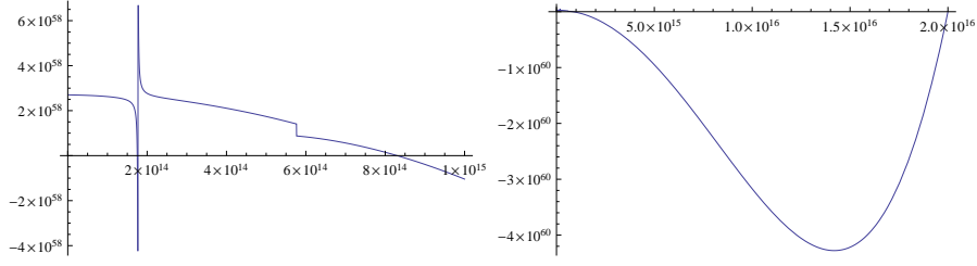
FIGURE 13. Running of \gamma_{0,H}(\Lambda) with f_2 = 1 and with \gamma_0(\Lambda_{unif}) = 0 .
