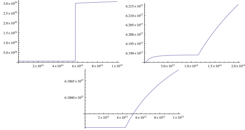
FIGURE 4. The coefficient \epsilon as a function of the energy scale \Lambda near the three see-saw scales.
