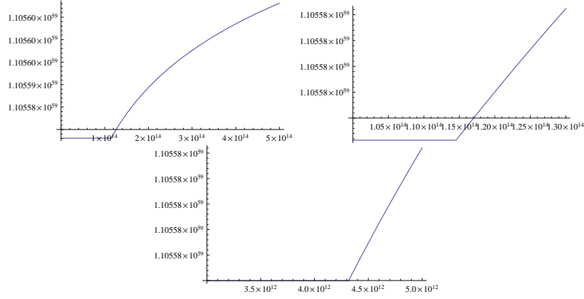
FIGURE 3. The coefficient \mathfrak{d} as a function of the energy scale \Lambda near the three see-saw scales.
