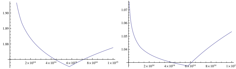
FIGURE 1. Coefficients \mathbf{a} and \mathbf{b} as functions of the energy scale \Lambda near the top see-saw scale.
