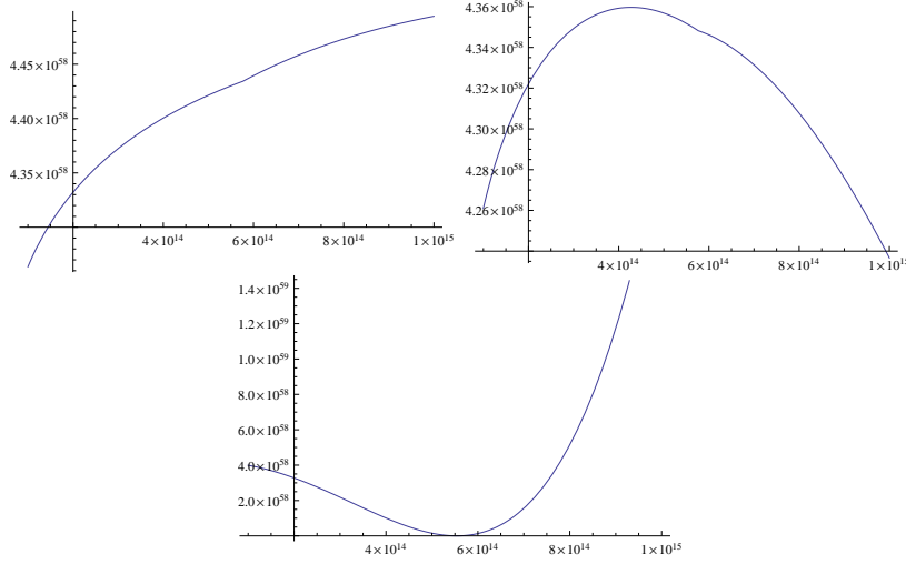
FIGURE 11. The behavior of the asymptotic value V_E of the potential V_E(H) , plotted above for f_2 = 10^{-4} , f_2 = 10^{-3} , and f_2 = 1/10 and for 10^{14} \leq \Lambda \leq 10^{15}
