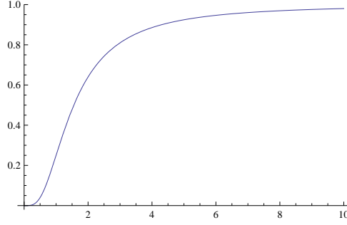
FIGURE 10. Plot of V_E(H)/V_E against \psi .
