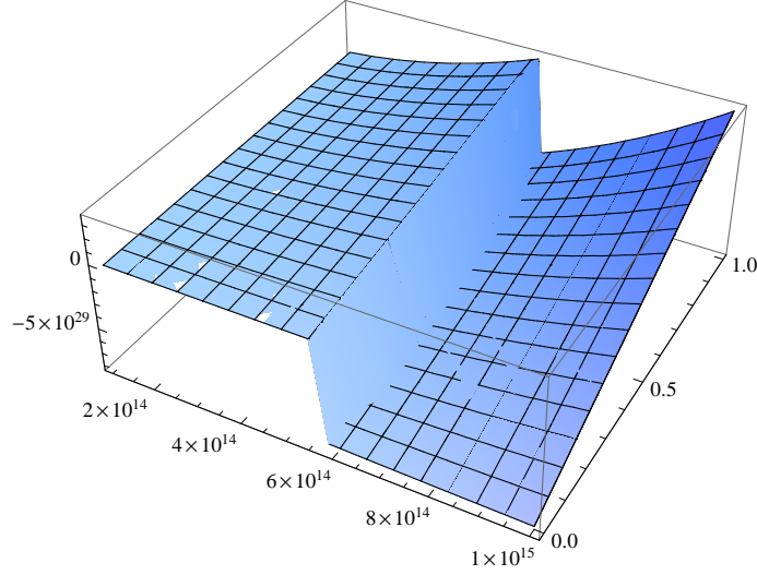
FIGURE 8. The surface \ell_H(\Lambda, f_2) in the range 10^{14} \leq \Lambda \leq 10^{15} GeV, around the top see-saw scale, for 10^{-4} \leq f_2 \leq 1 .
