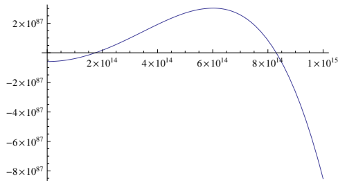
FIGURE 14. Running of \gamma_0(\Lambda)/(8\pi G_{\text{eff}}(\Lambda)) with f_2 = 1 and with \gamma_0(\Lambda_{\text{unif}}) = 0 .
