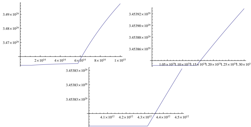
FIGURE 2. The coefficient \mathbf{c} as a function of the energy scale \Lambda near the three see-saw scales.
