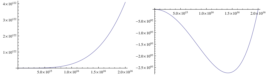
FIGURE 12. Running of \gamma_0(\Lambda) under the assumptions of vanishing \gamma_0(\Lambda_{ew}) = 0 or \gamma_0(\Lambda_{unif}) = 0 .
