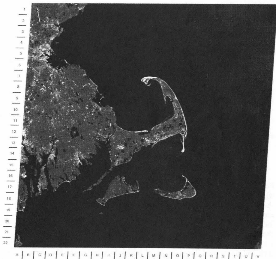
Figure 4. A sandy shore often has cusplike spits.
