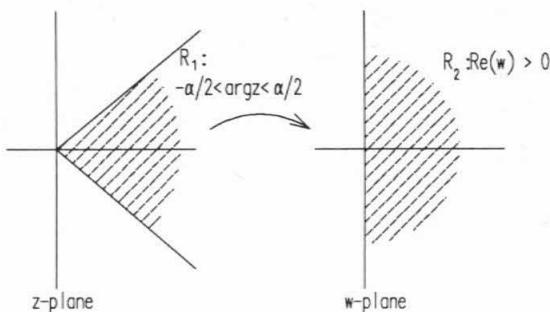
Figure 9. Straightening of a corner by a conformal map.
