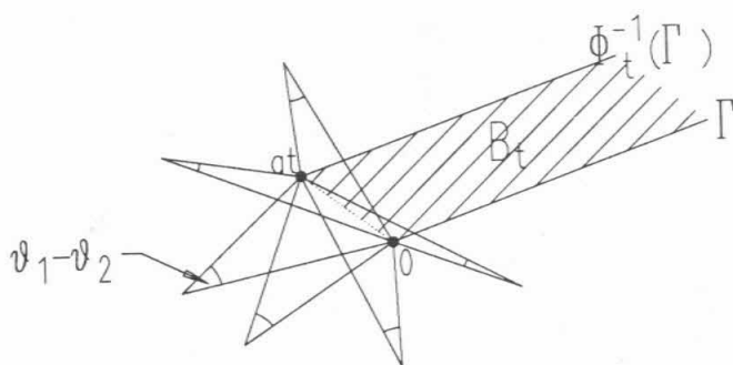
Figure 17. The function \theta_1 - \theta_2 .
