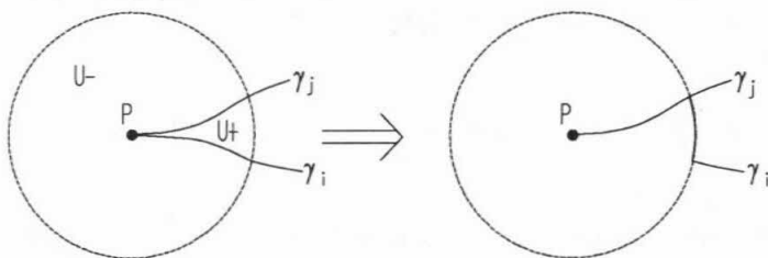
Figure 15. Eliminating cuspidal corners in \Gamma .
