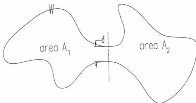
Figure 5. Definition of the isoperimetric constant.
