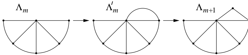
FIGURE 7. Lemon building from edge doubling.
