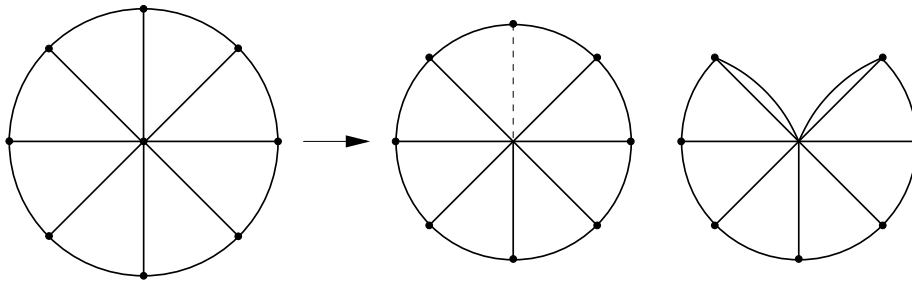
FIGURE 6. Deletion-contraction on the wheel W_8 .
