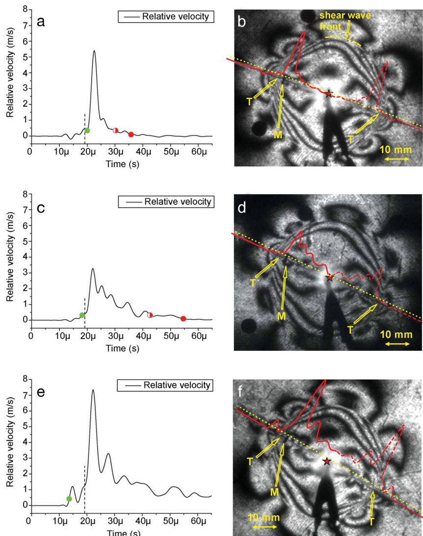
Fig. 2. Three representative rupture modes corresponding to different inclination angles. (a and b) A narrow sub-Rayleigh pulse for \alpha = 20^\circ . (c and d) A wider (e and f) A sub-Rayleigh crack-like rupture for \alpha = 30^\circ . Compression load P is 10 MPa for all three cases. (Left) Relative velocity histories recorded at 20 mm distance from the hypocenter. The dashed lines indicate the time of the shear wave arrival. The green fully filled dots indicate the estimated initiation time of interface sliding. The red half-filled and fully filled dots indicate two estimates of interface locking time. Note that there are no estimates of locking time marked in panel e because the interface in that case experiences no locking at the measurement location within the window of observation. (Right) Contours of maximum shear stress captured at 22 \mu\text{s} after rupture initiation. Letters T indicate rupture tips. Letters M indicates the measurement location for the two velocimeters. The relative velocity record is superimposed on the photoelastic pattern to facilitate the analysis of rupture behavior. The yellow dotted lines indicate the value of the elastic cut-off velocity for each case.
