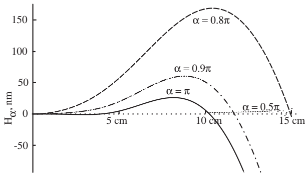
FIG. 2: The correction H_\alpha(r) to the mirror shape for hyperboloidal beams with D = 10 cm and with twist angles \alpha between \pi/2 and \pi . For \alpha = 0 , the correction is the negative of that for \alpha = \pi ; for \alpha = 0.1\pi it is the negative of that for 0.9\pi ; for any \alpha between 0 and \pi/2 , it is the negative of that for \pi - \alpha . For \alpha = \pi (the Mexican-hat correction for our new CM mesa beam), H_0(r) drops to about -500 nm (half the wavelength of the light beam) at r = 16 cm (the mirror's edge). These corrections are added onto the fiducial spheroidal shape S_\alpha(r) [Eq. (13)].
