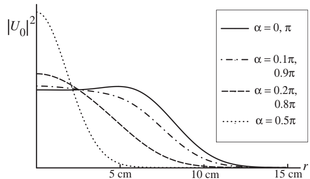
FIG. 3: The light beam's un-normalized intensity |U_\alpha|^2 as a function of radius r on the mirror, for hyperboloidal beams with D = 10 cm and various twist angles \alpha . For \alpha = 0 and \pi , the intensity has the mesa shape; for \alpha = 0.5 it is a minimal Gaussian.
