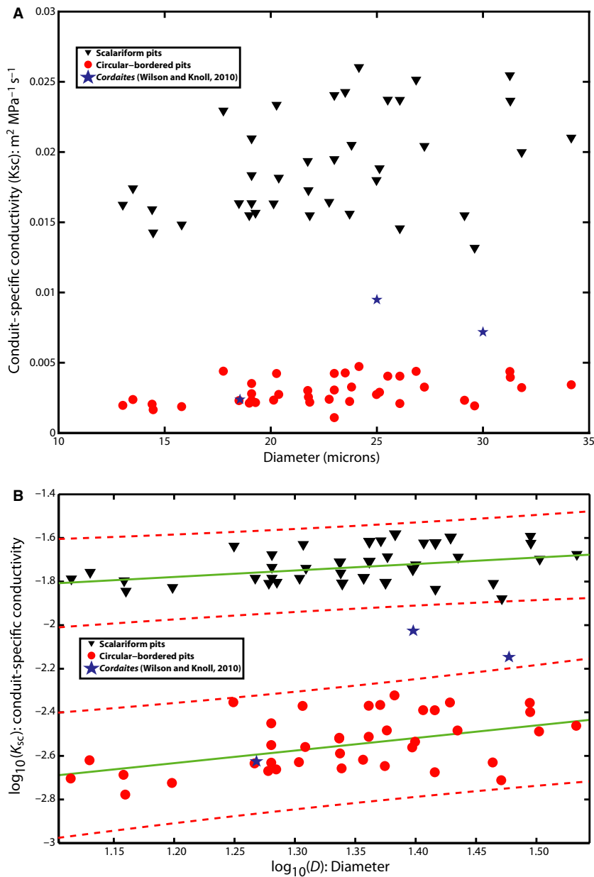
Fig. 3 Conductivity of Asteroxylon mackei tracheids as a function of diameter: scalariform pits increase conductivity over circular-bordered pits. (A) Conduit-specific conductivity (conductivity normalized to cross-sectional wall area; \text{m}^2 \text{MPa}^{-1} \text{s}^{-1} ) vs. diameter ( \mu\text{m} ). (B) Log-transformed conduit-specific conductivity vs. diameter. Green lines show least-squares linear regressions through datasets, red lines are 95% confidence intervals on regressions. Equation for circular-bordered pit data: \log_{10}(K_{sc}) = 0.5768 * \log_{10}(D) - 3.3288 . Equation for scalariform pit data: \log_{10}(K_{sc}) = 0.2972 * \log_{10}(D) - 2.1357 . Blue stars are modeled conductivities through tracheids of an extinct conifer, Cordaites (Wilson & Knoll, 2010). Black triangles are A. mackei tracheids with scalariform pits, red dots are tracheids with circular-bordered pits with approximately the same pitted area.
