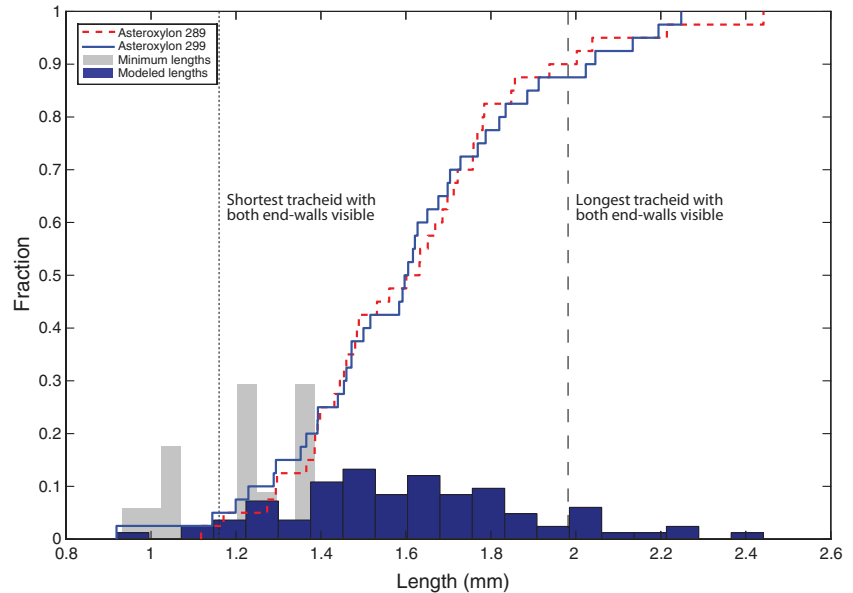
Fig. 2 Statistical distribution of tracheid lengths in Asteroxylon mackei . Lines are cumulative distribution functions of modeled lengths for two specimens. Dark histogram is distribution of modeled values. Because thin sections rarely preserve both ends of a single tracheid, we measured minimum lengths of 43 tracheids that only had a single wall preserved (gray histogram). These tracheids cannot be any smaller than the amount we measured, and fall comfortably within the distribution of modeled lengths.
