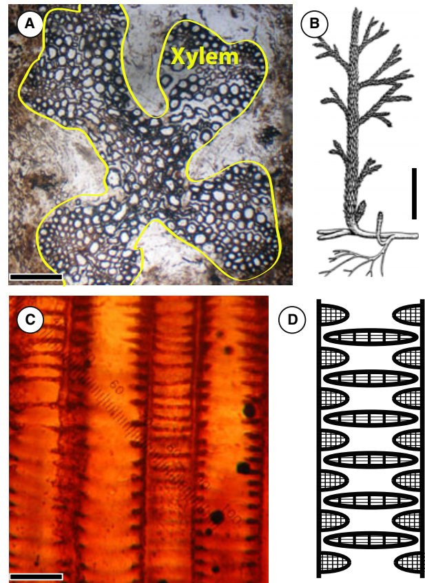
Fig. 1 Morphology and anatomy of Asteroxylon mackei , an Early Devonian vascular plant. (A) Cross-section of permineralized A. mackei stem, vascular tissue outlined in yellow (Harvard University Paleobotanical Collection #29288). Scale bar is 200 \mu\text{m} . Specimen is from the Rhynie Chert deposit. (B) Reconstruction of A. mackei , based on permineralized material from the Rhynie Chert, from Kidston & Lang (1920); note the small leaves (microphylls). Scale bar is 10 cm. (C) Longitudinal section through A. mackei vascular tissue, showing several xylem cells next to each other. Scale bar is 25 \mu\text{m} . (D) Schematic showing scalariform-type pitting used to quantify conductivity through A. mackei tracheids. Elliptically shaped porous areas (ovals with internal crossed lines) are spirally arranged to represent pitted area within tracheids.
