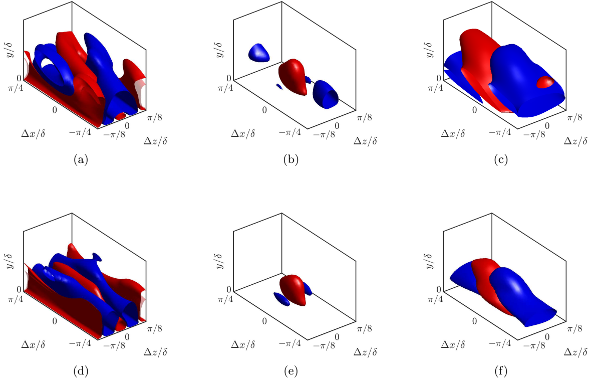
Figure 8: Correlations (a,d) C_{uu} , (b,e) C_{vv} , and (c,f) C_{ww} conditioned to (a,b,c) high forcing-intensity and (d,e,f) low forcing-intensity events for Re_\tau \approx 186 . The isosurfaces are 0.1 (red) and -0.04 (blue).
