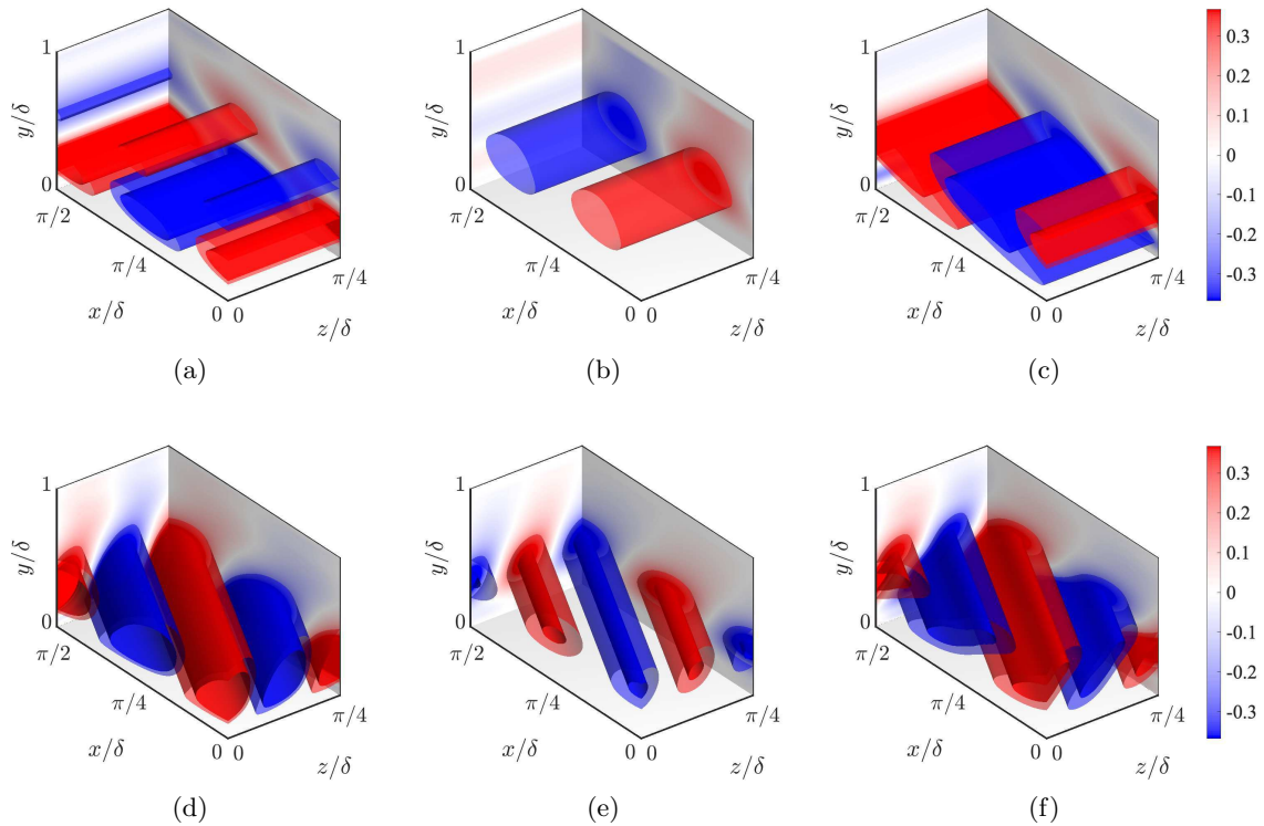
Figure 7: Average (a) \mathcal{F}^{-1}\hat{u} , (b) \mathcal{F}^{-1}\hat{v} , (c) \mathcal{F}^{-1}\hat{w} for (k'_x, k'_z) and (d) \mathcal{F}^{-1}\hat{u} , (e) \mathcal{F}^{-1}\hat{v} , (f) \mathcal{F}^{-1}\hat{w} for (k_x - k'_x, k_z - k'_z) conditioned to high forcing-intensity events shown in physical coordinates for Re_\tau \approx 186 . The surface plots are in wall units with values indicated by the colorbar. The isosurfaces are values corresponding to 0.41 (solid red), 0.26 (transparent red), -0.26 (transparent blue), and -0.41 (solid blue).
