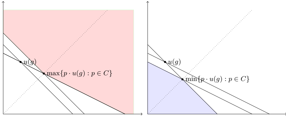
Figure 1: Upper and lower contour sets at an act g , with a binary state of the world, under a symmetric TFC preference. The axes describe the payoff u(g(\omega)) from the act in the two states.
