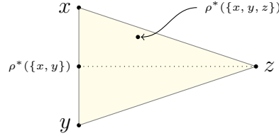
Figure 2: Path independence and Luce's IIA.
