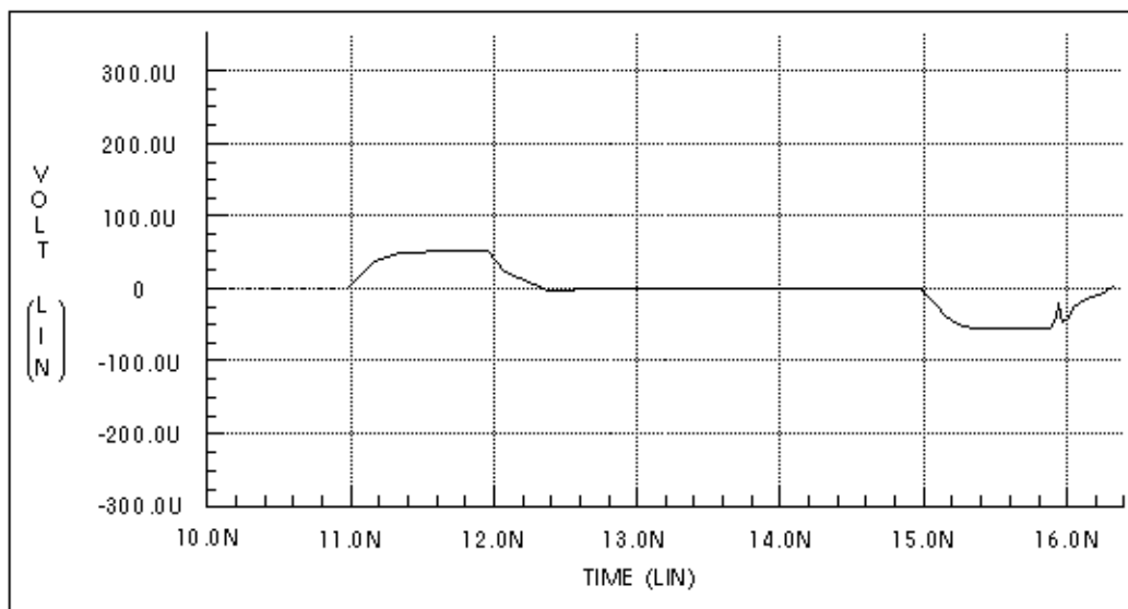
Figure B-33: Computed Furthest Coupled-Line Response
