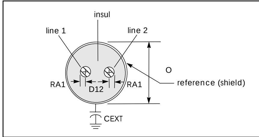
Figure B-18: Geometric Twinlead, DLEV=2, Shielded
