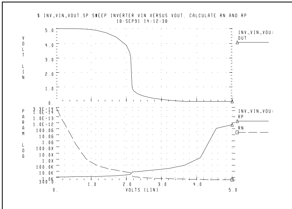
Figure 24-10: RP and RN as a Function of VIN
