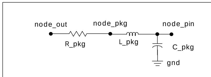
Figure 18-1: Circuit Diagram for Package
