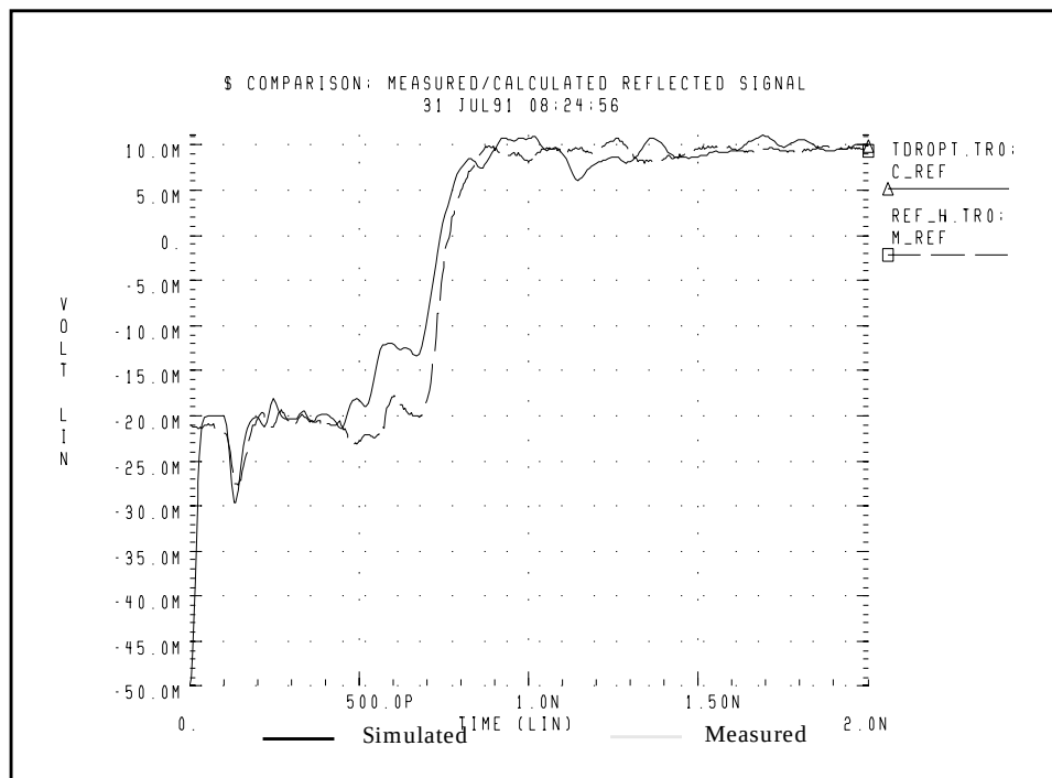
Figure 23-6: Reflected Signals Before Optimization
