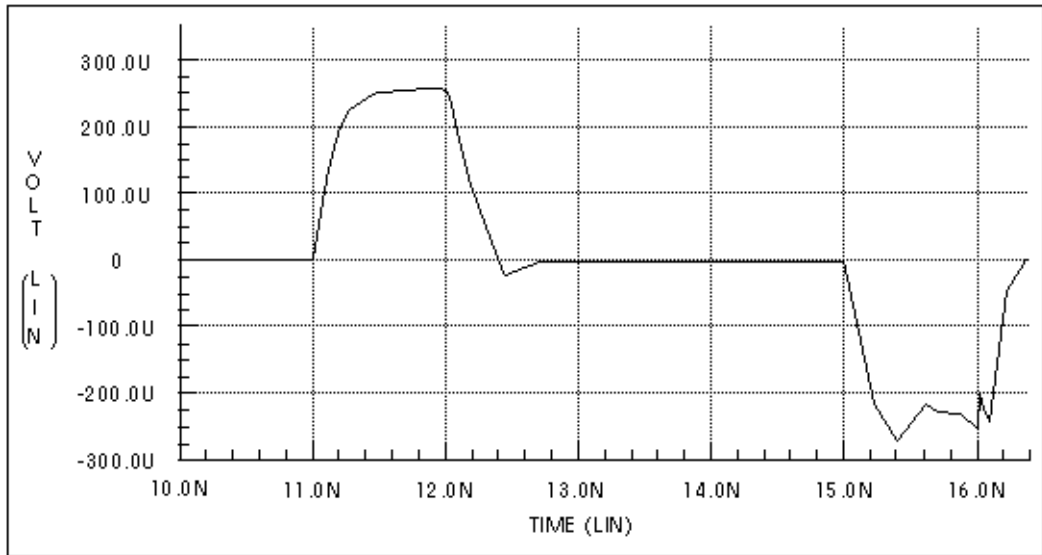
Figure B-32: Computed Nearest Coupled-Line Response
