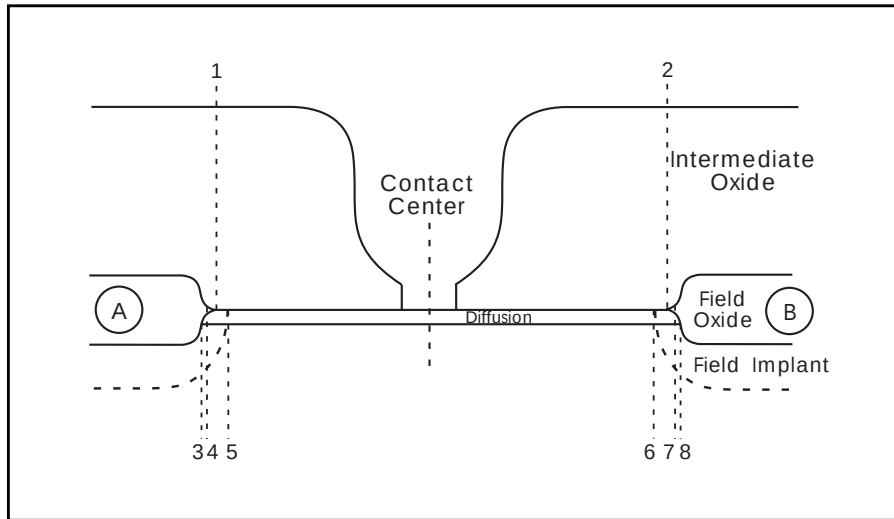
Figure 19-4: Isoplanar MOSFET Construction, Part A
