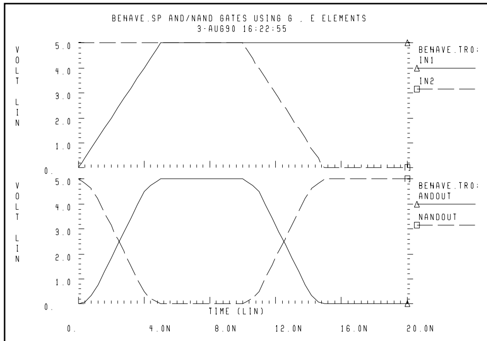
Figure 24-2: NAND/AND Gates
