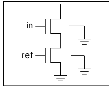
Figure 19-16: Low-frequency AC Analysis Measuring Output Impedance
