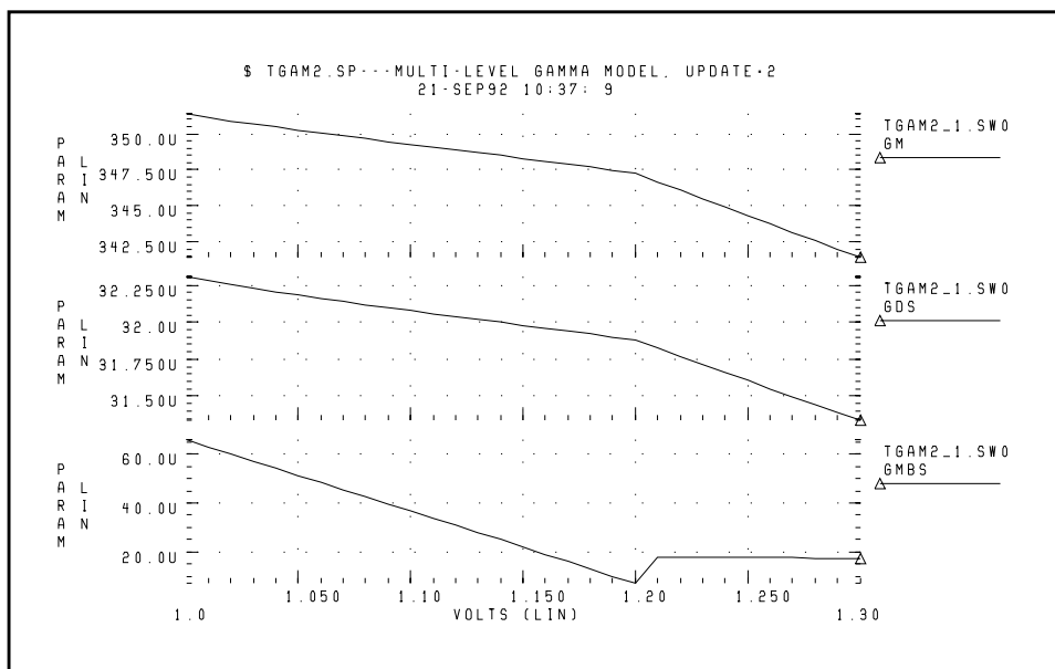
Figure 20-5: Variation of GM, GDS and GMBS for UPDATE=2
