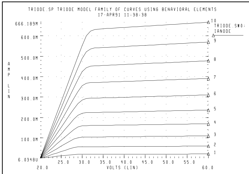
Figure 24-21: Triode Family of Curves
