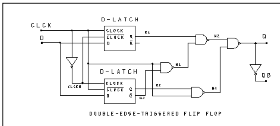
Figure 24-5: Double-Edge Triggered Flip-Flop Schematic
