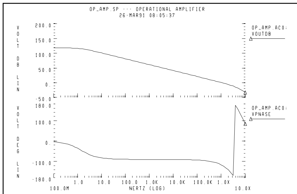
Figure 24-25: AC Analysis Response
