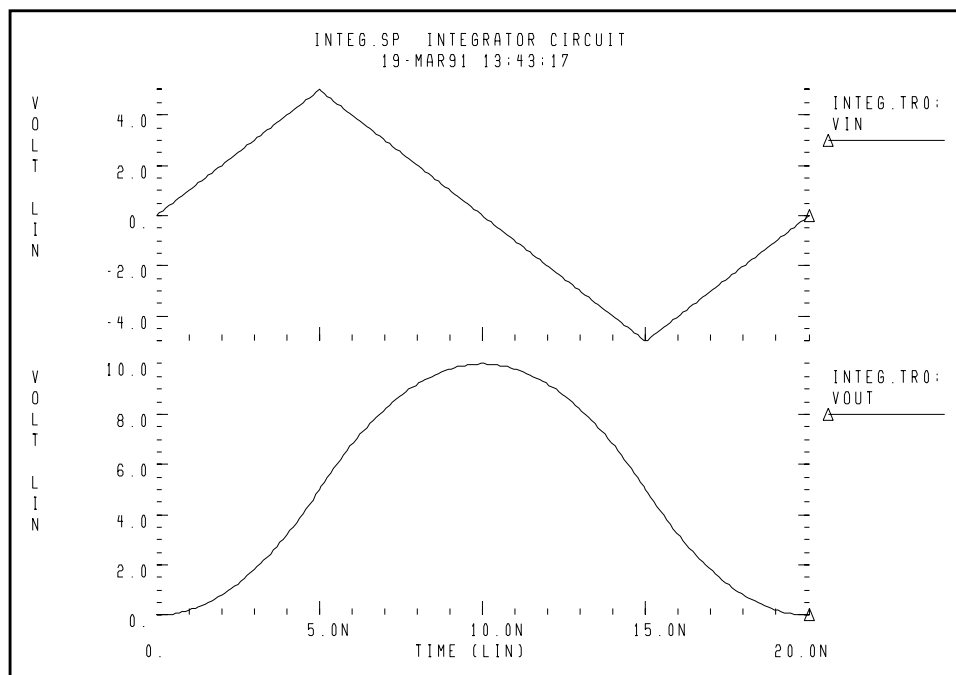
Figure 24-15: Response of Integrator to a Triangle Waveform
