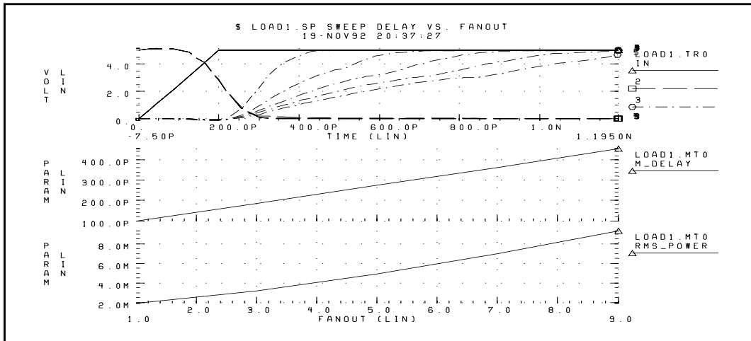
Figure 22-4: Inverter Delay and Power versus Fanout
