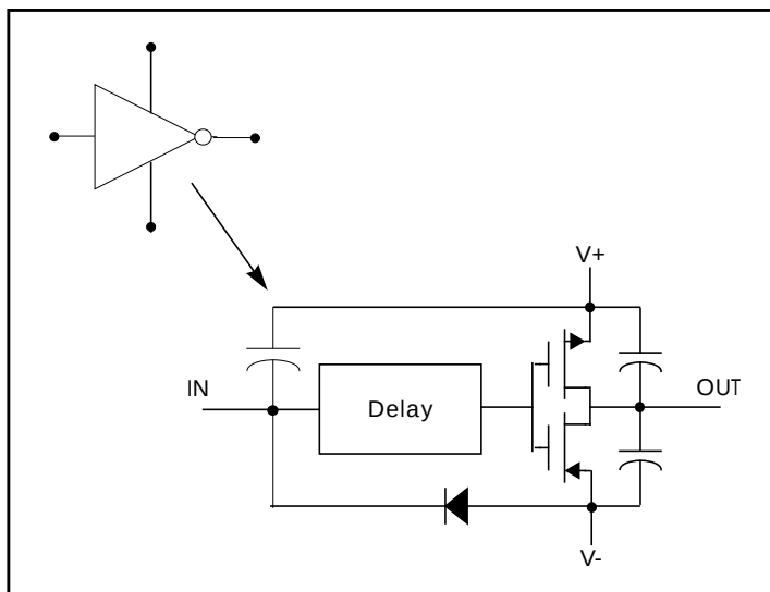
Figure 24-8: Inverter
