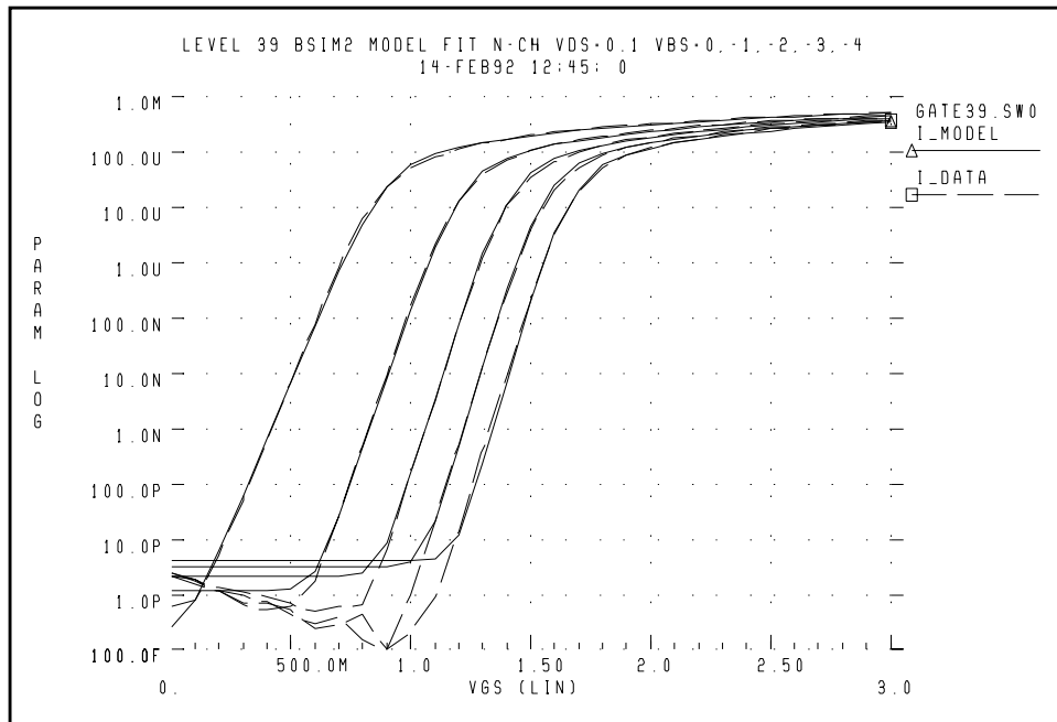
Figure 20-10: I_{DS} vs. V_{GS} for V_{DS} = 0.1V , V_{BS} = 0, -1, -2, -3, -4V , Showing Subthreshold Region; Model vs. Data
