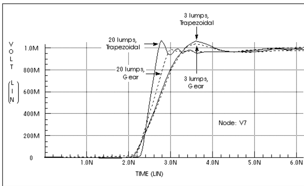
Figure B-27: Computed Responses for 20 Lumps and 3 Lumps, Gear and Trapezoidal Integration Methods
