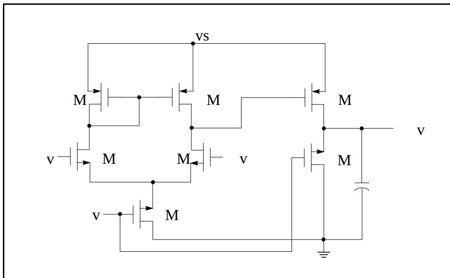
Figure 12-31: CMOS Op-amp
