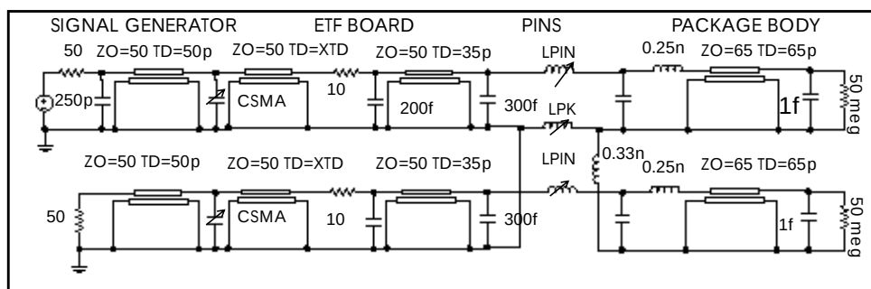
Figure 23-5: SPICE Model for Package-Plus-Test Fixture Optimized Parameters: XTD, CSMA, LPIN, and LPK
