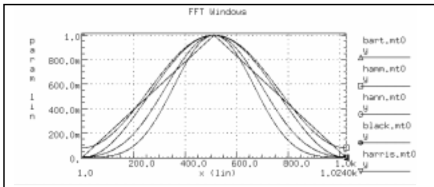
Figure 26-1: FFT Windows
