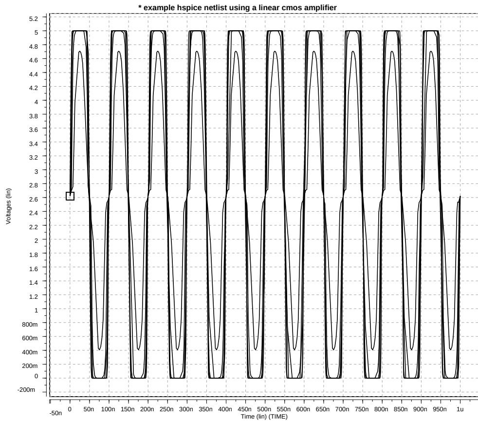
Figure E-5: Plot of Voltage on Node inv2out vs. Time
