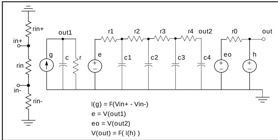
Figure 24-24: Op-Amp Circuit
