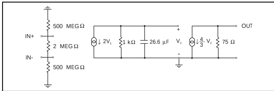
Figure 25-7: Linear Model of the 741C Op-Amp
