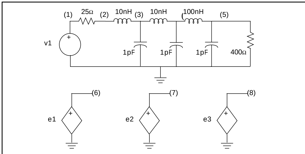
Figure 27-11: Circuits for a Low-Loss Line
