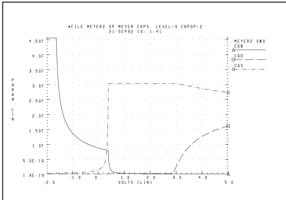
Figure 19-23: CAPOP=2 Capacitances for Level 3 Model
