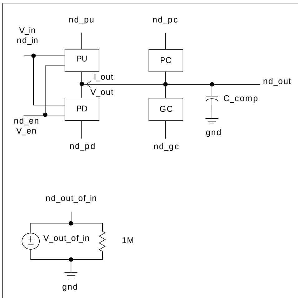
Figure 18-5: Input-Output Buffer
