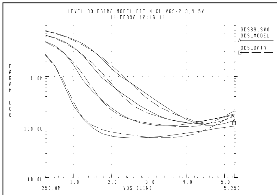
Figure 20-9: g_{ds} vs. V_{ds} for V_{gs} = 2, 3, 4, 5V ; BSIM2 Model vs. Data, LOG scale
