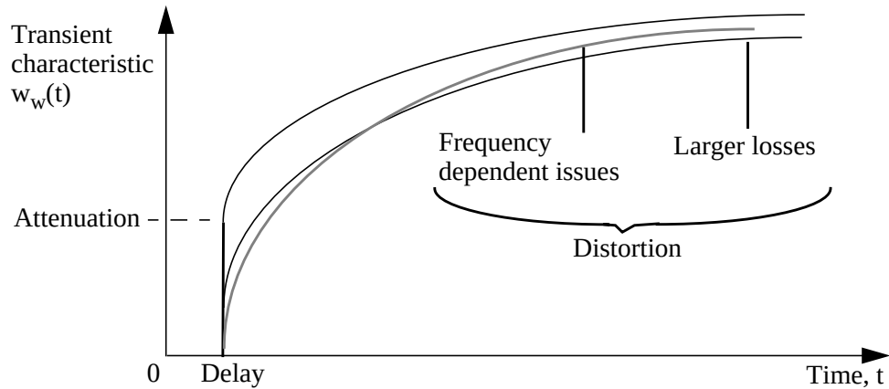
Figure 17-4: Propagation Function Transient Characteristics (unit-step response)
