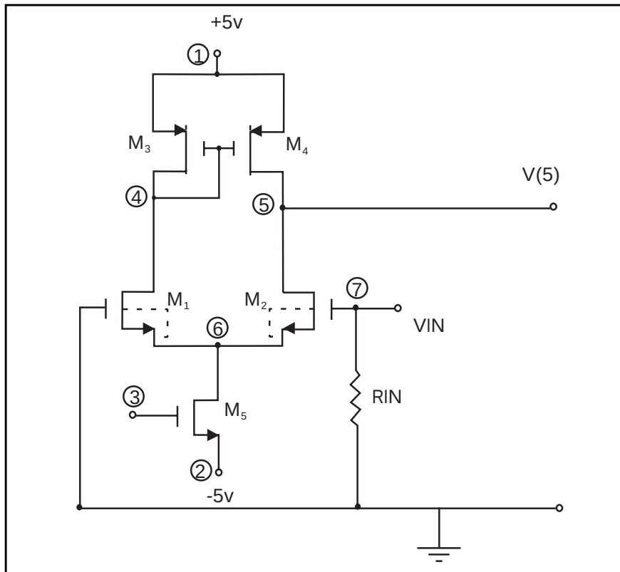
Figure 25-5: CMOS Differential Amplifier
