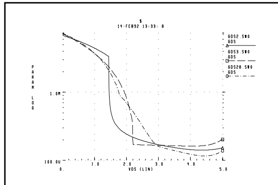
Figure 20-37: Levels 2, 3, 28 gds vs. Vds Curves
