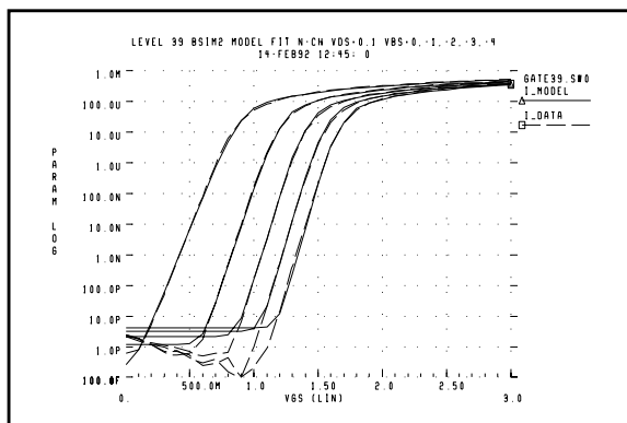
Figure 20-30: Level 39 Ids vs. Vgs Curves
