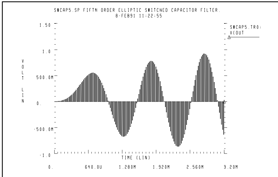
Figure 27-23: Response to 1-kHz Sinusoidal Input
