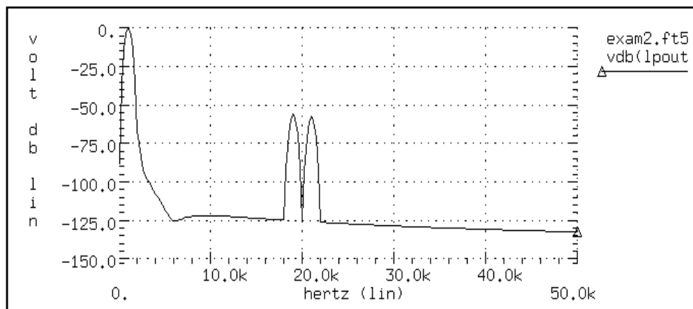
Figure 26-14: Filtered Output Signal (Blackman-Harris window)
