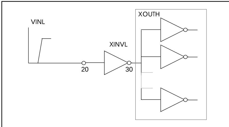
Figure 22-8: Cell Characterization Circuit 2
