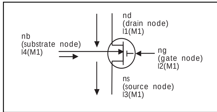
Figure 19-7: MOSFET Current Convention, N-channel
