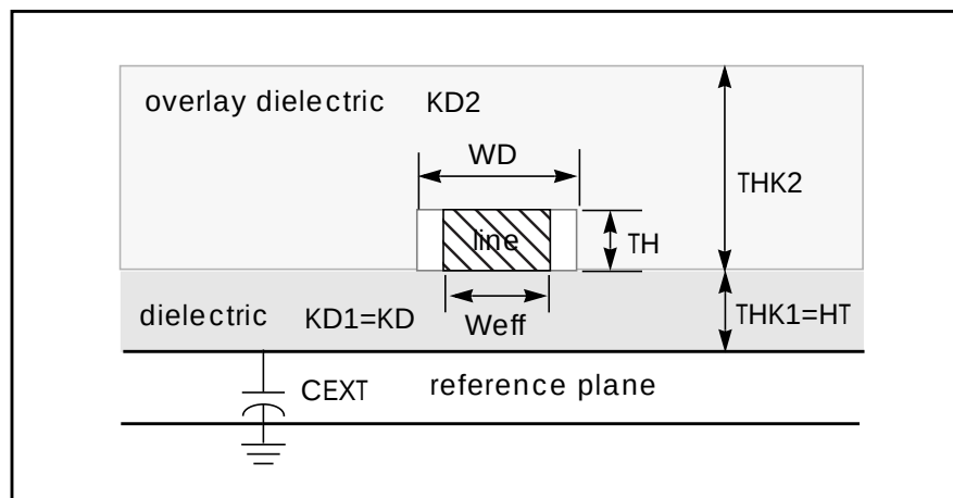
Figure B-14: Planar Transmission Line, DLEV=3, Overlay Dielectric
