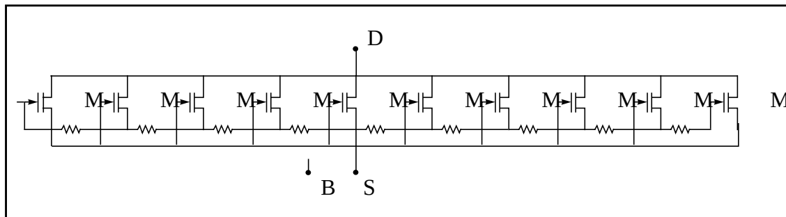
Figure 29-13: Nine-stage Ladder Model
