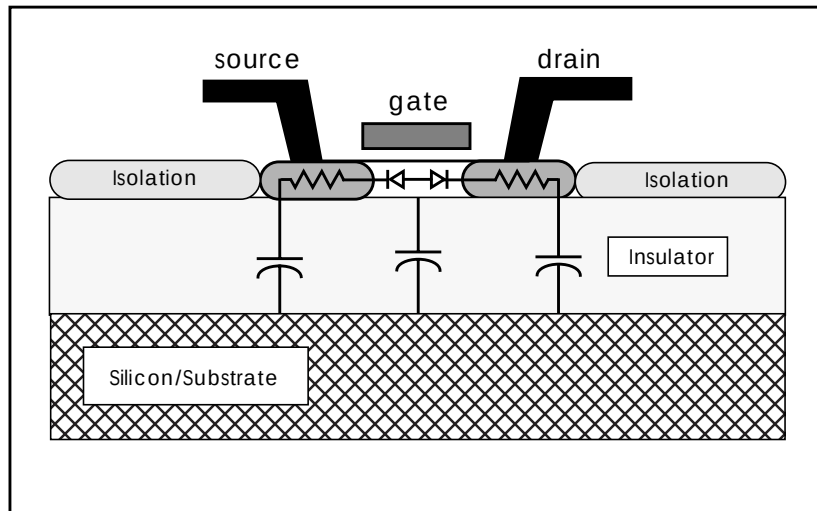
Figure 20-6: Non-fully Depleted SOI Model
