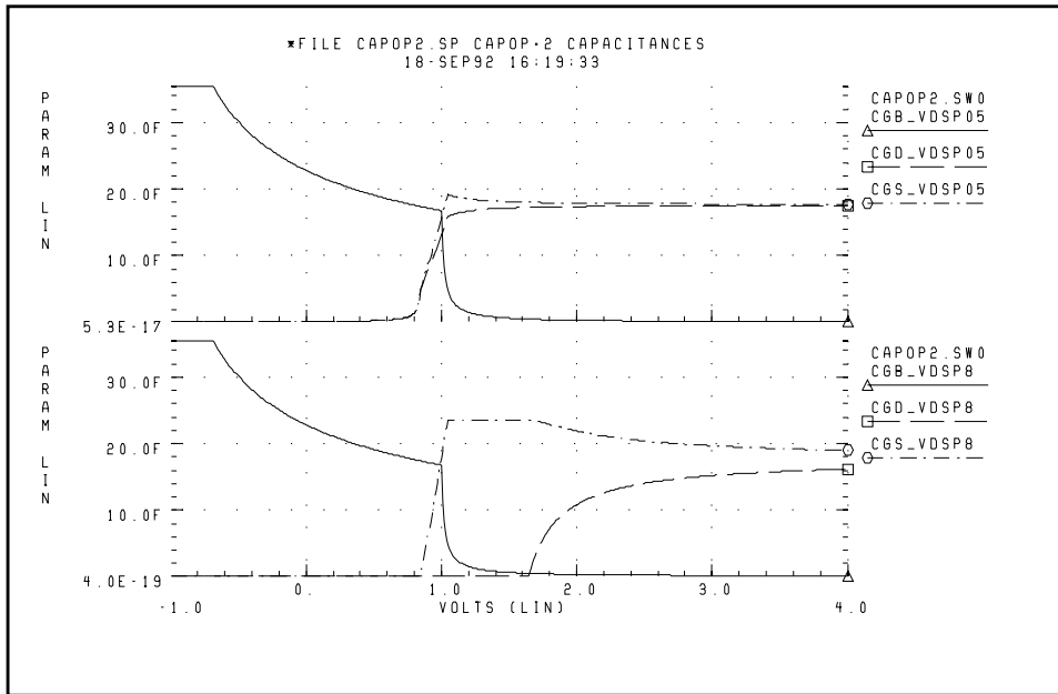
Figure 19-21: CAPOP=2 Capacitances
