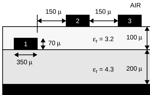
Figure 17-14: Three Traces Immersed in Stratified Dielectric Media
