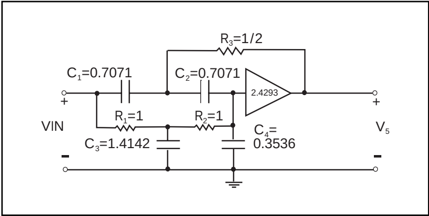
Figure 25-3: Design Example for Kerwin’s Circuit
