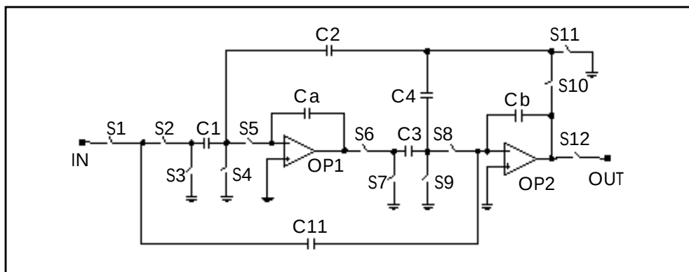
Figure 27-22: Low_Q Biquad Section
