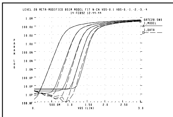
Figure 20-26: Level 28 Ids vs. Vgs Curves
