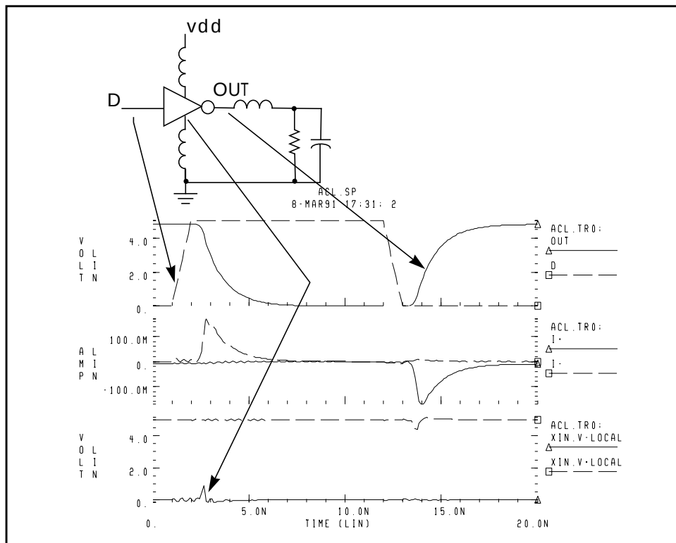
Figure 24-7: ACL Family Output Buffer
