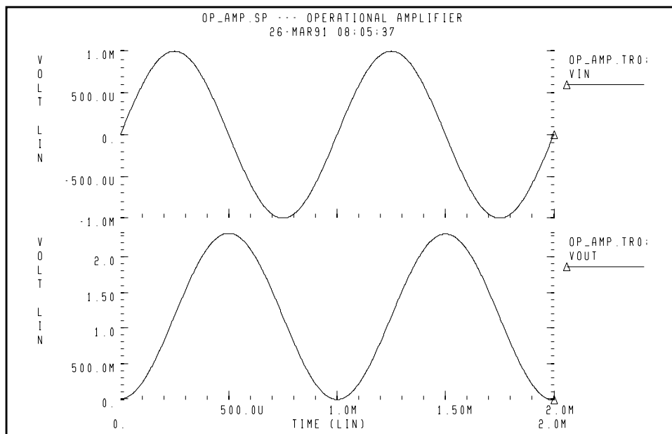
Figure 24-26: Transient Analysis Response 1 .
