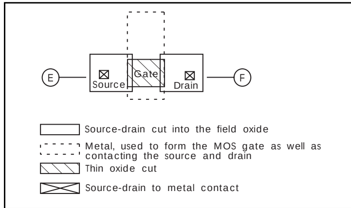
Figure 19-1: Field Effect Transistor
