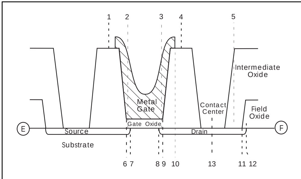
Figure 19-2: Field Effect Transistor Geometry
