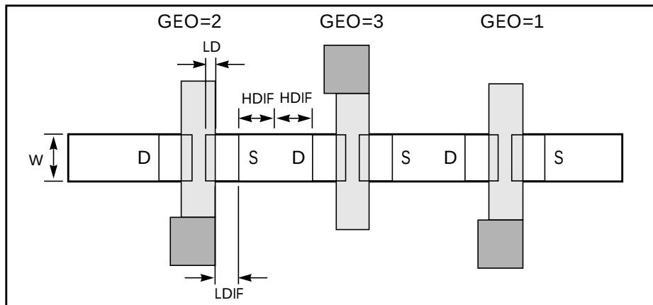
Figure 19-14: Stacked Devices and Corresponding GEO Values
