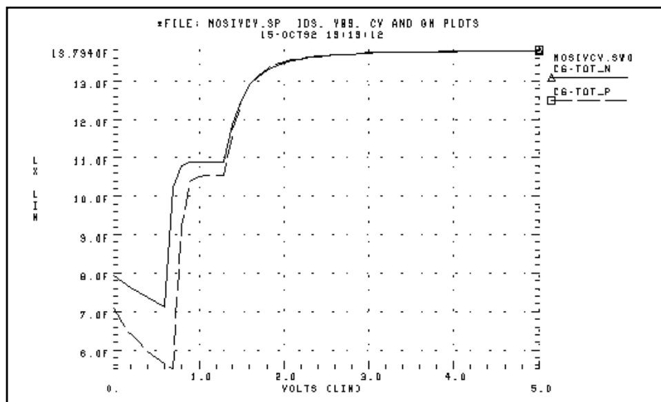
Figure 29-9: Asic1.sp Demo Local Supply Voltage
