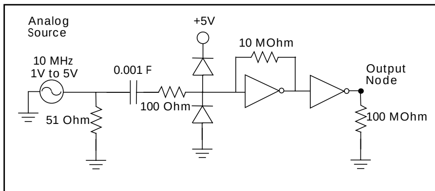
Figure E-1: Circuit Diagram for Linear CMOS Inverter
