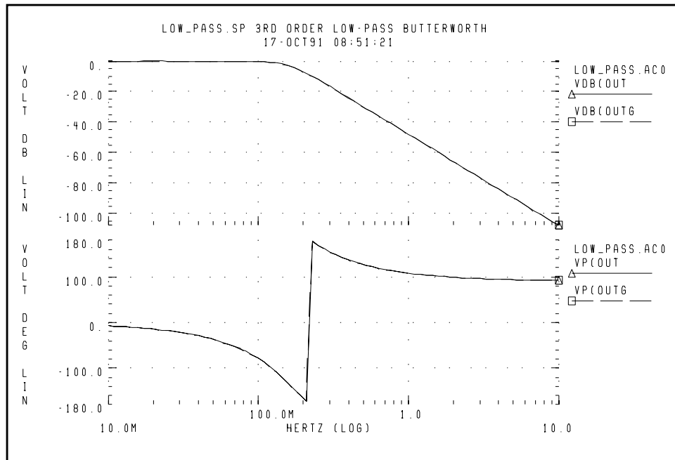
Figure 27-5: Frequency Response of Circuit and Functional Element
