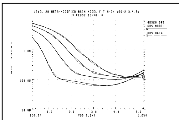
Figure 20-23: Level 28 gds vs. Vds Curves
