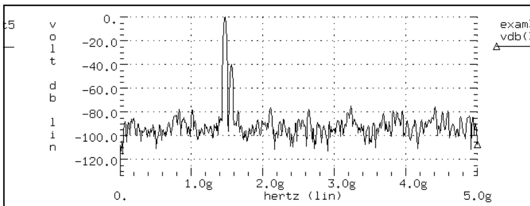
Figure 26-20: Mixer Output Spectrum, Blackman-Harris Window
