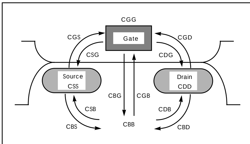
Figure 19-17: MOS Capacitances
