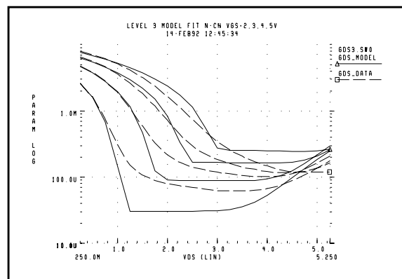
Figure 20-21: Level 3 gds vs. Vds Curves
