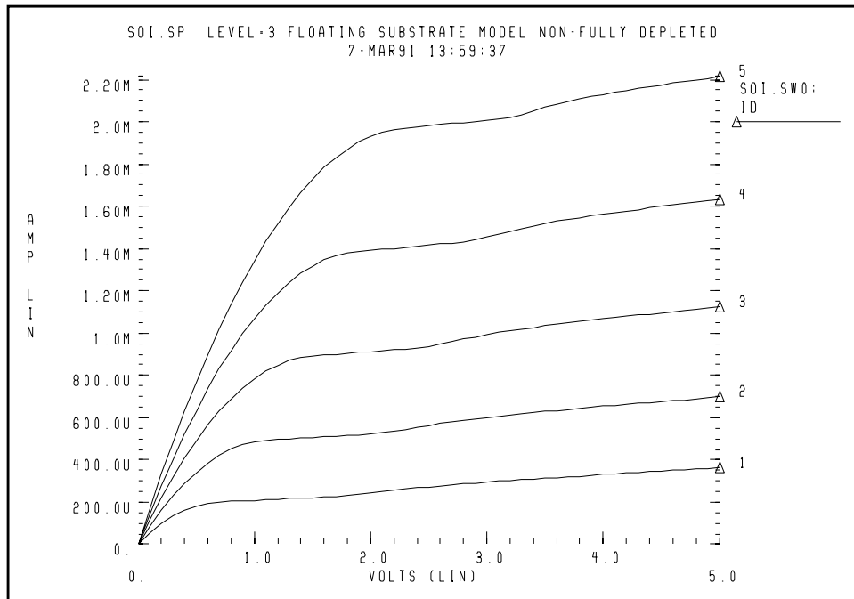
Figure 20-7: Level 3 Floating Bulk Model
