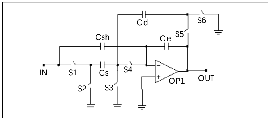
Figure 27-20: Linear Section
