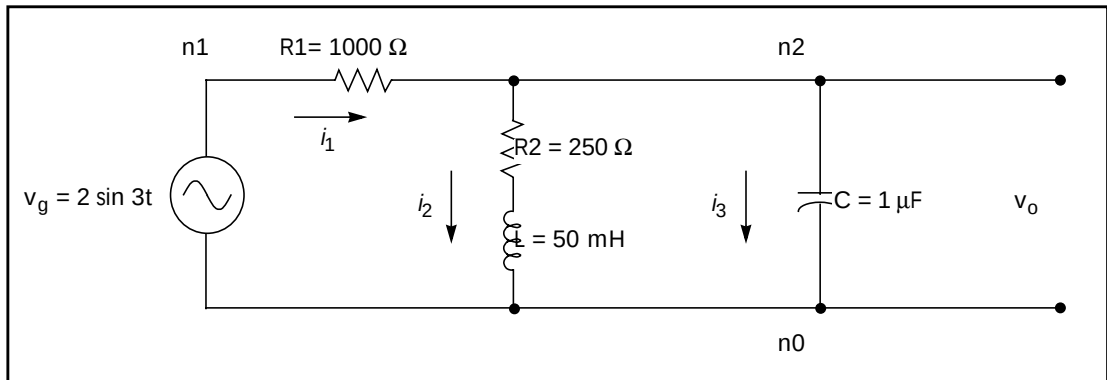
Figure 27-7: LAPLACE Example 1 Circuit
