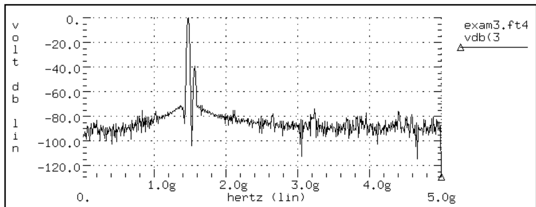
Figure 26-19: Mixer Output Spectrum, Blackman Window
