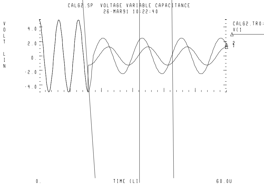
Figure 24-30: Correct Result Corresponding to CTYPE=1
