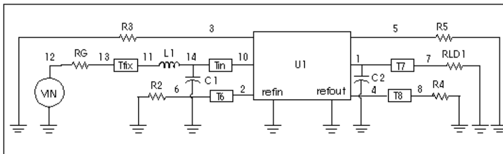
Figure B-23: Schematic Using the Three Coupled Striplines U Model
