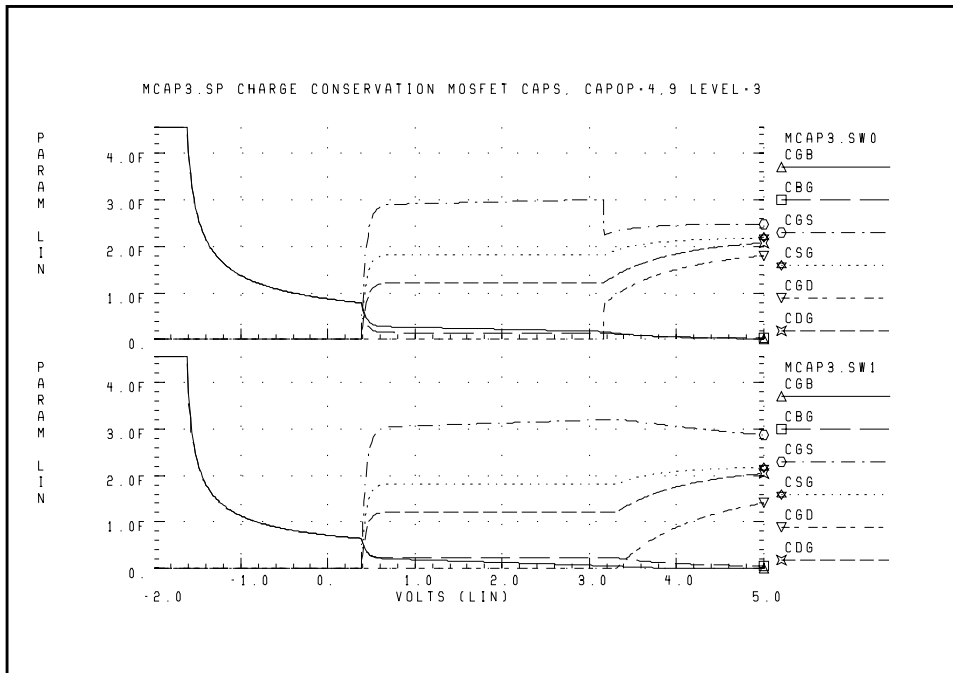
Figure 19-22: CAPOP=4, 9 Capacitances for Level 3 Model
