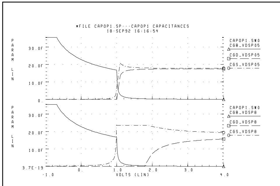
Figure 19-20: CAPOP=1 Capacitances
