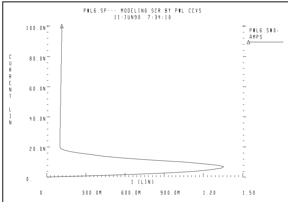
Figure 24-20: Silicon Controlled Rectifier
