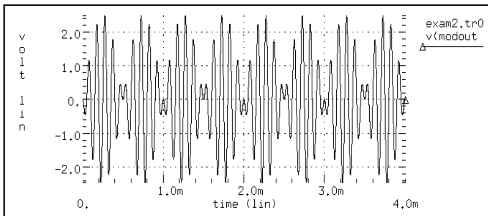
Figure 26-7: Modulated Signal
