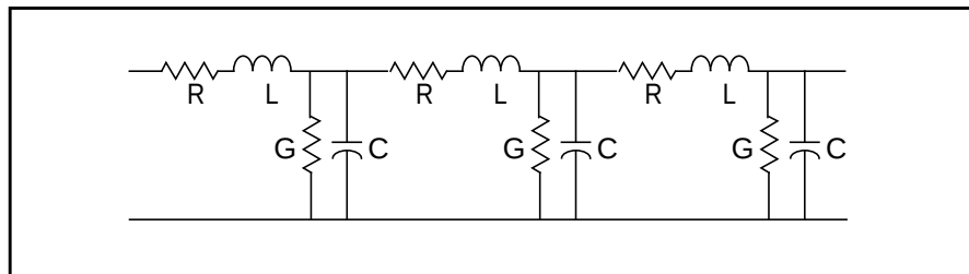
Figure B-48: Lossy Transmission Line Model
