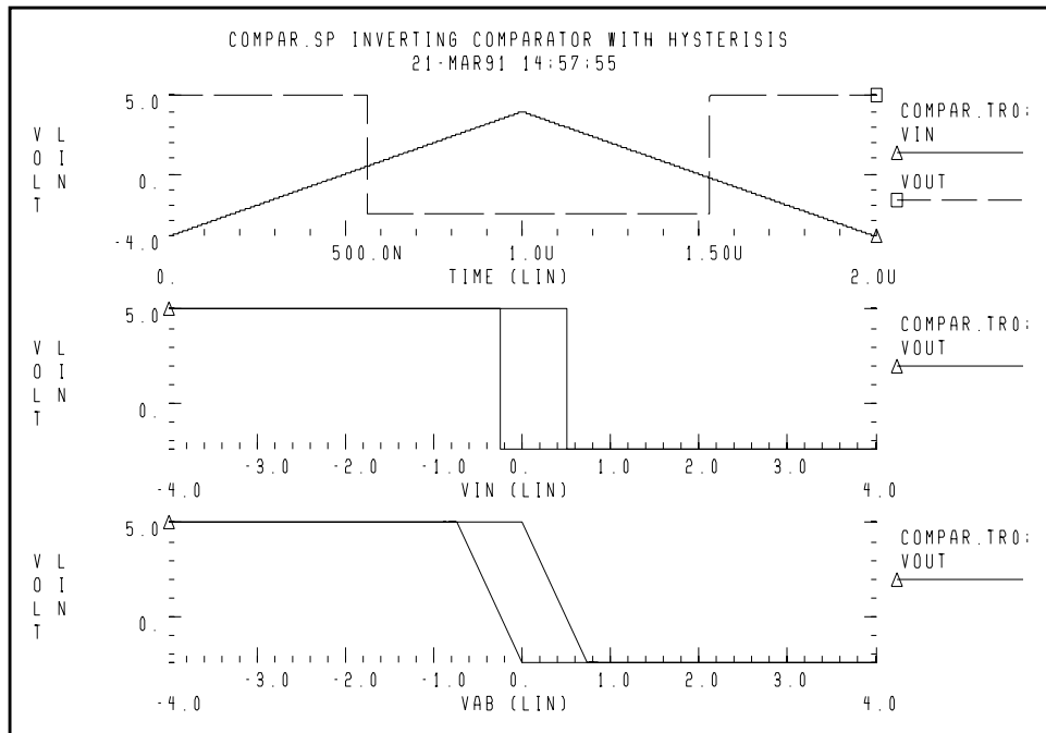
Figure 24-28: Response of Comparator
