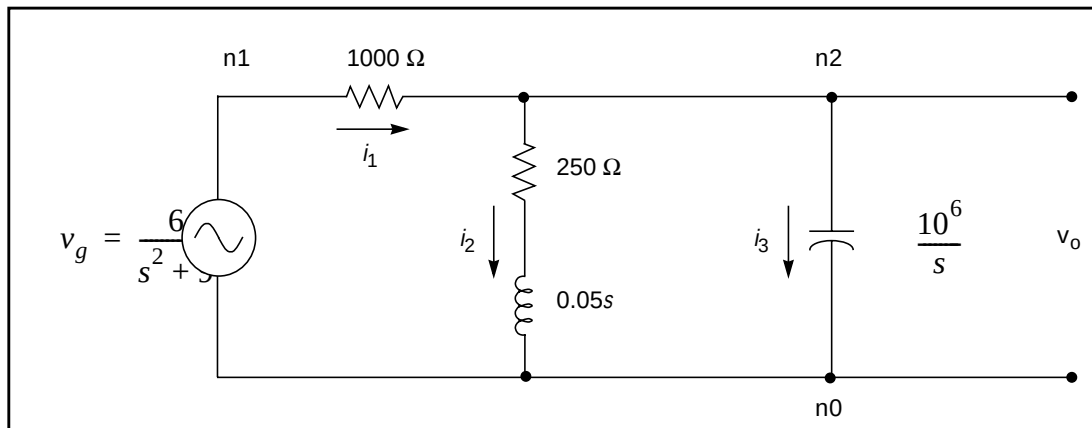
Figure 27-8: S-Domain Equivalent of the LAPLACE Example 1 Circuit
