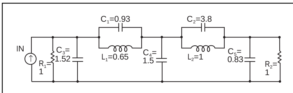
Figure 25-1: Low-Pass Prototype Filter
