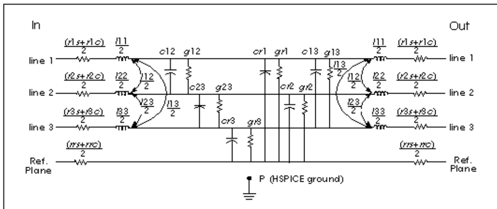
Figure B-19: Precomputed Components for Three Conductors and a Reference Plane
