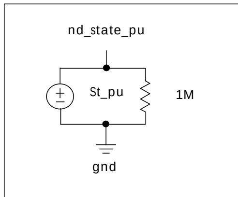
Figure 18-10: Equivalent Circuit for xv\_pu=nd\_state\_pu Keyword
