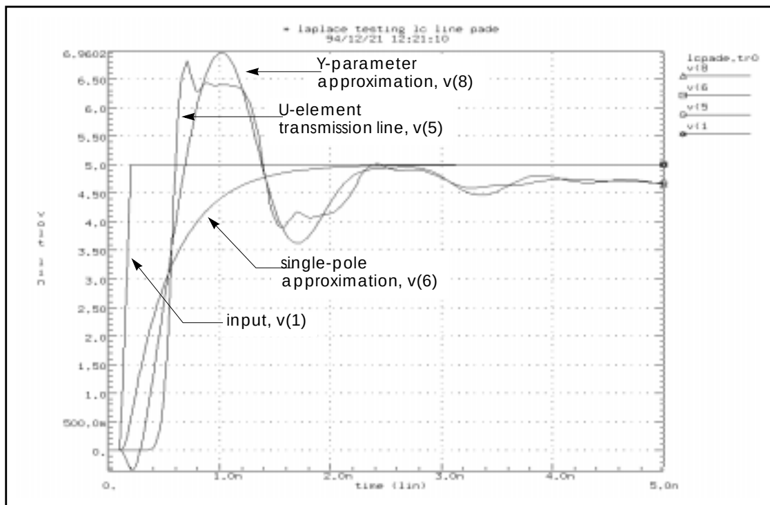
Figure 27-16: Transient Response of the Y-Parameter Line Model
