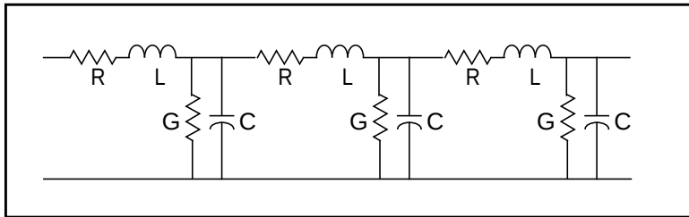
Figure B-45: Equivalent Circuit Model of a Lossy Transmission Line
