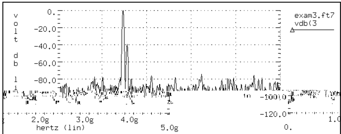
Figure 26-22: Mixer Output Spectrum, Kaiser-Bessel Window
