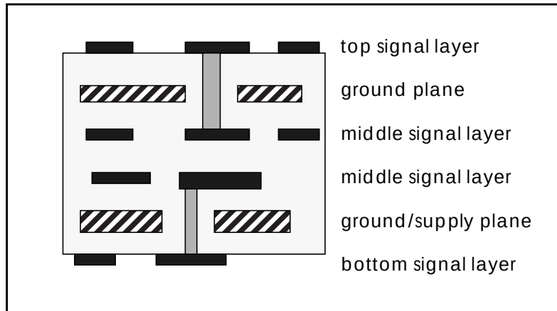
Figure B-37: Six-Layer Printed Circuit Board
