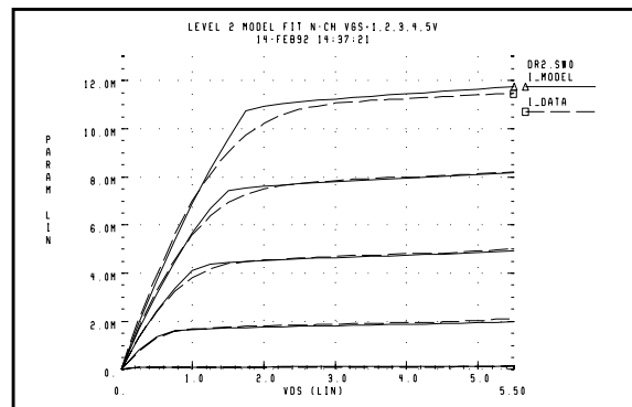
Figure 20-13: Level 2 Ids Model vs. Data Curves
