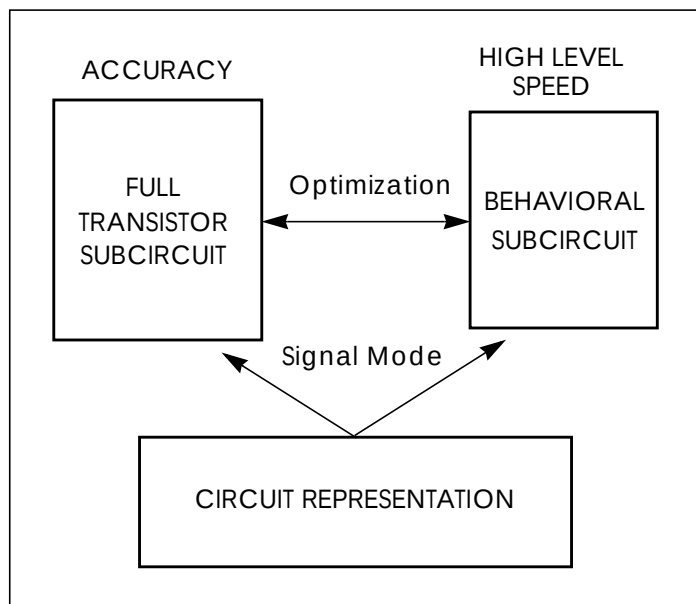
Figure 24-1: Netlisting by Signal Mode
