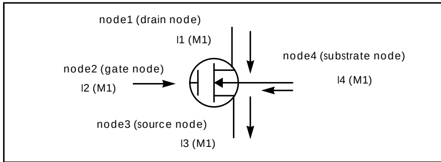
Figure 21-3: MOSFET (node1, node2, node3, node4) - n-channel
