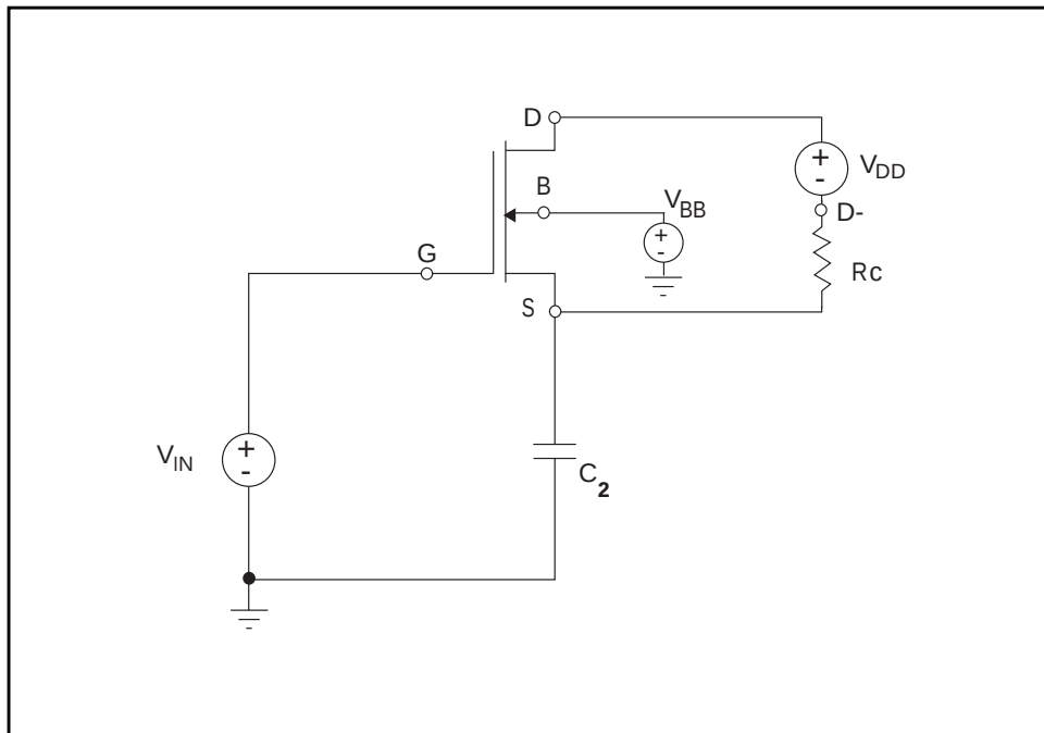
Figure 19-24: Charge Pump Circuit
