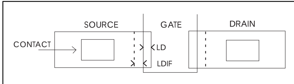
Figure 19-12: ACM=1 MOS Diode
