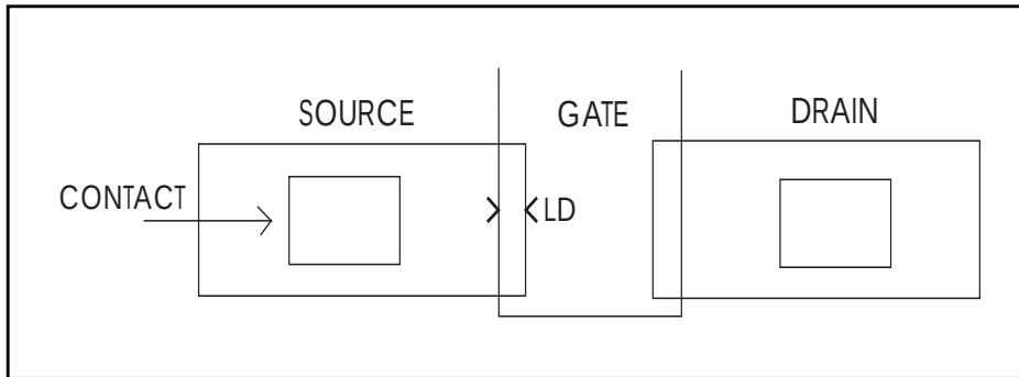
Figure 19-11: ACM=0 MOS Diode
