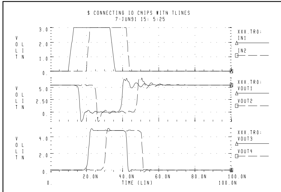
Figure 23-12: Connecting I/O Chips with Transmission Lines
