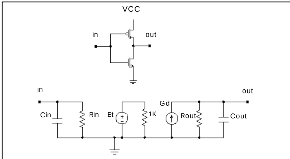
Figure 24-11: CMOS Inverter and its Equivalent Circuit
