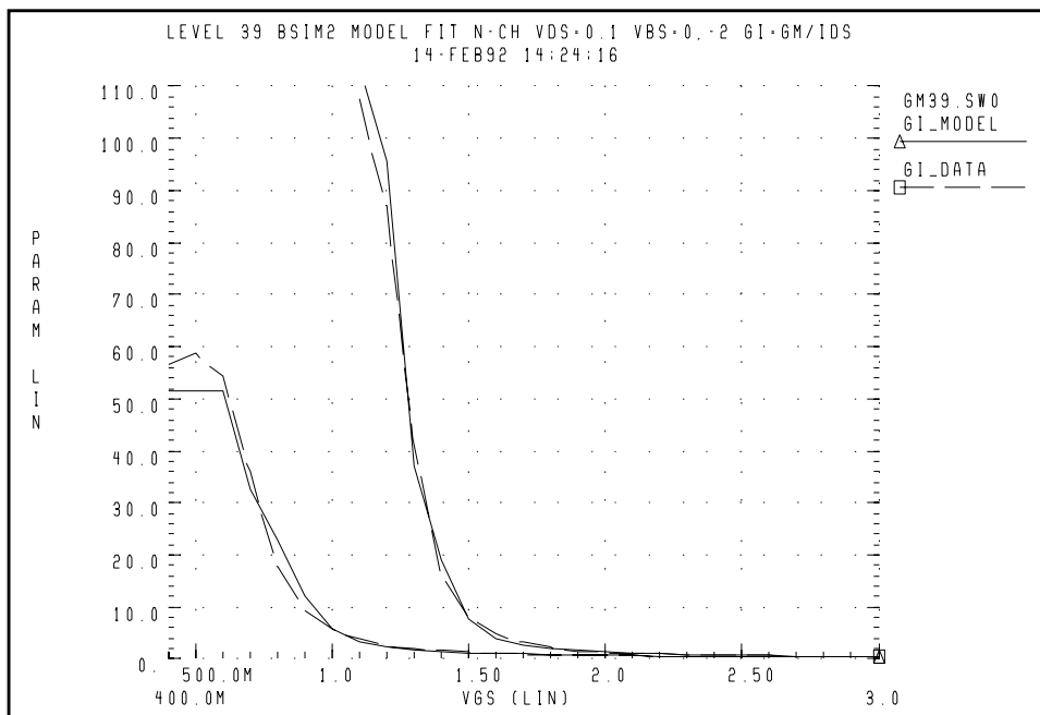
Figure 20-11: g_m/I_{DS} vs. V_{gs} for V_{ds} = 0.1V , V_{bs} = 0, -2V ; BSIM2 Model vs. Data
