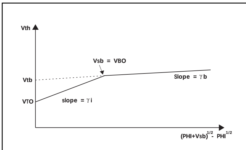
Figure 20-1: Threshold Voltage Variation
