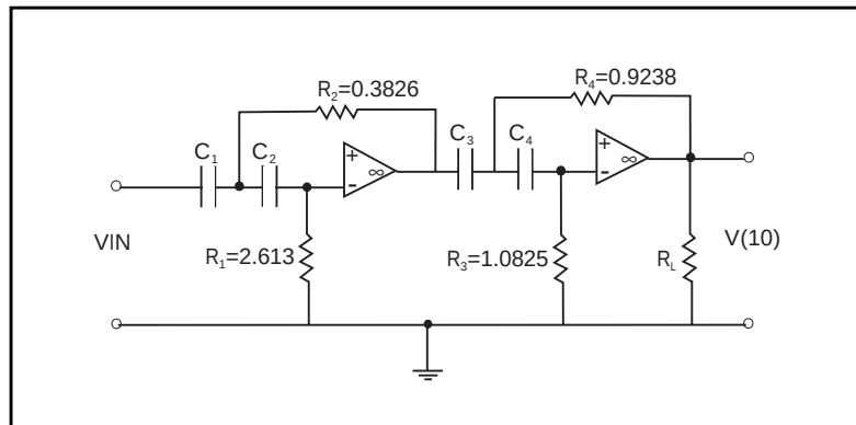
Figure 25-4: Fourth-Order High-Pass Butterworth Filter
