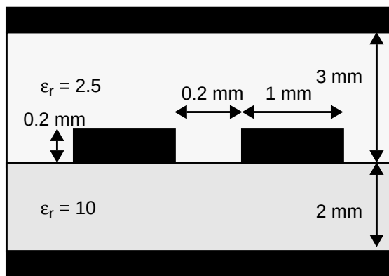
Figure 17-16: Two Traces Between Two Ground Planes
