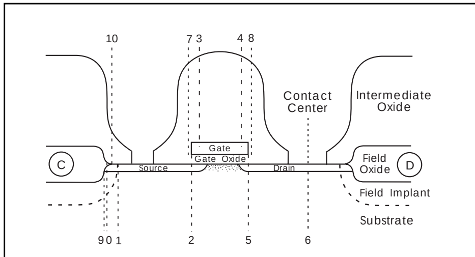
Figure 19-5: Isoplanar MOSFET Construction, Part B
