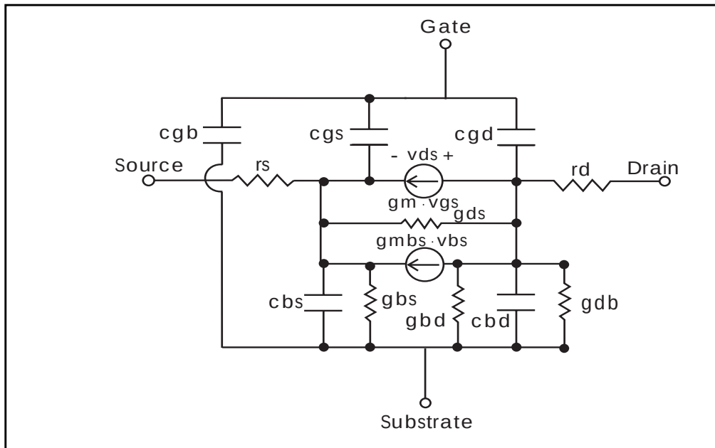
Figure 19-9: Equivalent Circuit, MOSFET AC Analysis
