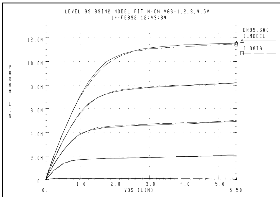
Figure 20-8: I_{DS} vs. V_{ds} for V_{gs} = 1, 2, 3, 4, 5V ; BSIM2 Model vs. Data
