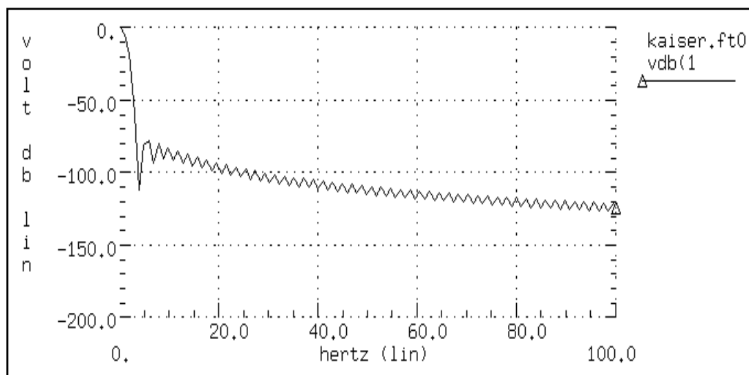
Figure 26-3: Kaiser-Bessel Window Characteristics, ALFA=3.0
