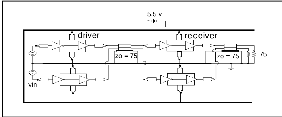
Figure 23-11: I/O Drivers/Receivers with Package Lead Inductance, Parallel 4" Lossy Microstrip Connectors
