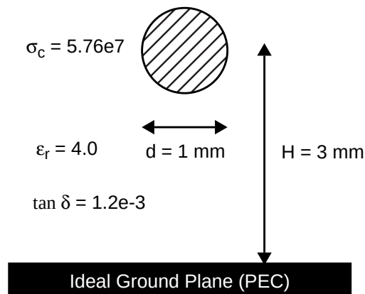
Figure 17-13: Cylindrical Conductor Above a Ground Plane
