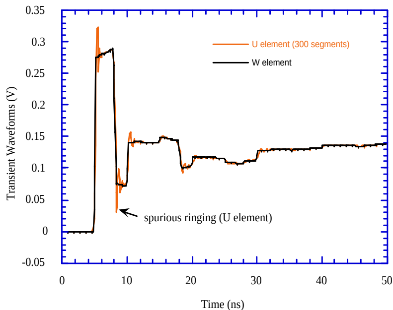
Figure 17-5: Spurious Ringing in U Element
