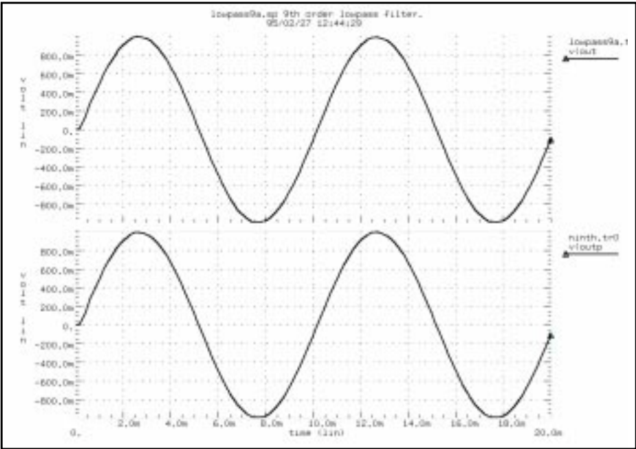
Figure 27-17: Transient Responses of the Circuit and Pole/Zero Models
