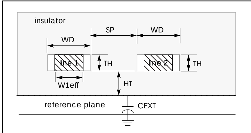
Figure B-11: Planar Transmission Line, DLEV=0, Sea of Dielectric
