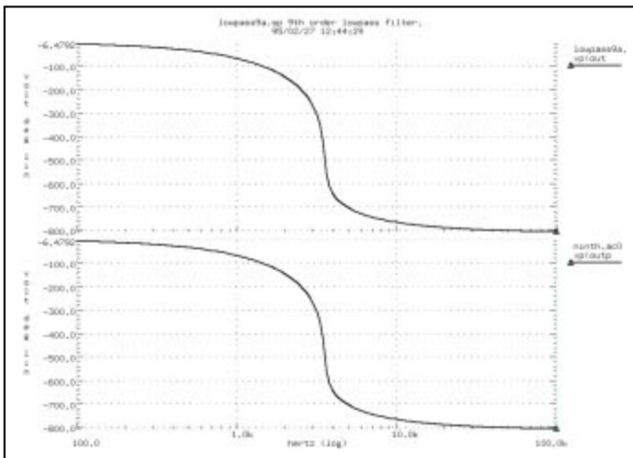
Figure 27-18: AC Analysis Responses of the Circuit and Pole/Zero Models
