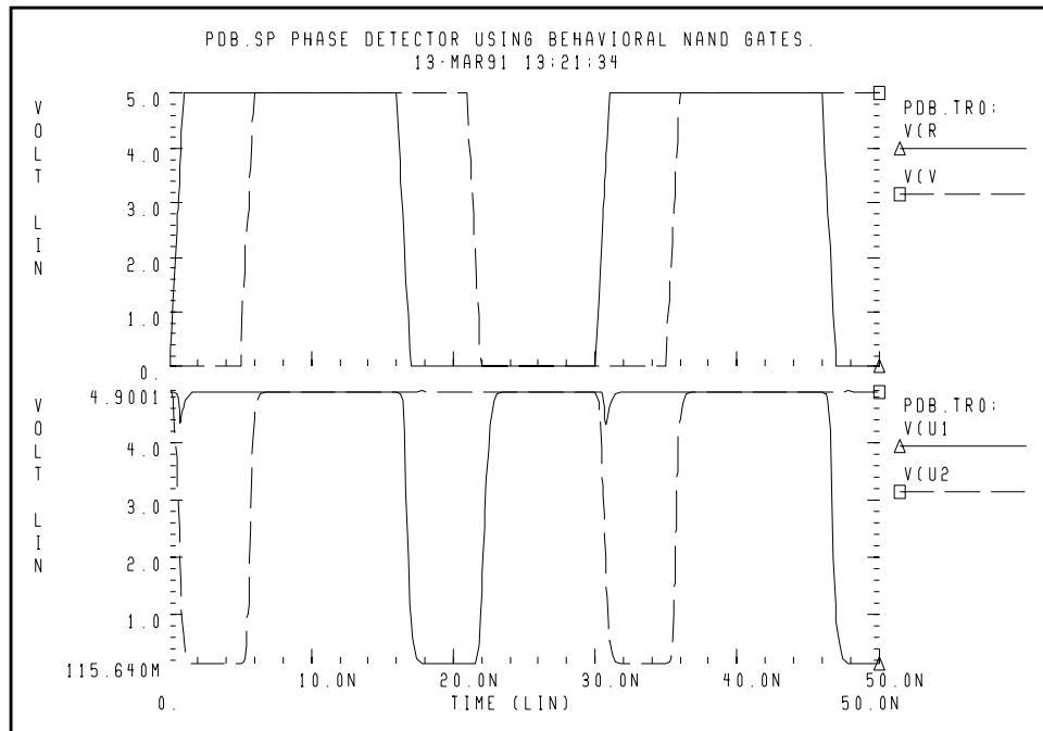
Figure 24-33: Phase Detector Response
