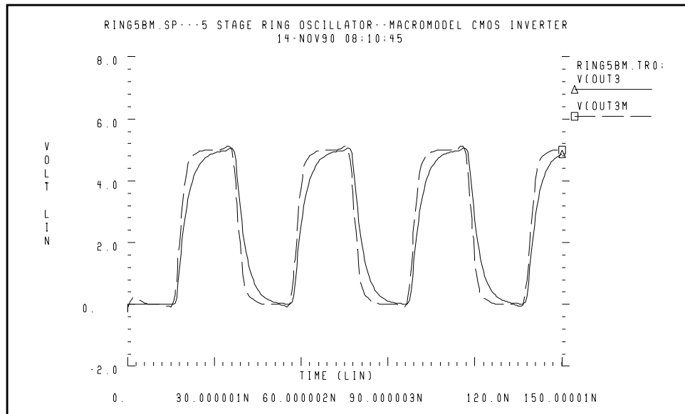
Figure 24-13: Ring Oscillator Response
