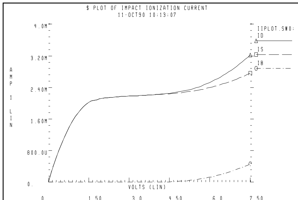
Figure 19-15: Drain, Source, and Bulk Currents for v_{gs}=3 , with IIRAT=0.5
