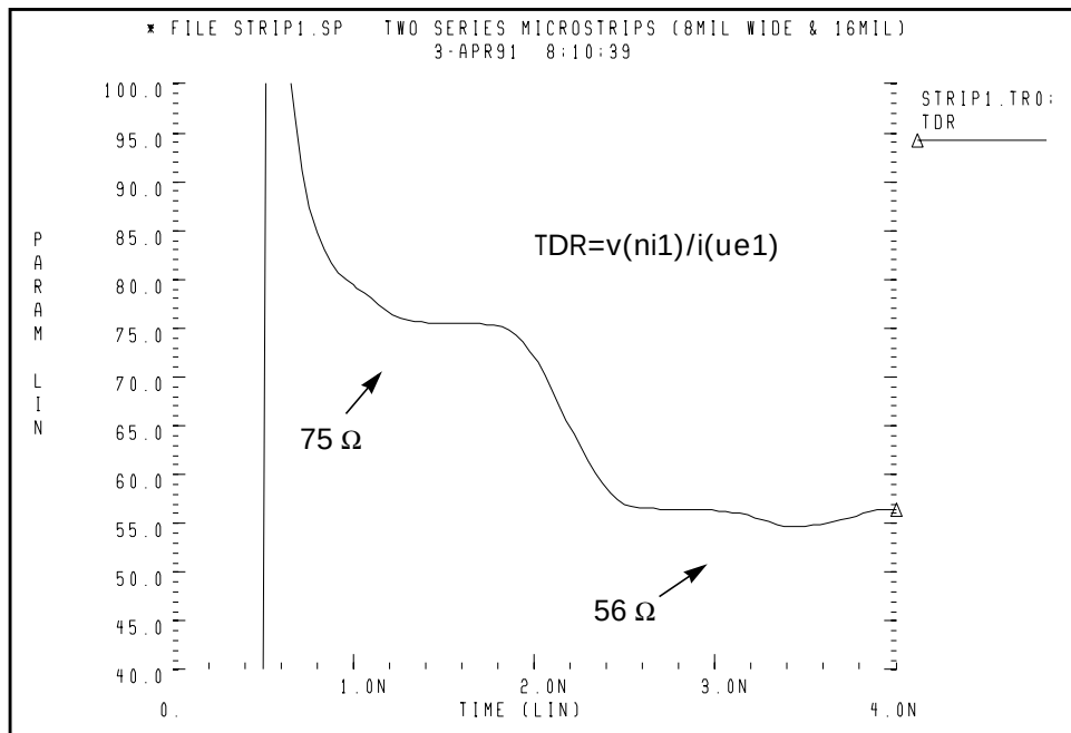
Figure B-43: Impedance from TDR at Input
