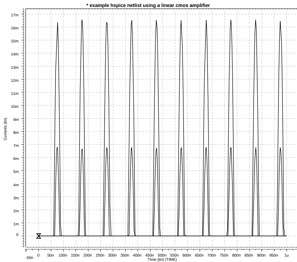
Figure E-6: Plot of Current through Diode dlow vs. Time
