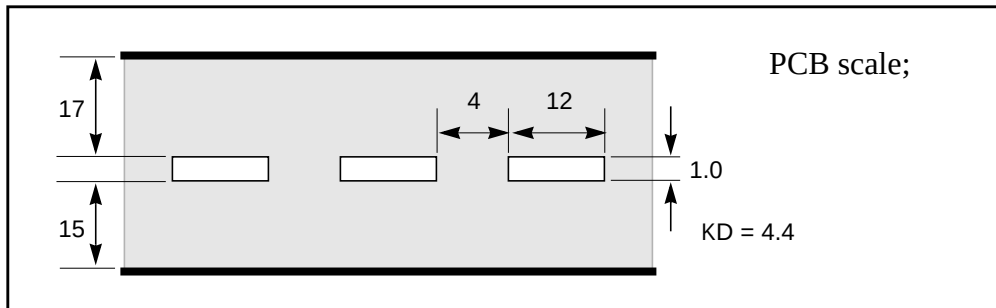
Figure B-22: Three Coupled Striplines (PCB Scale)
