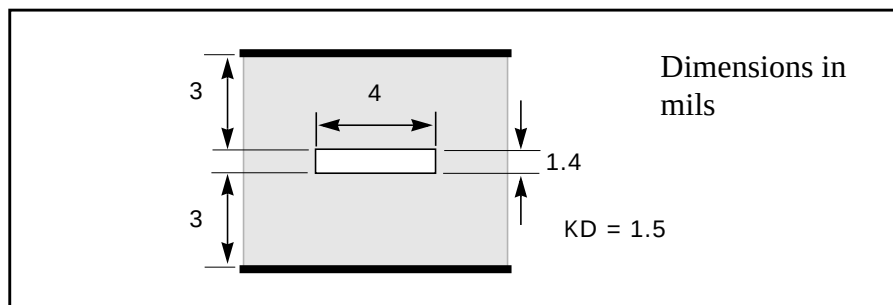
Figure B-35: Stripline Geometry Used in MCM Technology
