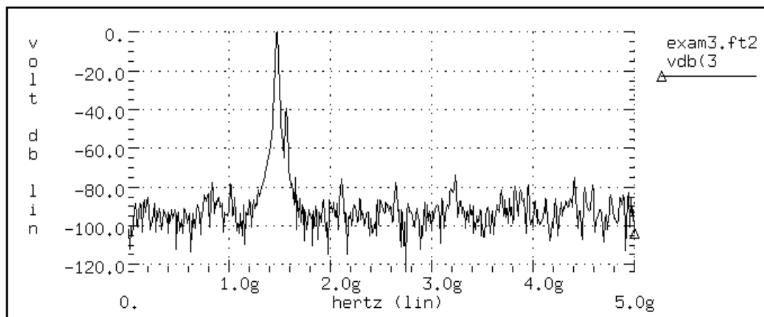
Figure 26-17: Mixer Output Spectrum, Hanning Window
