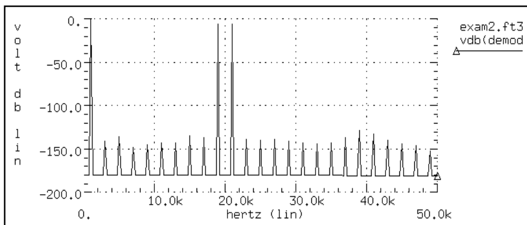
Figure 26-12: Demodulated Signal Spectrum
