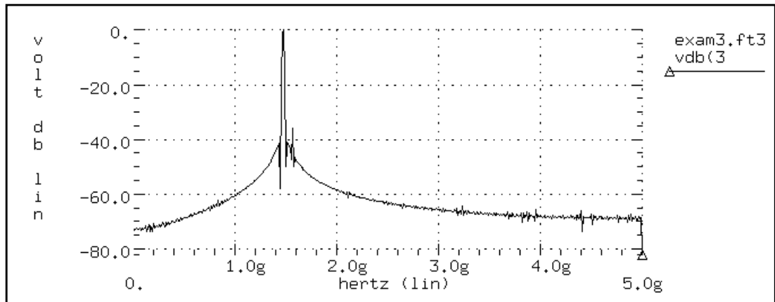
Figure 26-18: Mixer Output Spectrum, Hamming Window
