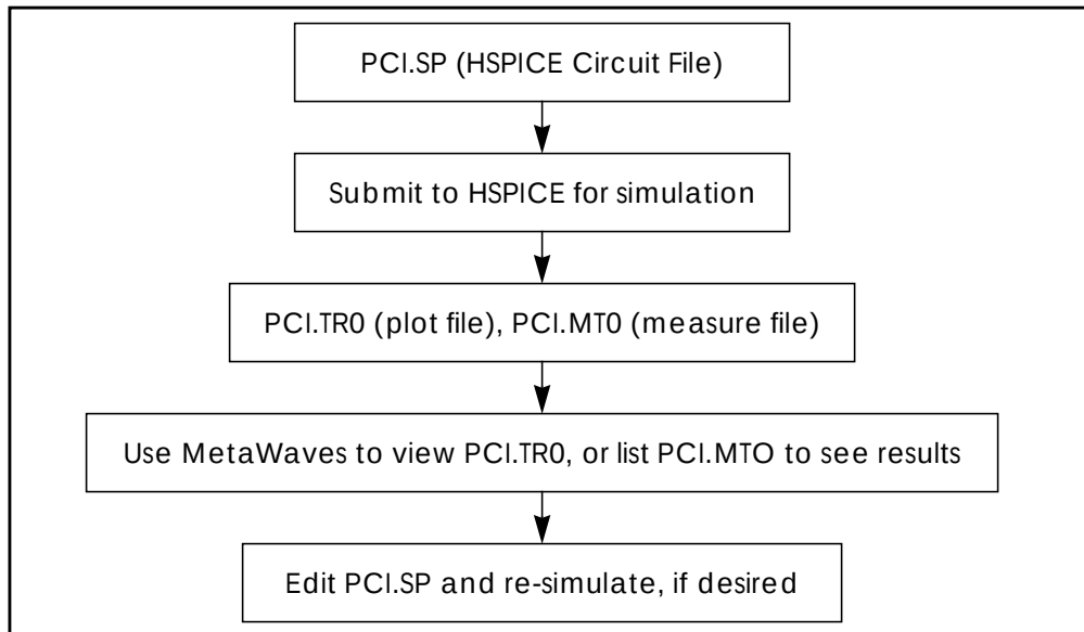
Figure 23-20: PCI Simulation Process
