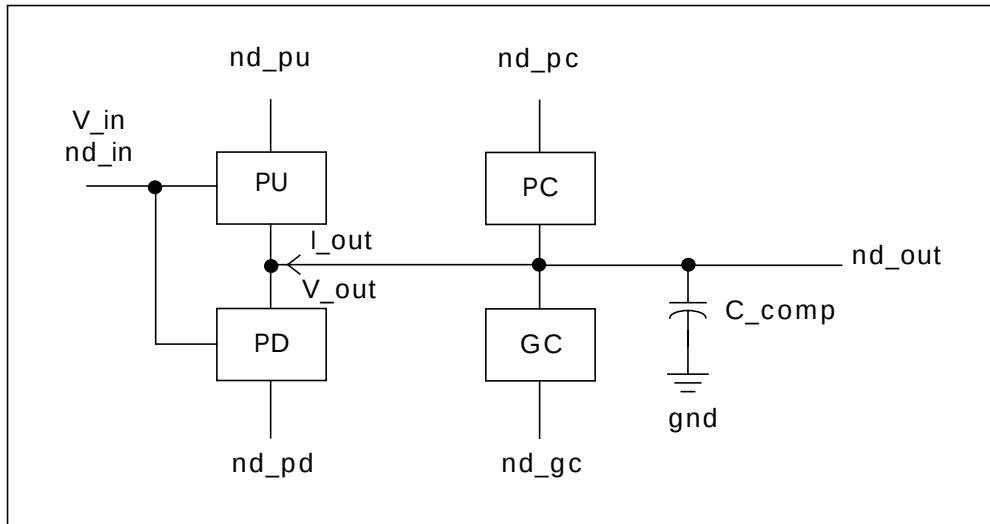
Figure 18-3: Output Buffer
