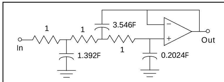
Figure 27-4: Third-Order Active Low-Pass Filter
