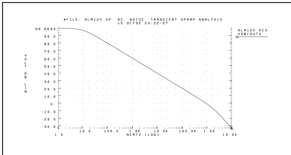
Figure 22-6: Magnitude Plot of Op-Amp Gain
