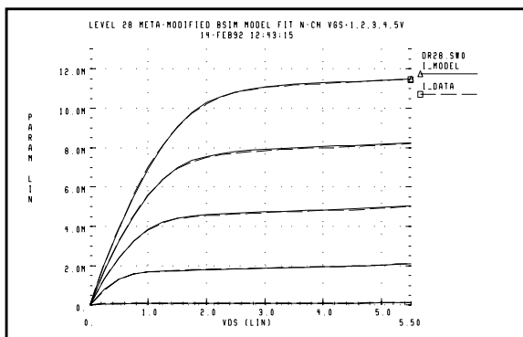
Figure 20-14: Level 28 Ids Model vs. Data Curves
