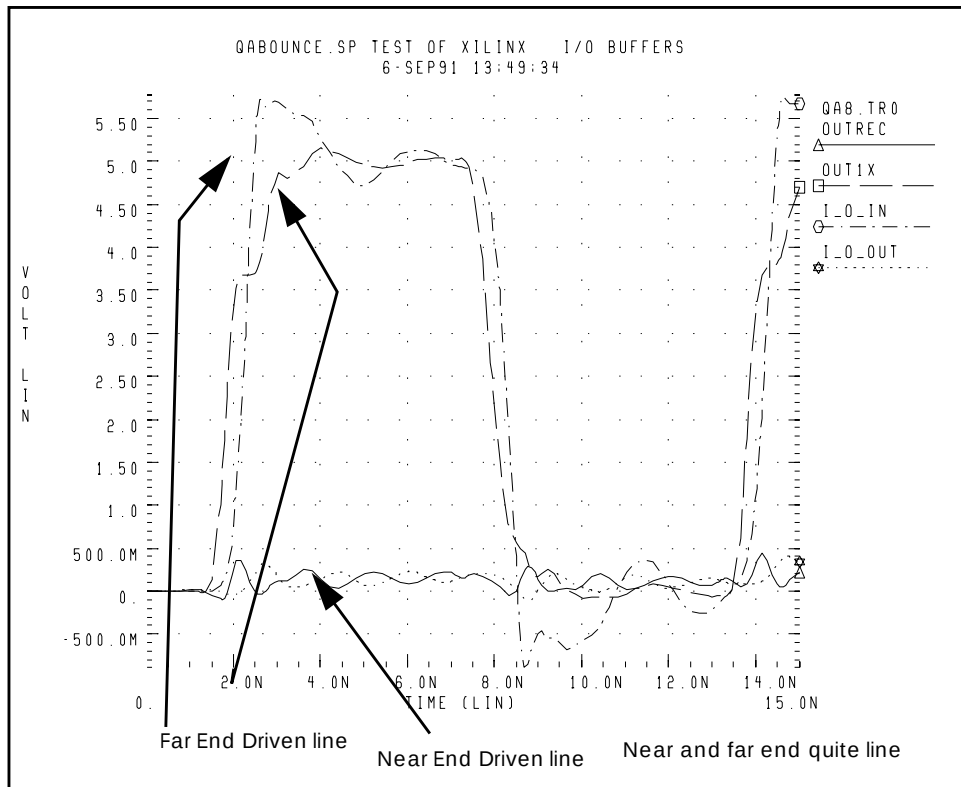
Figure 23-16: Results of Coupled Noise Simulation
