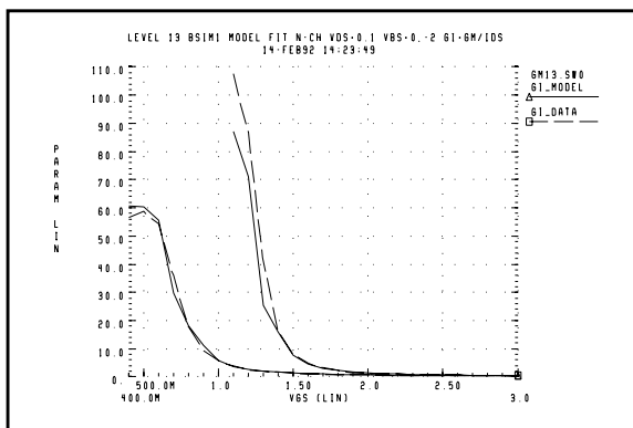
Figure 20-34: Level 13 gm/Ids vs. Vgs Curves
