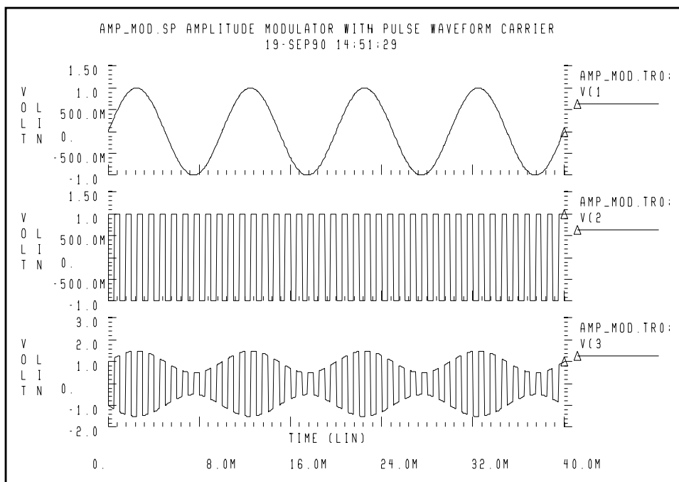
Figure 24-22: Amplitude Modulator Waveforms
