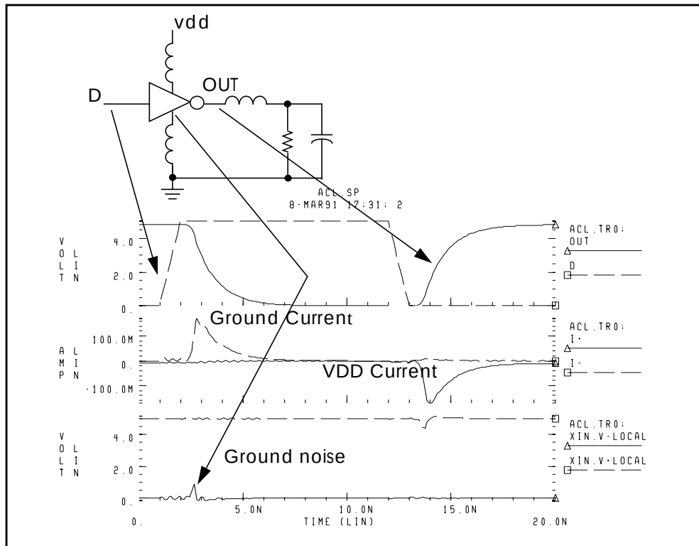
Figure 23-1: Simulation of Output Buffer with 2 ns Delay and 1.8 ns Rise and Fall Times
