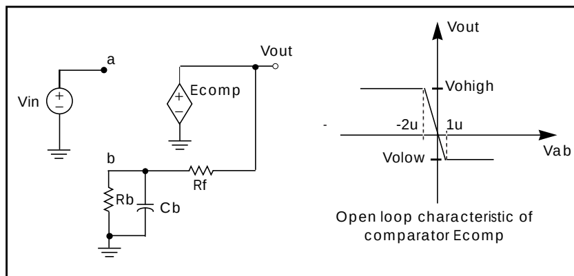
Figure 24-27: Inverting Comparator with Hysteresis
