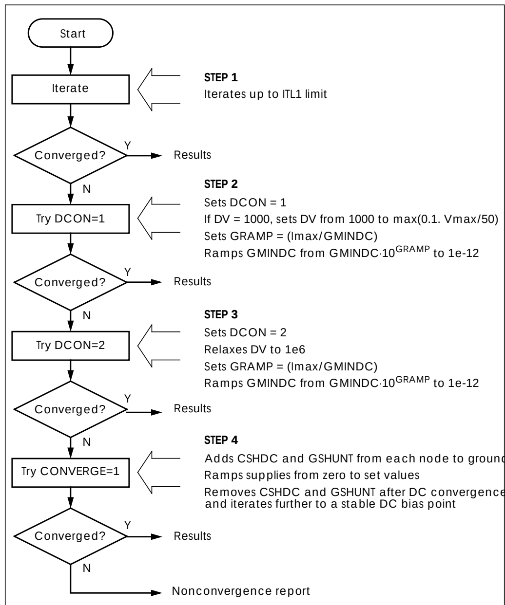
Figure 9-3: Autoconvergence Process Flow Diagram
