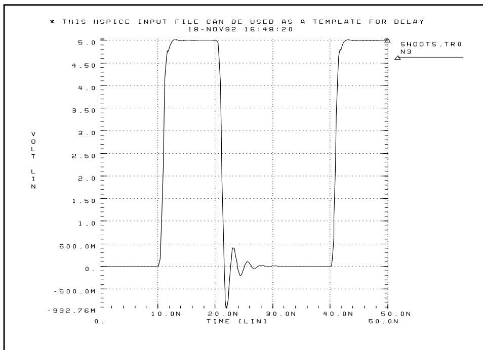
Figure 23-22: Overshoot Template Example
