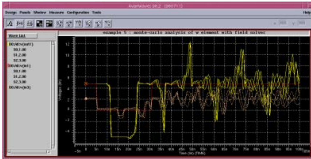
Figure 17-17: Monte-Carlo Analysis with a Field Solver and W Element
