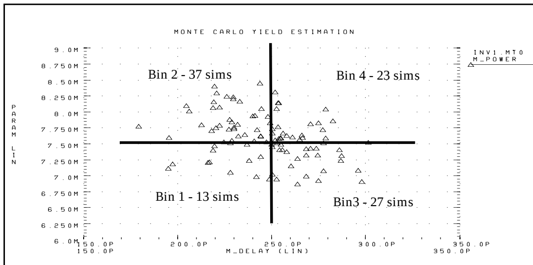
Figure 12-20: Speed/Power Yield Estimation
