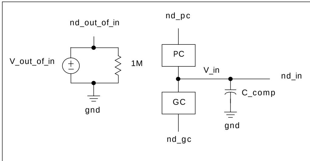
Figure 18-6: Input ECL Buffer
