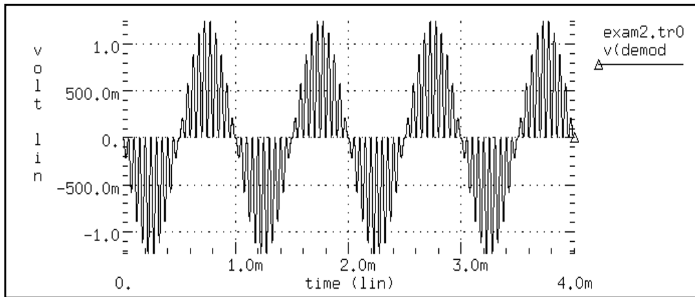
Figure 26-8: Demodulated Signal
