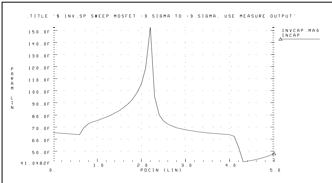
Figure 22-5: Graph of Pin Capacitance versus Inverter Input Voltage
