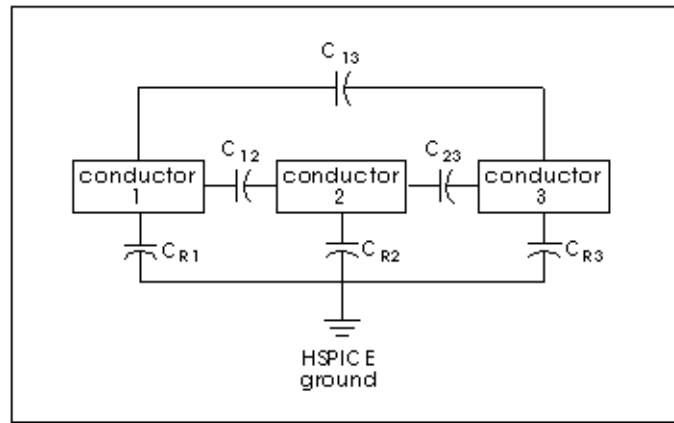
Figure B-34: Conductor Capacitances for Example 2
