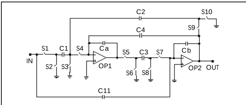
Figure 27-21: High_Q Biquad Section
