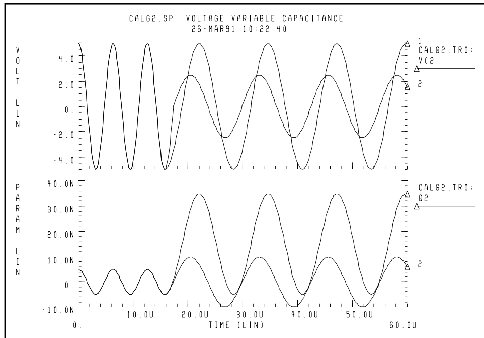
Figure 24-31: Incorrect Result Corresponding to CTYPE=0
