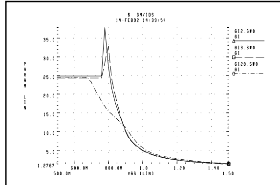
Figure 20-41: Levels 2, 3, 28 gm/Ids vs. Vgs Curves
