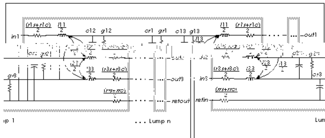
Figure B-29: Schematic for Three Coupled Lines with One Reference Plane
