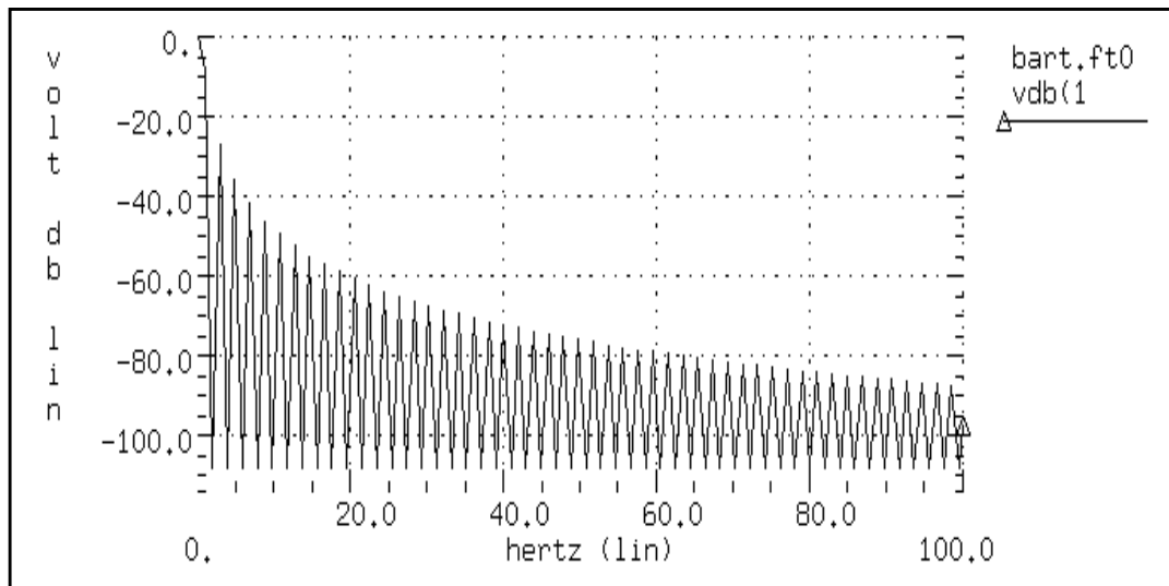
Figure 26-2: Bartlett Window Characteristics
