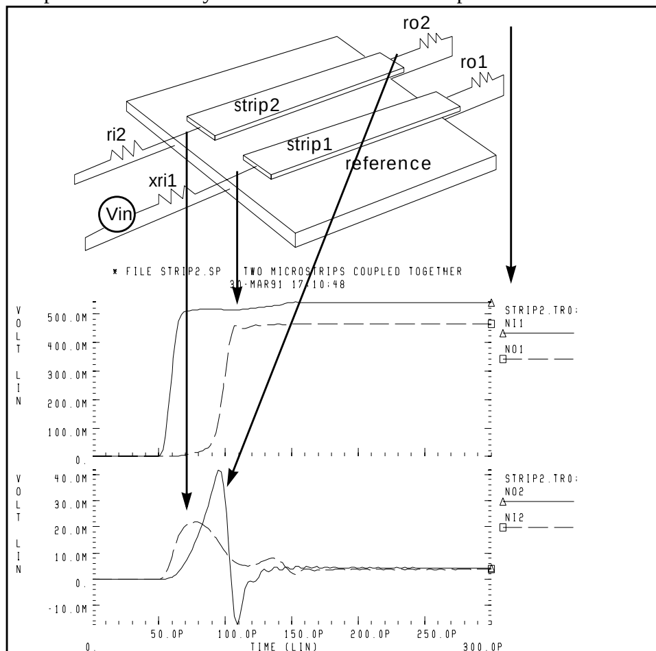
Figure B-38: Two Coupled Microstrips Geometrically Defined as LSI Metallization
