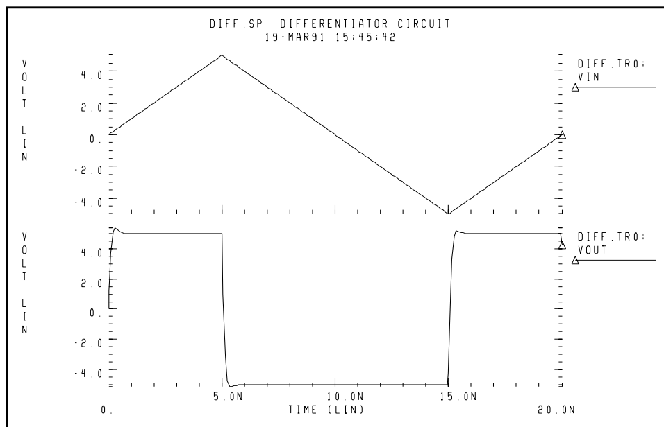
Figure 24-17: Response Of a Differentiator to a Triangle Waveform
