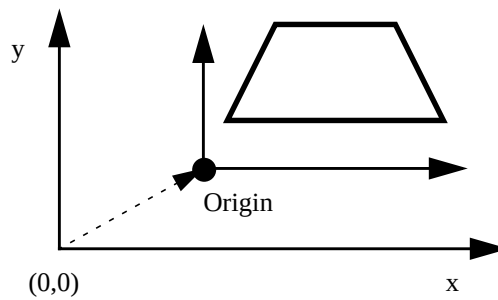
Figure 17-12: Coordinates of a Polygon
