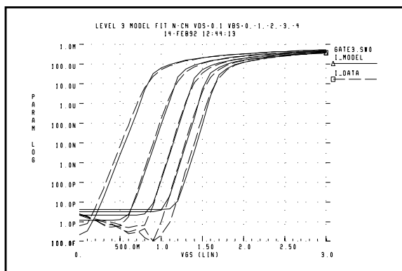
Figure 20-27: Level 3 Ids vs. Vgs Curves
