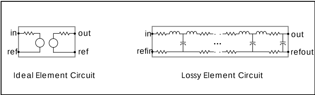
Figure B-3: Ideal versus Lossy Transmission Line Model
