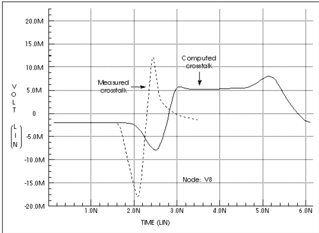
Figure B-26: Measured Versus Computed Forward Crosstalk Response
