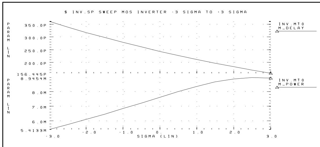
Figure 12-14: Sweep MOS Inverter, Pair Delay and Power: -3 Sigma to 3 Sigma
