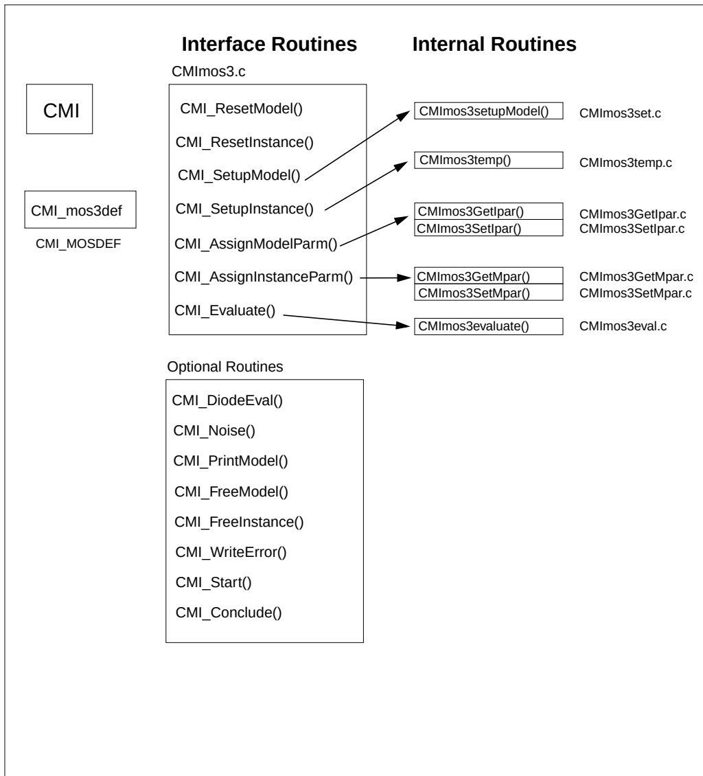
Figure 21-2: Hierarchy of Interface and Internal Routines
