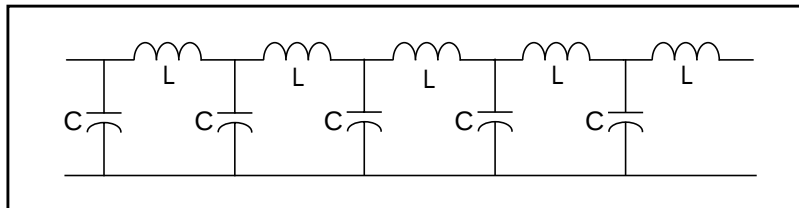
Figure B-44: Equivalent Circuit Model of a Lossless Transmission Line
