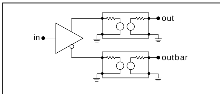
Figure B-6: Use of Two T Elements for Full Signal and Reference
