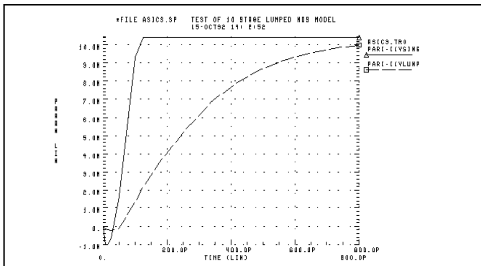
Figure 29-12: T2N2222 Optimization
