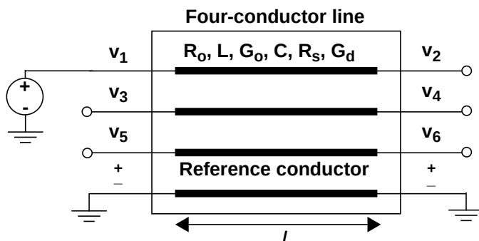
Figure 17-8: Four-conductor Line
