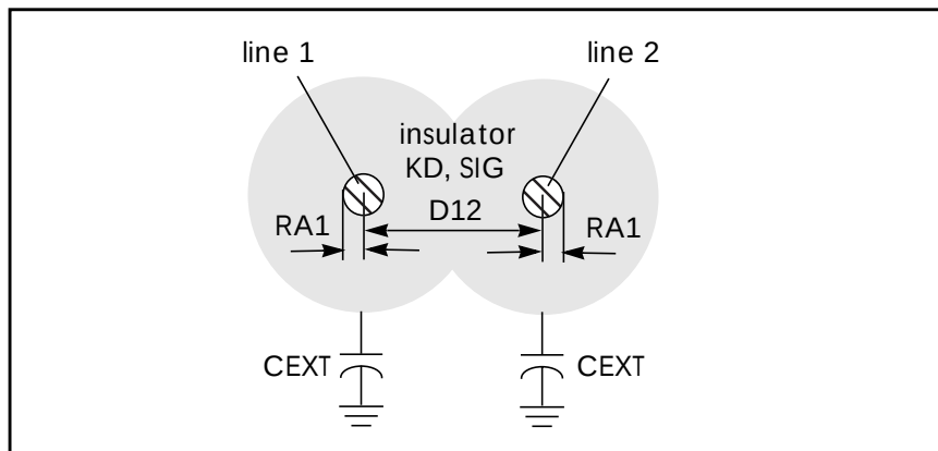
Figure B-16: Geometric Embedded Twinlead, DLEV=0, Sea of Dielectric
