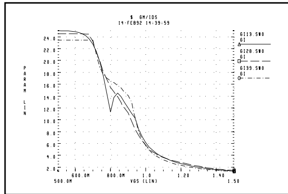
Figure 20-42: Levels 13, 28, 39 gm/lds vs. Vgs Curves
