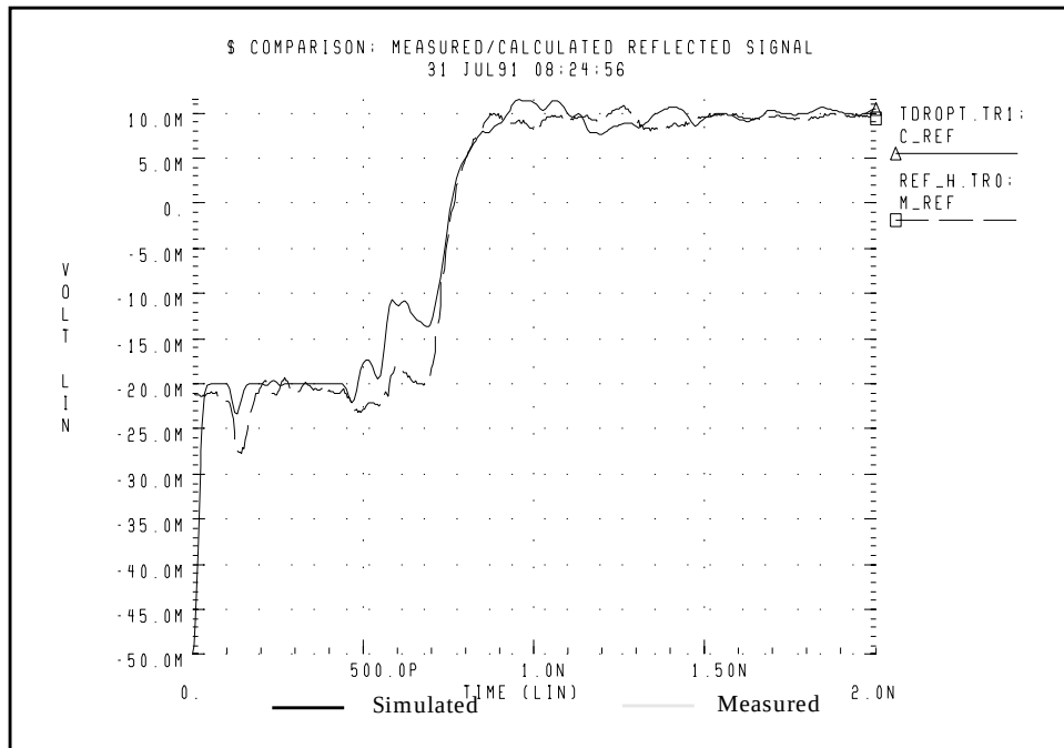
Figure 23-7: Reflected Signals After Optimization
