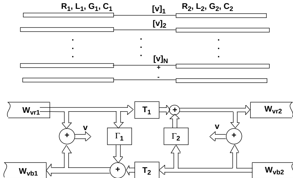
Figure 17-3: System Model for a Line-to-Line Junction
