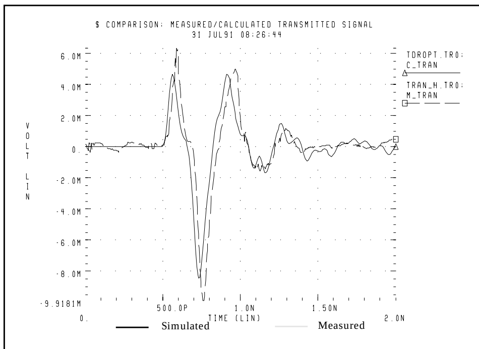
Figure 23-8: Transmitted Signals Before Optimization
