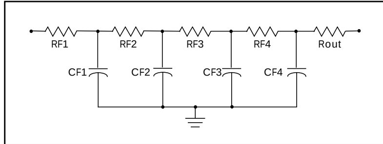
Figure B-39: Circuit Diagram of an RC Filter
