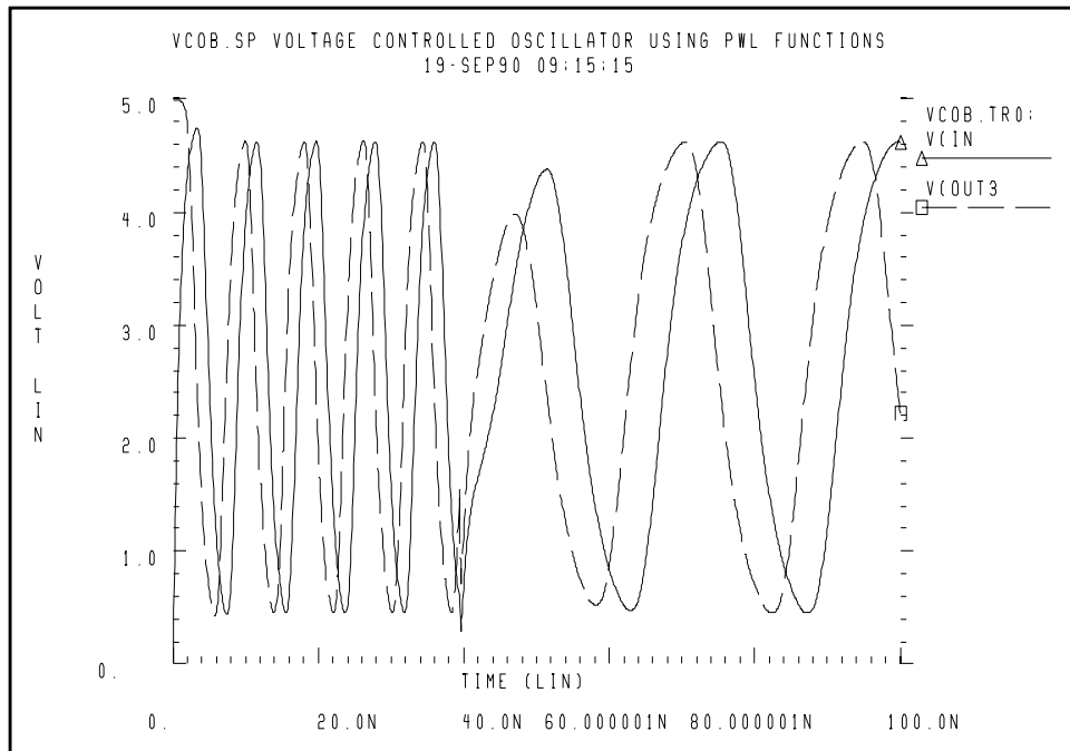
Figure 24-29: Voltage Controlled Oscillator Response
