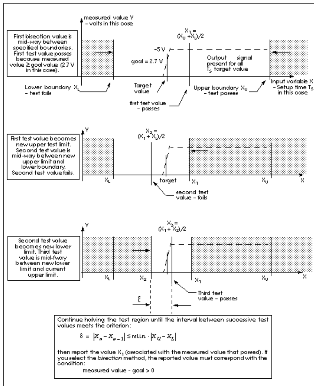
Figure 28-2: Bisection Example for Three Iterations
