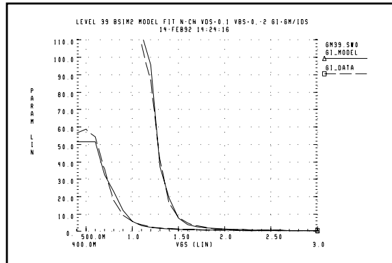
Figure 20-36: Level 39 gm/Ids vs. Vgs Curves
