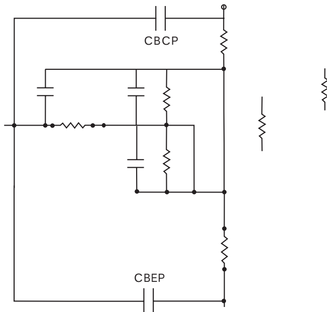
Figure 15-7: Vertical Transistor, BJT AC Noise Analysis
