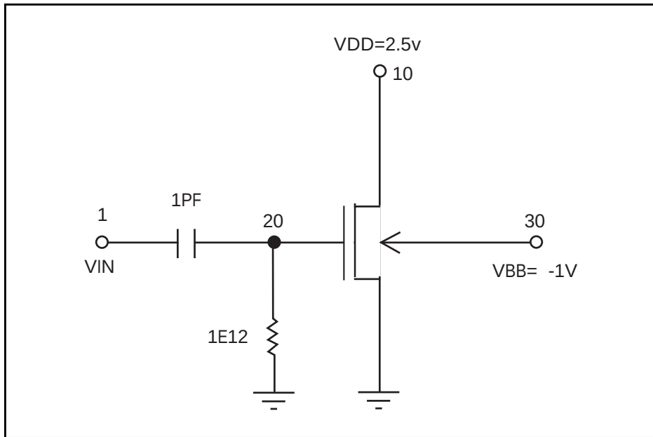
Figure 19-26: Charge Conservation Test Circuit
