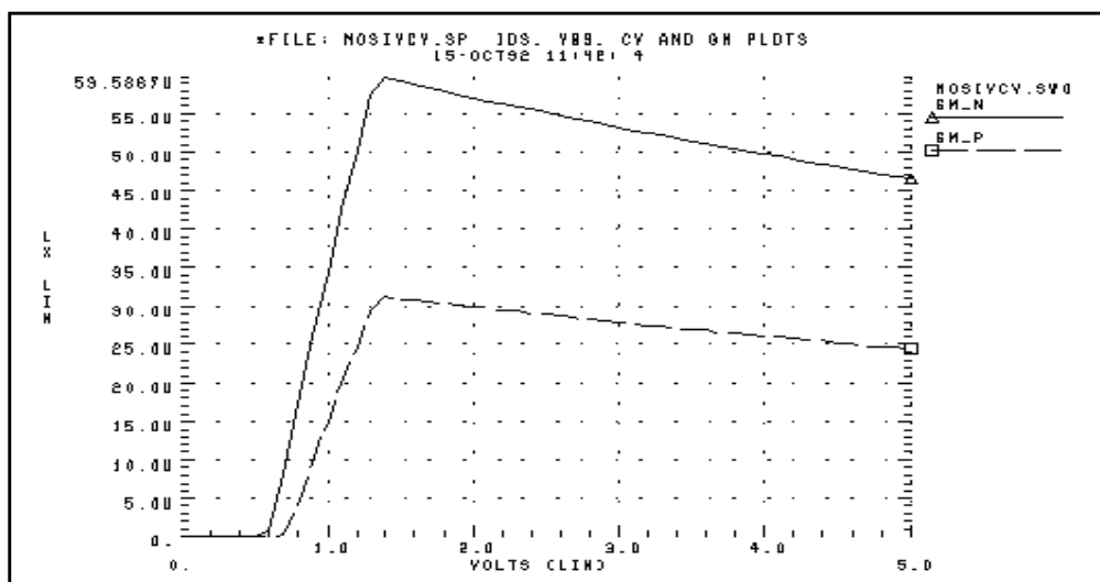
Figure 29-8: Noise Bounce
