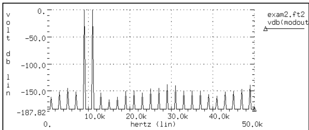
Figure 26-11: Modulated Signal Spectrum
