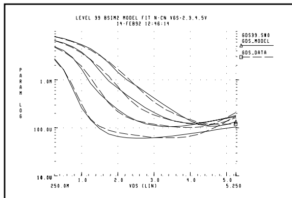
Figure 20-24: Level 39 gds vs. Vds Curves
