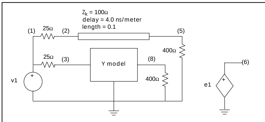
Figure 27-13: Line and Y-Parameter Modeling
