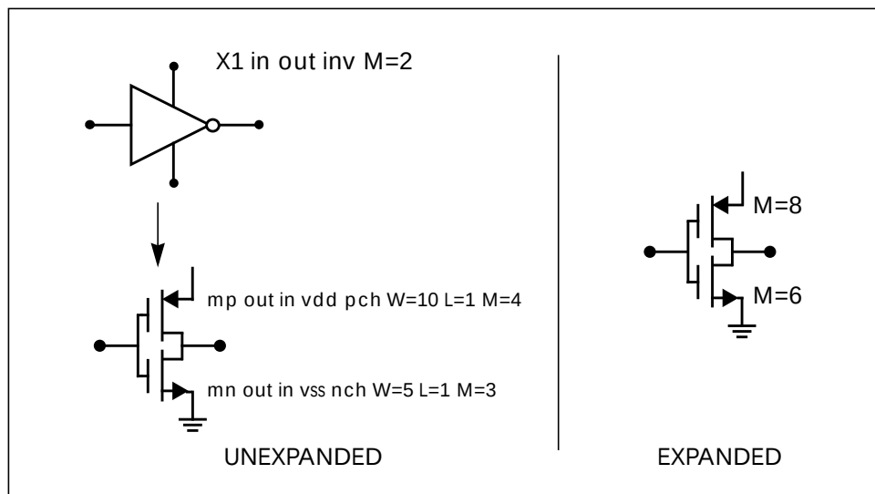
Figure 3-4: Hierarchical Parameters Simplify Flip-flop Initialization
