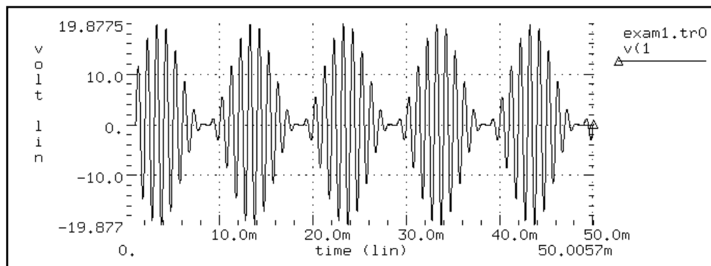
Figure 26-4: AM Modulation
