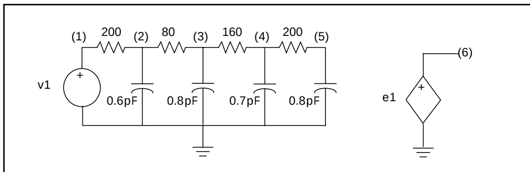
Figure 27-9: Circuits for an RC Line
