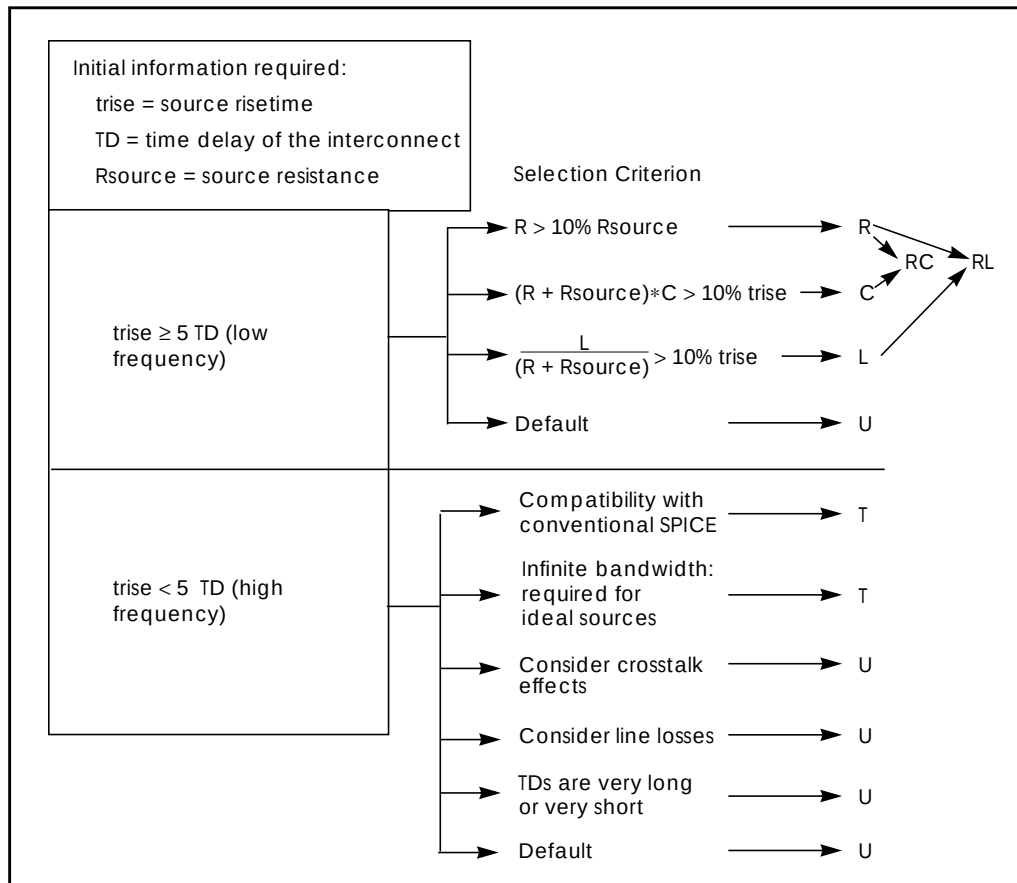
Figure B-1: Wire Model Selection Chart
