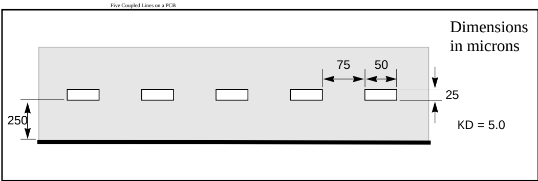
Figure B-36: Five Coupled Lines on a PCB
