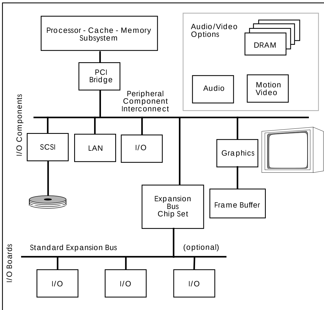
Figure 23-17: PCI System Block Diagram
