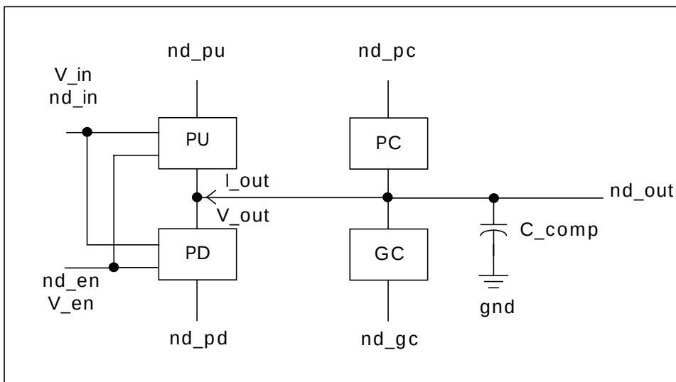
Figure 18-4: Tristate Buffer
