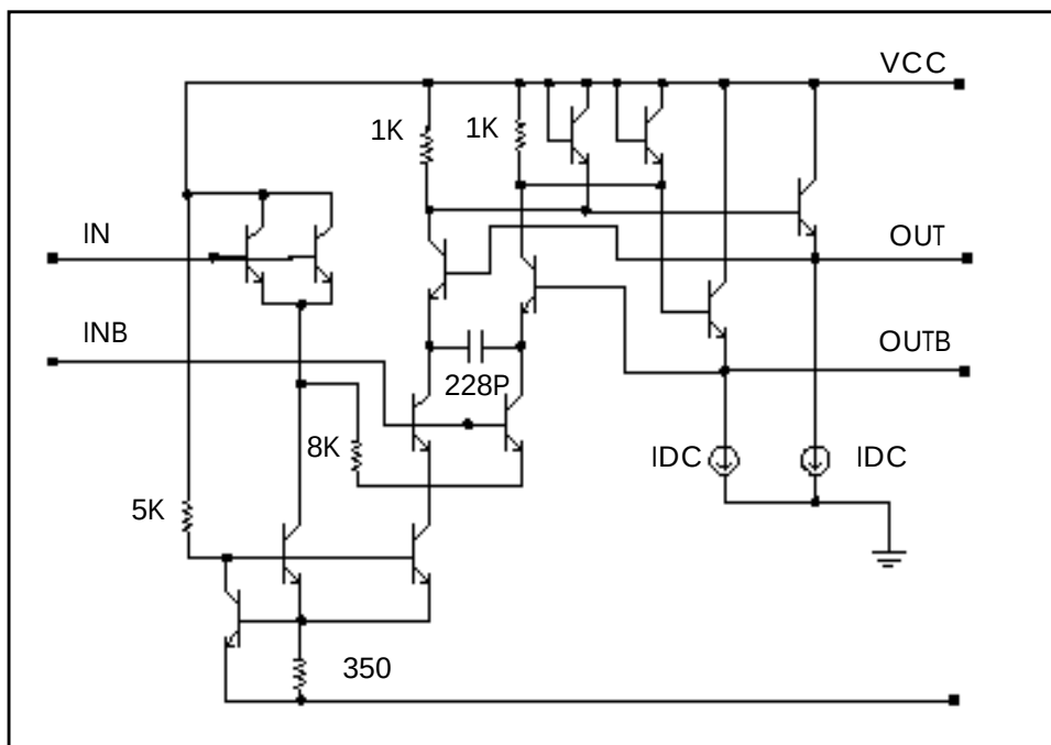
Figure 24-36: Voltage Controlled Oscillator Circuit
