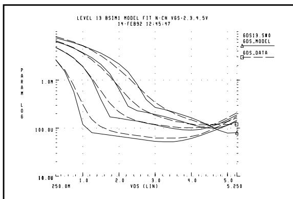
Figure 20-22: Level 13 gds vs. Vds Curves
