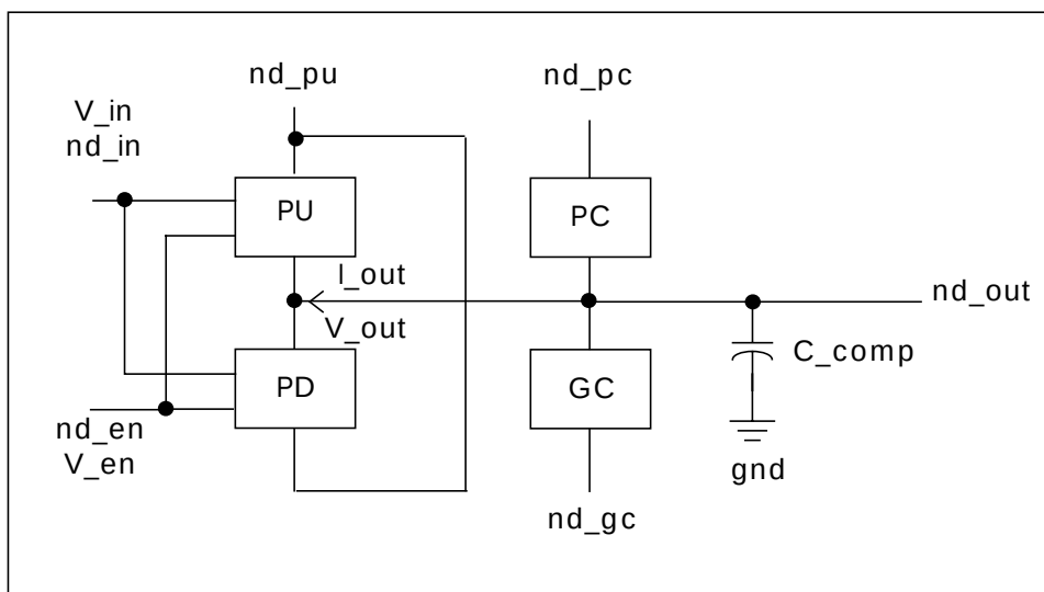
Figure 18-8: Tristate ECL Buffer
