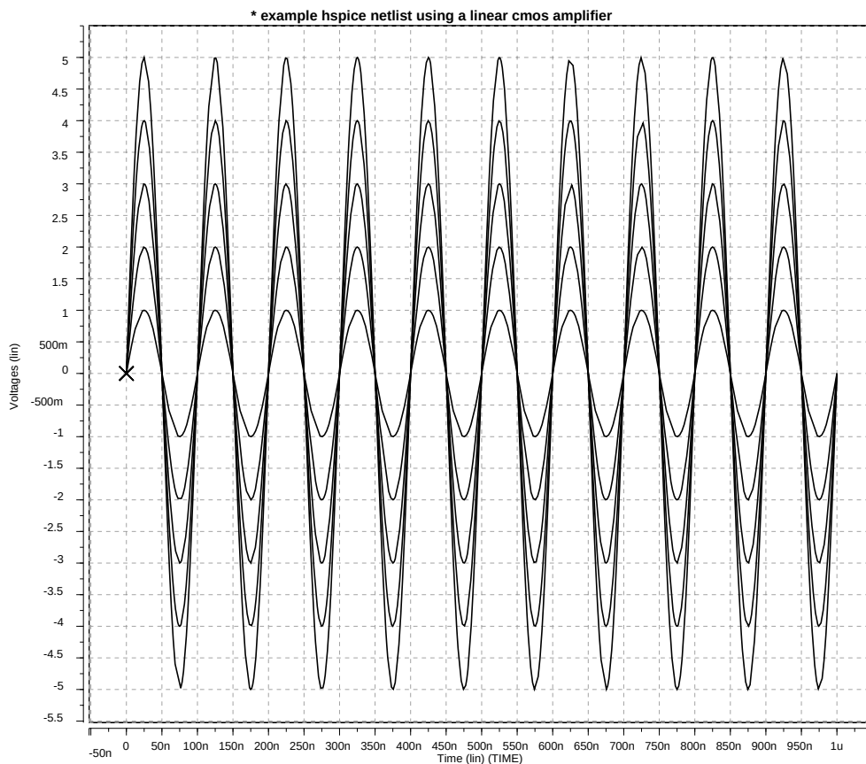
Figure E-2: Plot of Voltage on Node in
