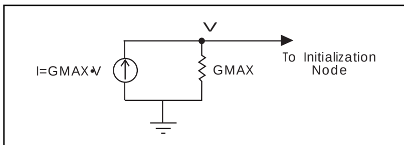
Figure 9-2: Equivalent Voltage Source: NODESET and .IC
