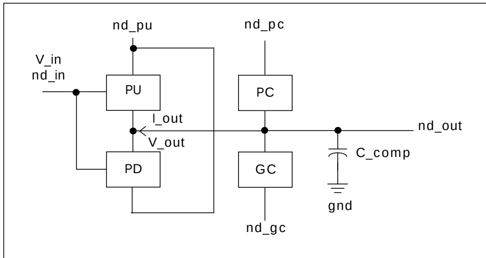
Figure 18-7: Output ECL Buffer
