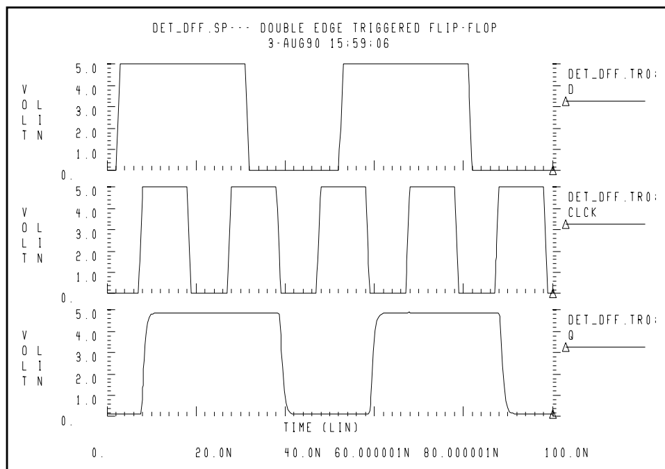
Figure 24-6: Double Edge Triggered Flip-Flop Response
