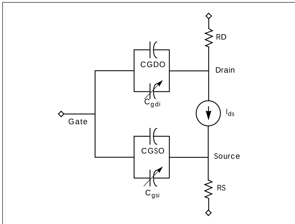
Figure 20-12: Level 40 HP a-Si TFT Topology
