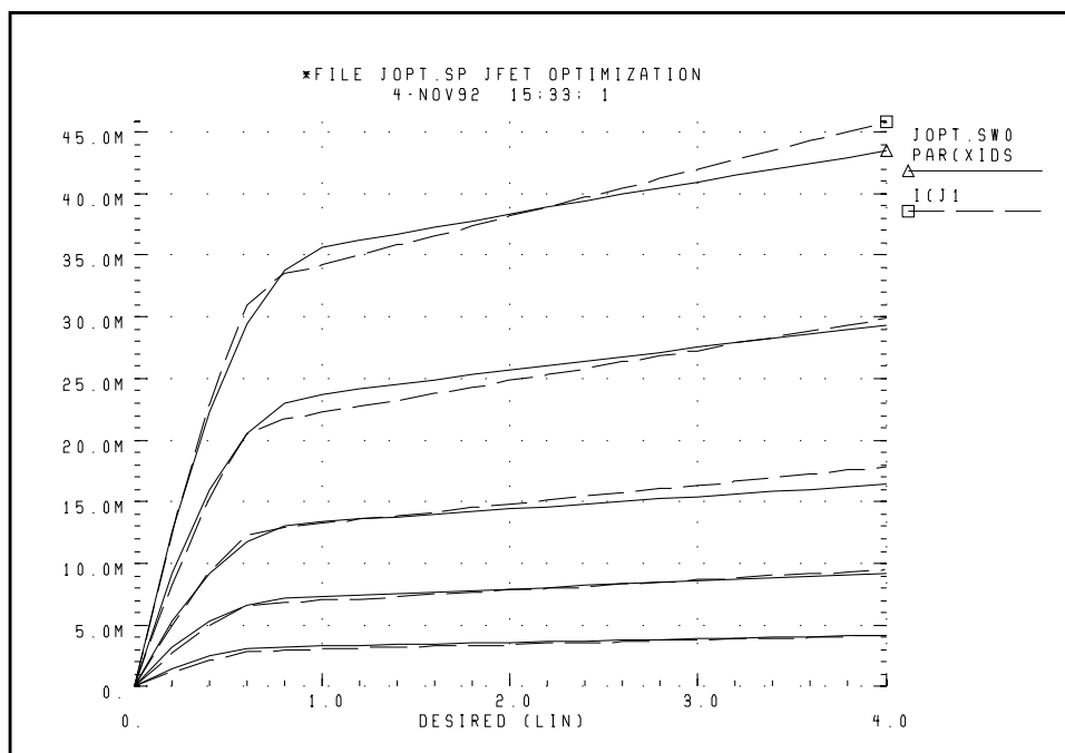
Figure 12-30: JFET Optimization
