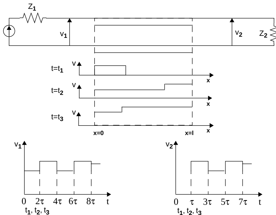
Figure 17-1: Propagation of a Voltage Step in a Transmission Line
