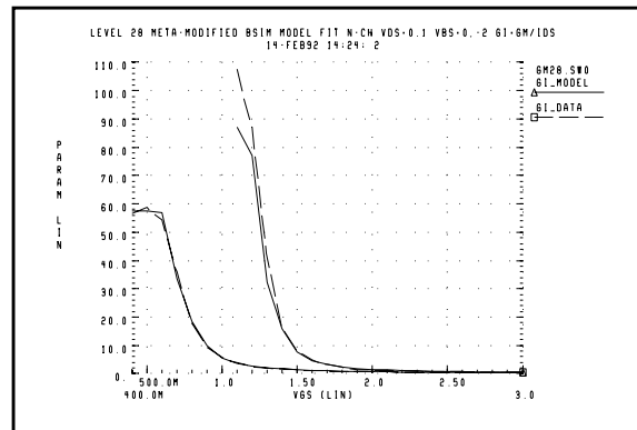
Figure 20-40: Level 28 gm/Ids vs. Vgs Curves
