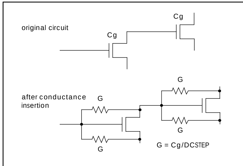
Figure 9-5: Conductance Insertion
