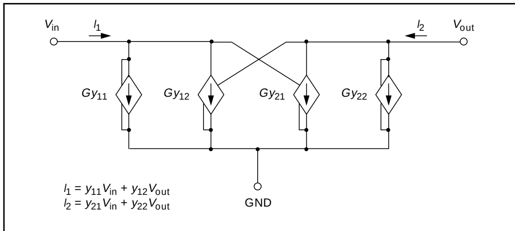
Figure 27-15: Schematic for the Y-Parameter Network
