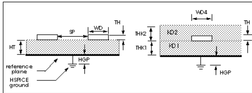
Figure B-9: U Element Conductor Dimensions
