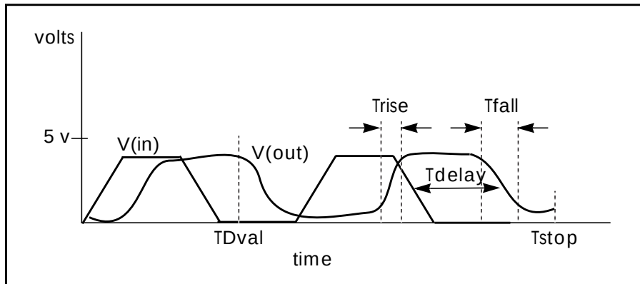
Figure 22-1: Rise, Fall, and Delay Time Demonstration
