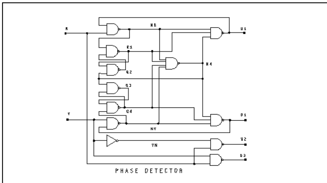
Figure 24-32: Circuit Schematic of Phase Detector
