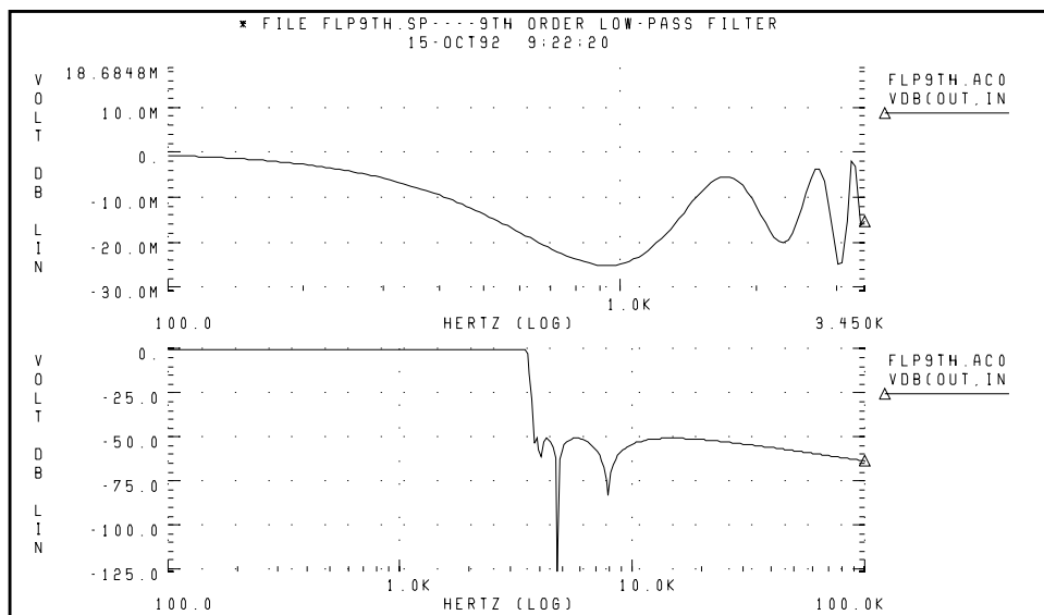
Figure 25-10: 9th Order Low-Pass Filter Response
