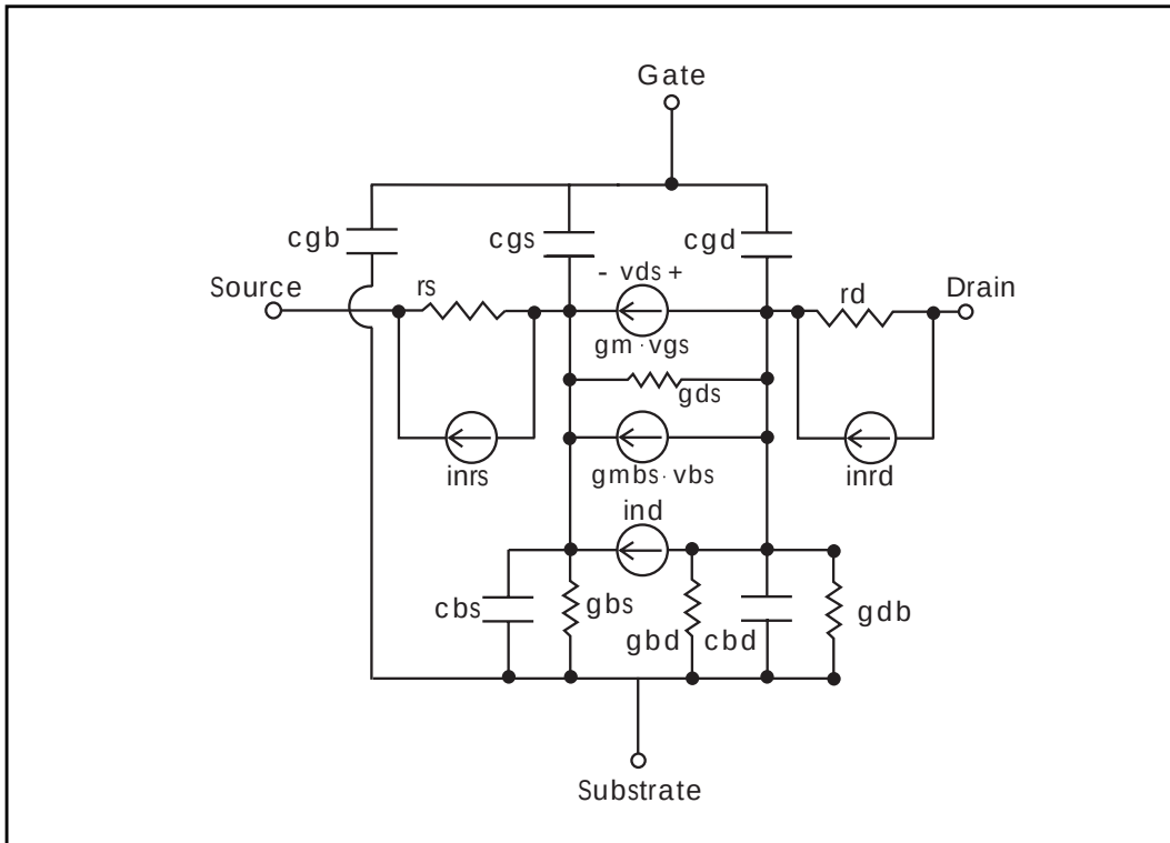
Figure 19-10: Equivalent Circuit, MOSFET AC Noise Analysis
