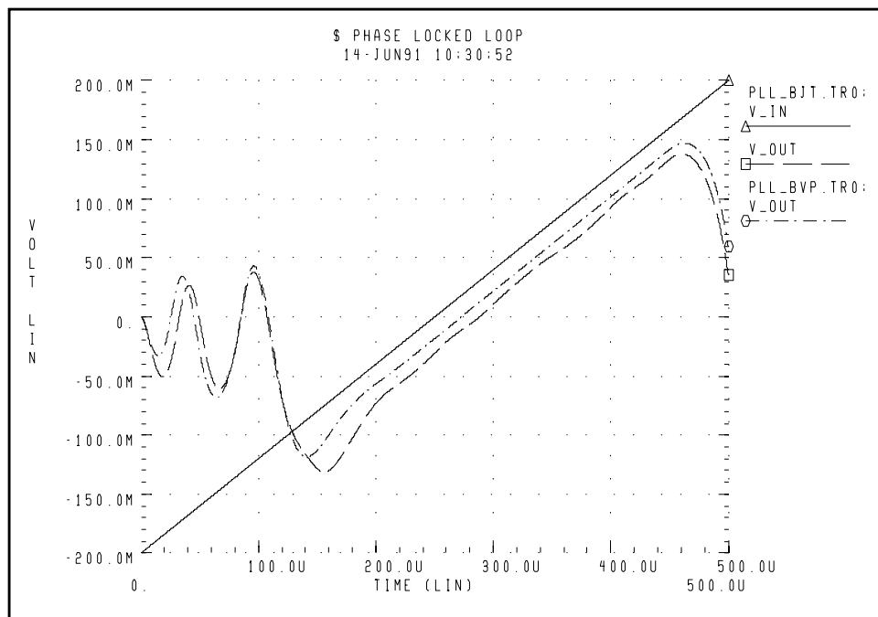
Figure 24-35: Behavioral (PLL_BVP Curve) vs. Bipolar (PLL_BJT Curve) Circuit Simulation
