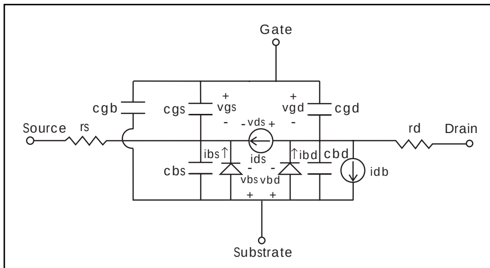
Figure 19-8: Equivalent Circuit, MOSFET Transient Analysis
