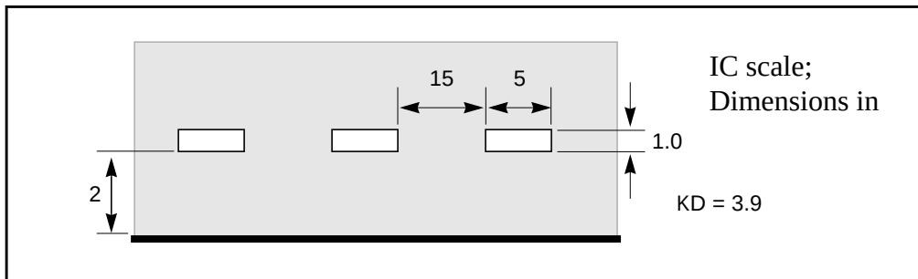
Figure B-28: Three Coupled Lines with One Reference Plane in a Sea of Dielectric (IC Scale)
