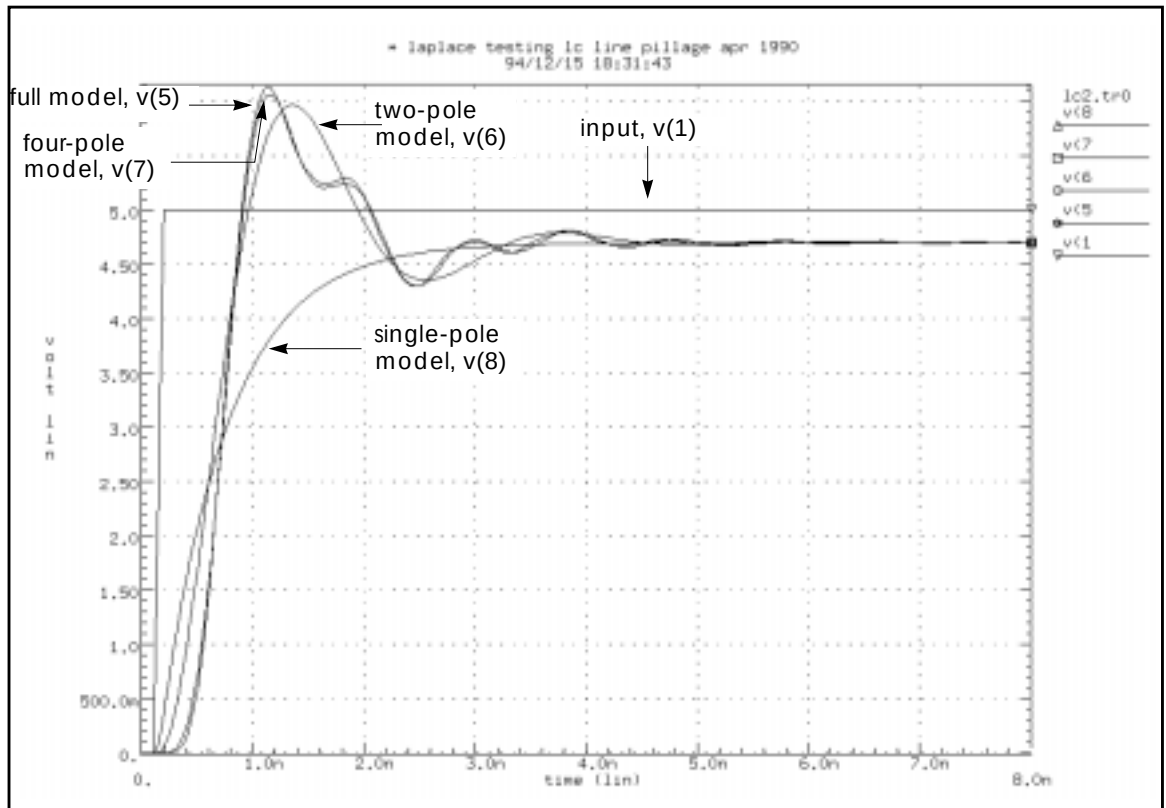
Figure 27-12: Transient Response of the Low-Loss Line
