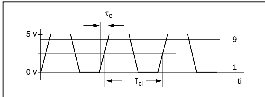
Figure B-46: Clock Waveform
