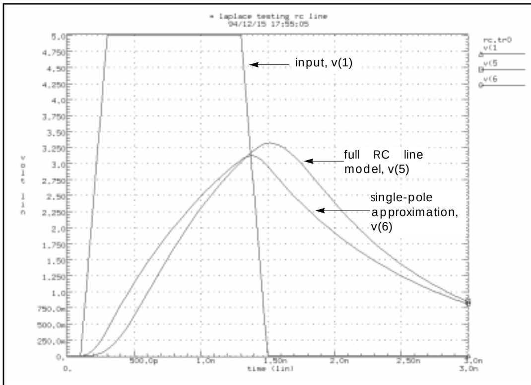
Figure 27-10: Transient Response of the RC Line and Single-Pole Approximation
