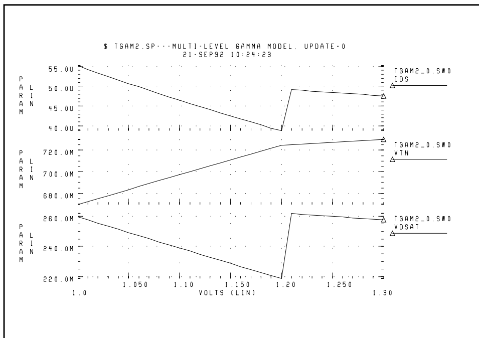
Figure 20-2: Variation of IDS, VTH and VDSAT for UPDATE=0
