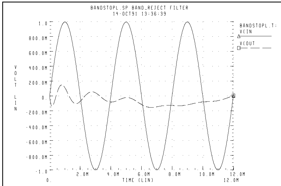
Figure 27-3: Transient Response of the Band-Reject Filter to a 250 Hz Sine Wave
