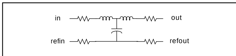
Figure B-7: Lossy Line with Reference Plane
