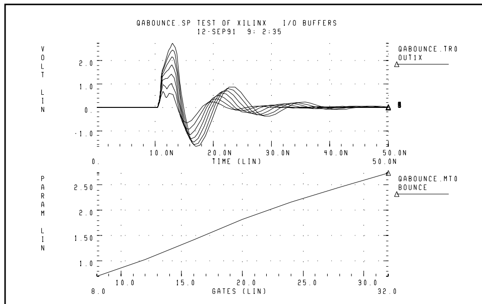
Figure 23-14: Results of Ground Bounce Simulation
