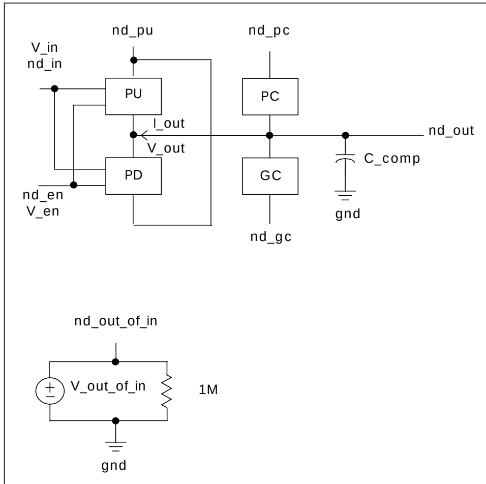
Figure 18-9: Input-Output ECL Buffer
