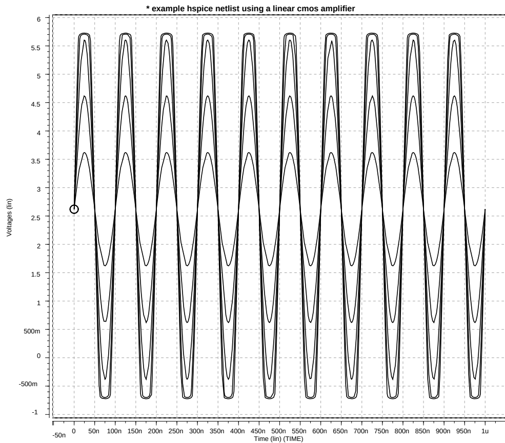
Figure E-3: Plot of Voltage on Node clamp vs. Time
