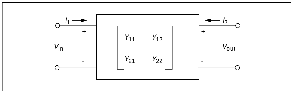
Figure 27-14: Y Matrix for the Two-Port Network
