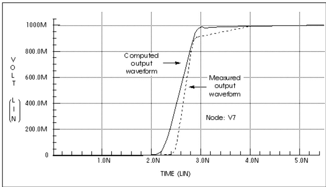
Figure B-24: Measured versus Computed Through-Line Response
