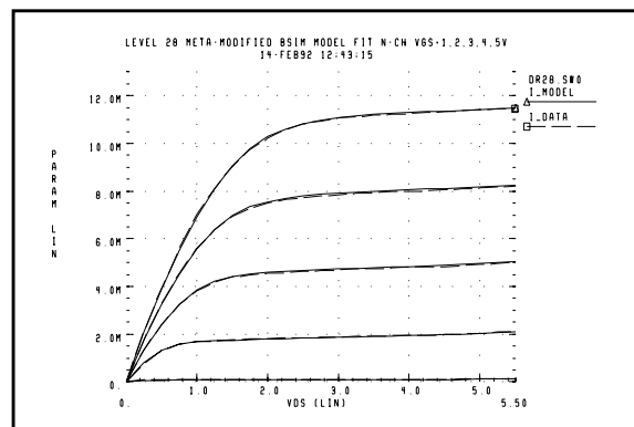
Figure 20-17: Level 28 Ids vs. Vds Curves
