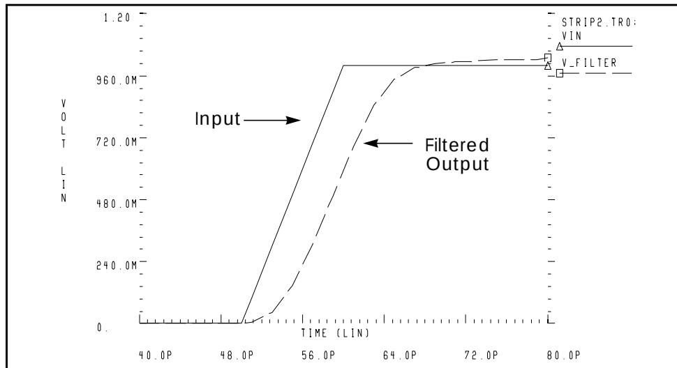
Figure B-40: Multistage RC Filter Input and Output
