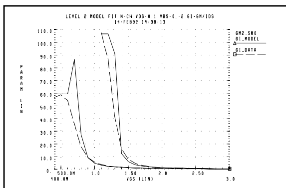
Figure 20-31: Level 2 gm/Ids vs. Vgs Curves
