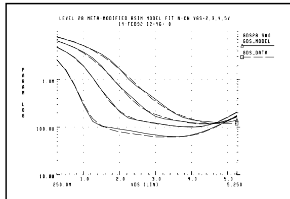
Figure 20-20: Level 28 gds vs. Vds Curves
