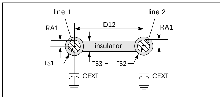
Figure B-17: Geometric Twinlead, DLEV=1, with Insulating Spacer
