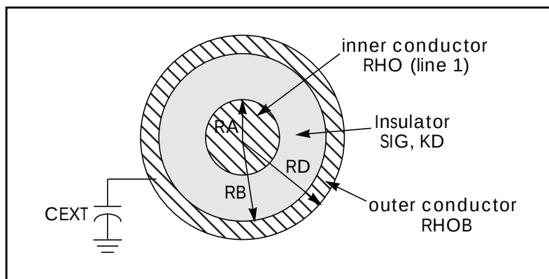
Figure B-15: Geometric Coaxial Cable
