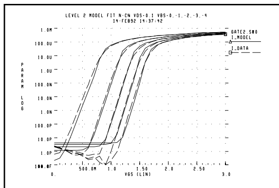
Figure 20-25: Level 2 Ids vs. Vgs Curves
