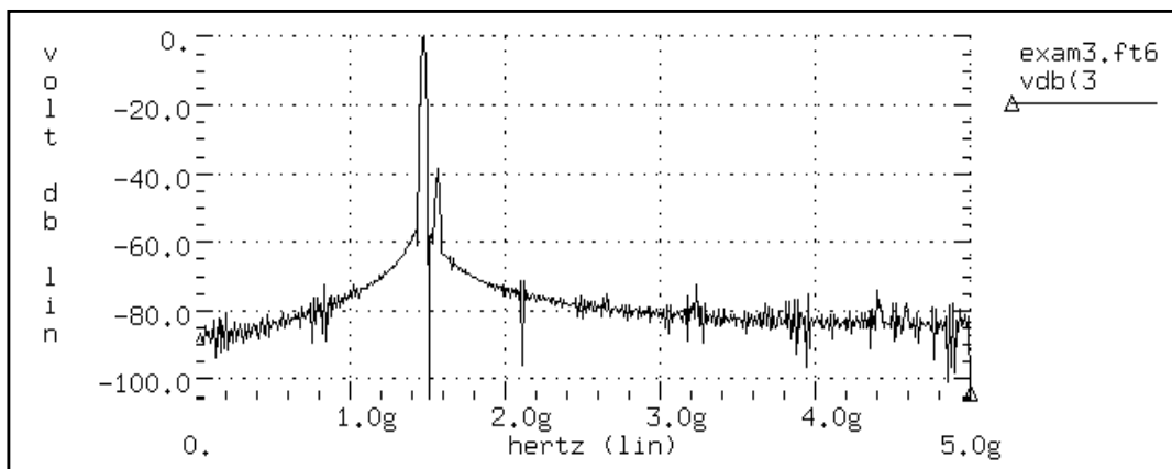
Figure 26-21: Mixer Output Spectrum, Gaussian Window
