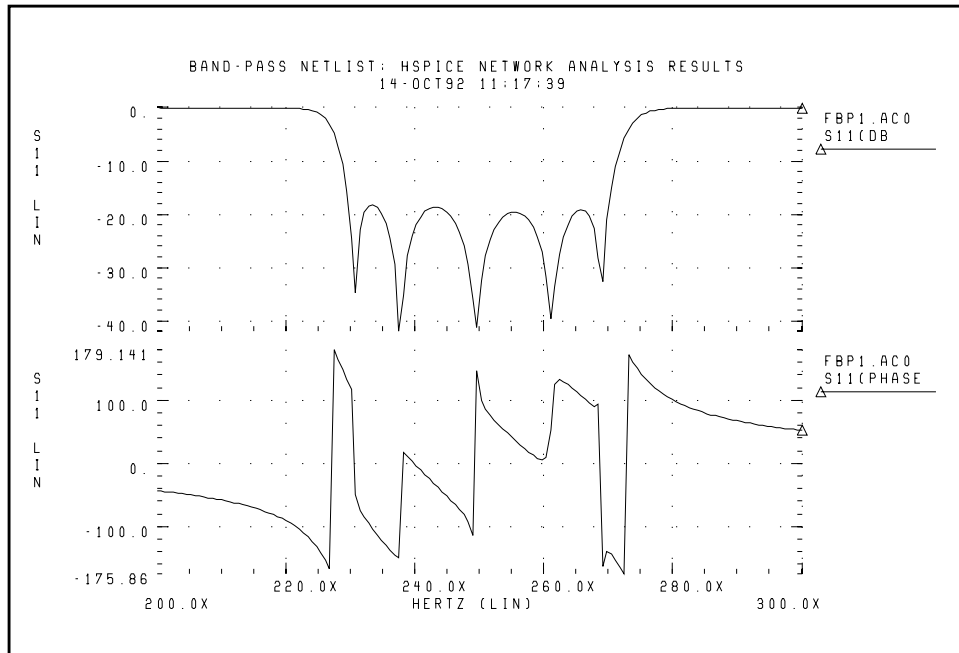
Figure 11-2: S11 Magnitude and Phase Plots
