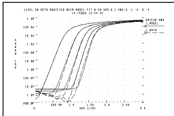
Figure 20-29: Level 28 Ids vs. Vgs Curves
