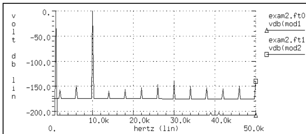
Figure 26-10: Modulating and Modulated Signal Spectrum
