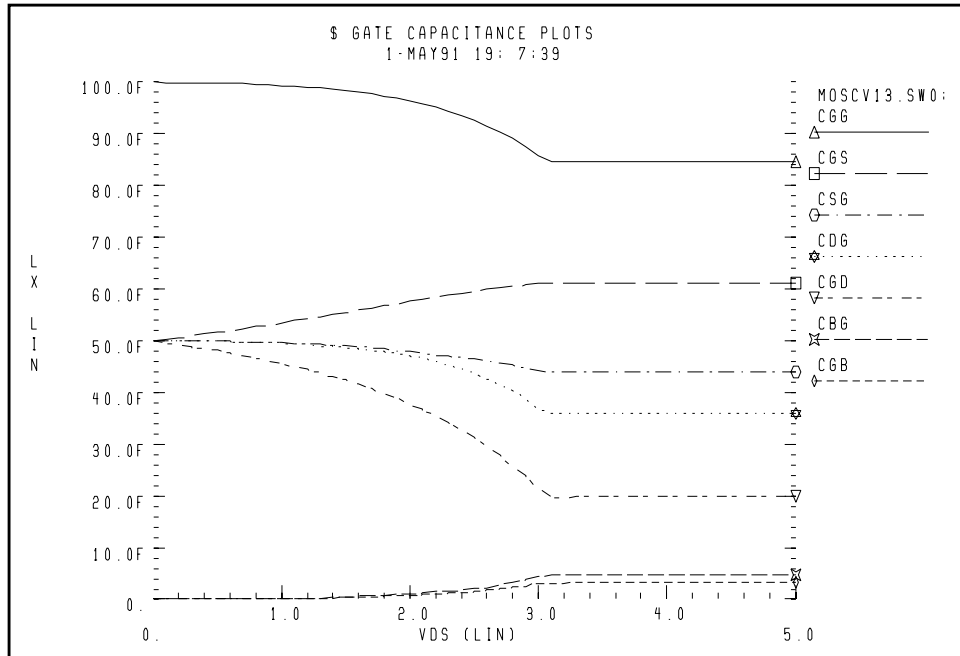
Figure 19-18: Gate Capacitance
