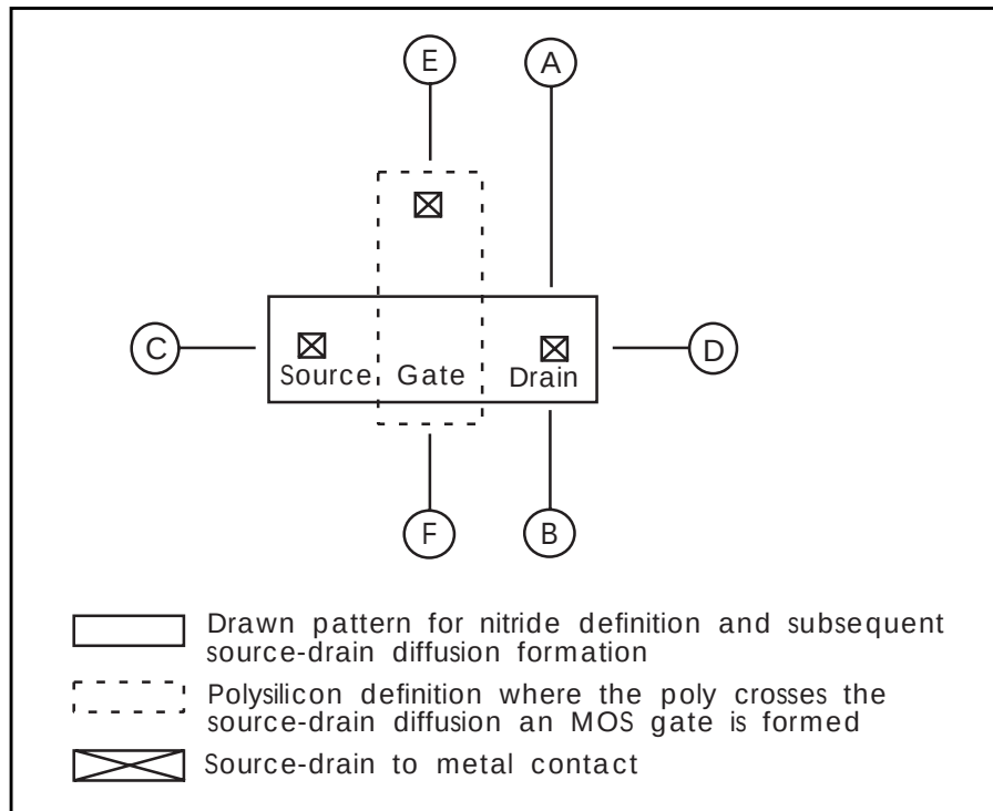
Figure 19-3: Isoplanar Silicon Gate Transistor
