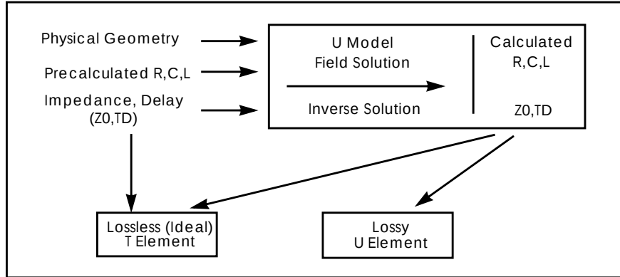
Figure B-2: U Model, T Element and U Element Relationship
