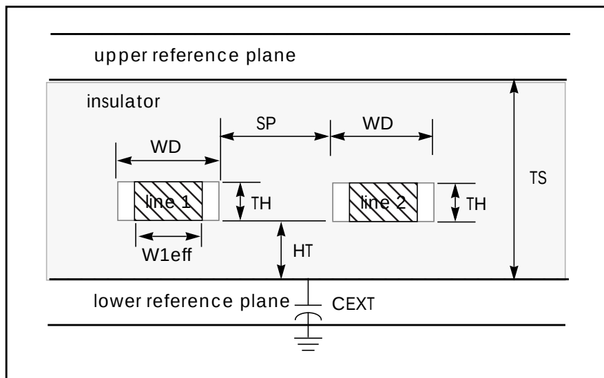
Figure B-13: Planar Transmission Line, DLEV=2, Stripline
