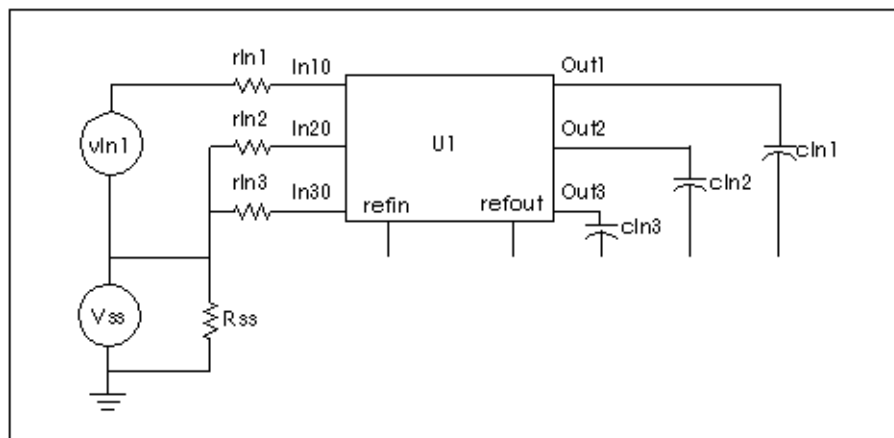
Figure B-30: Schematic Using the Three Coupled Lines U Model
