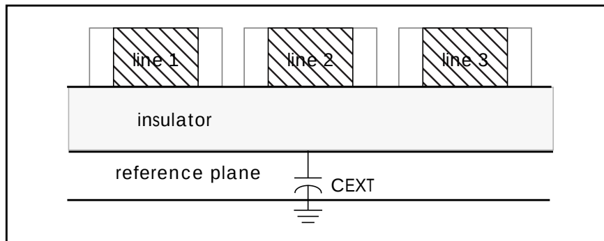
Figure B-12: Planar Transmission Line, DLEV=1, Microstrip
