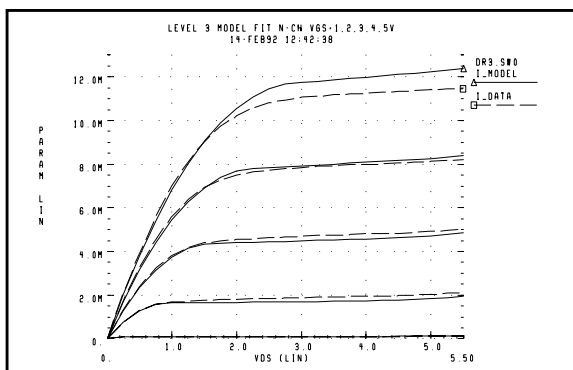
Figure 20-15: Level 3 Ids Model vs. Data Curves
