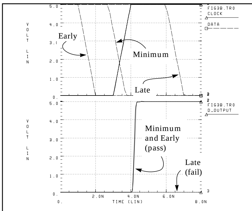
Figure 28-4: Early, Minimum, and Late Setup and Hold Times
