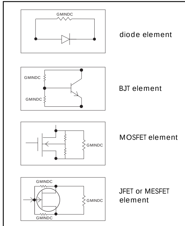
Figure 9-4: GMINDC Insertion
