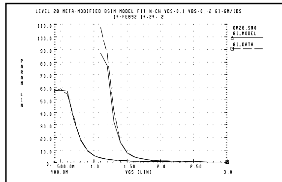
Figure 20-32: Level 28 gm/Ids vs. Vgs Curves
