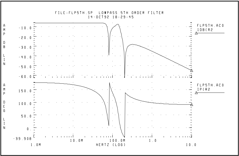
Figure 25-2: Fifth-Order Low-Pass Filter Response
