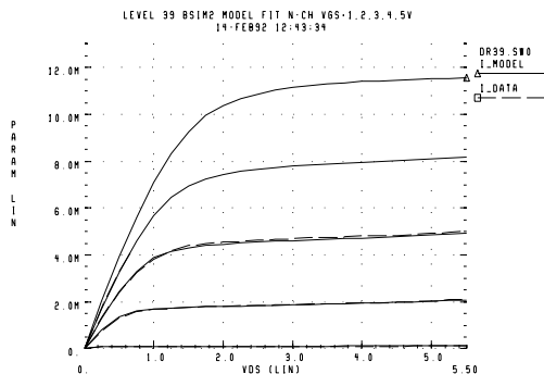
Figure 20-18: Level 39 Ids vs. Vds Curves
