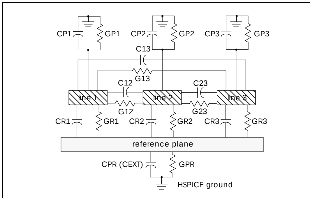
Figure B-21: Single-Lump Circuit Capacitance
