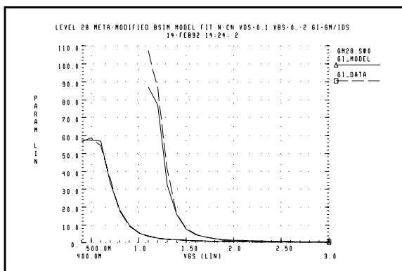
Figure 20-35: Level 28 gm/Ids vs. Vgs Curves
