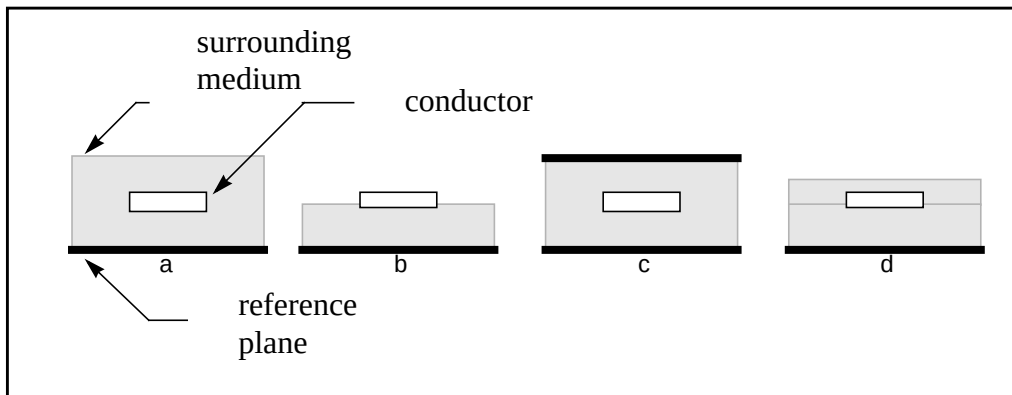
Figure B-8: Dielectric and Reference Plane Configurations
