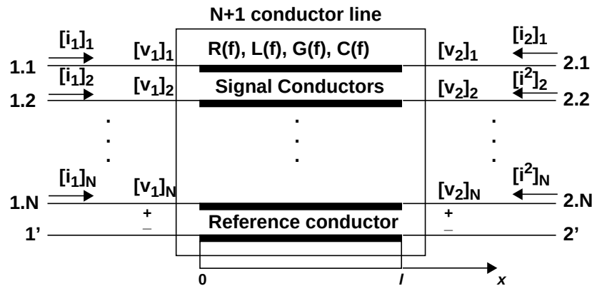
Figure 17-6: Terminal Node Numbering
