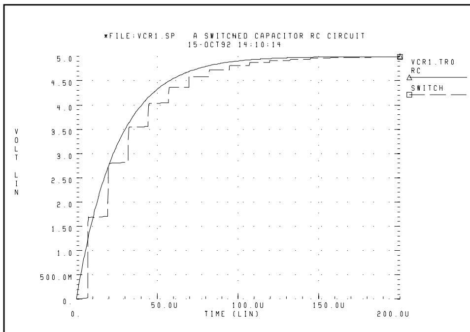
Figure 27-19: VCR1.SP Switched Capacitor RC Circuit
