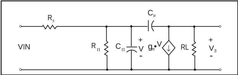
Figure 25-6: Simple Amplifier
