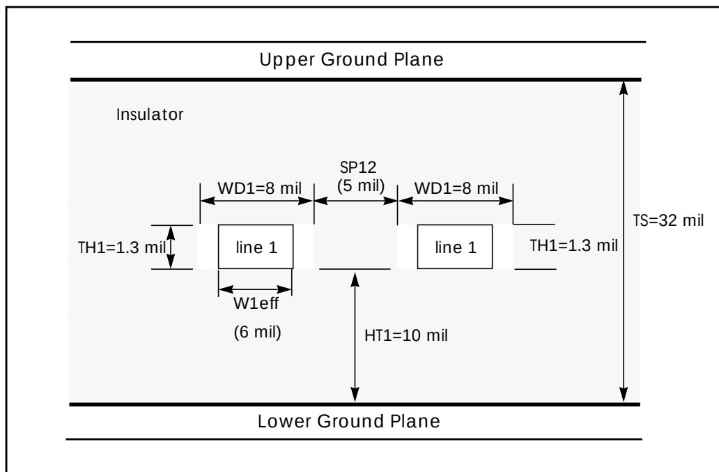
Figure 23-10: Planar Transmission Line DLEV=2: Microstrip Sea of Dielectric
