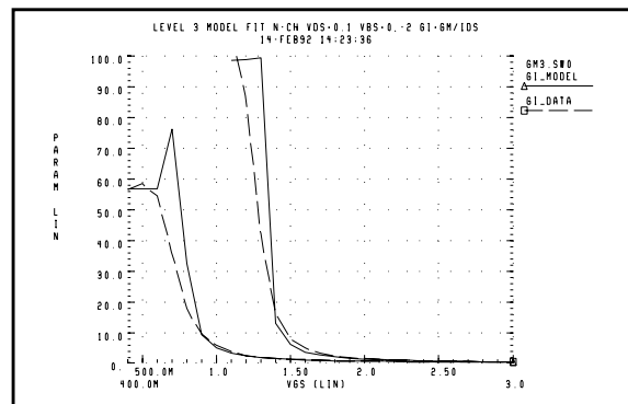
Figure 20-33: Level 3 gm/Ids vs. Vgs Curves
