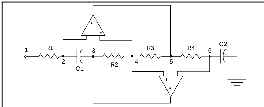
Figure 25-8: The FDNR Subcircuit
