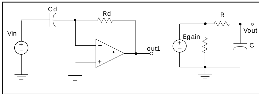
Figure 24-16: Differentiator Circuit
