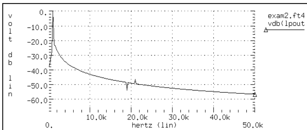
Figure 26-13: Filtered Output Signal (no window)
