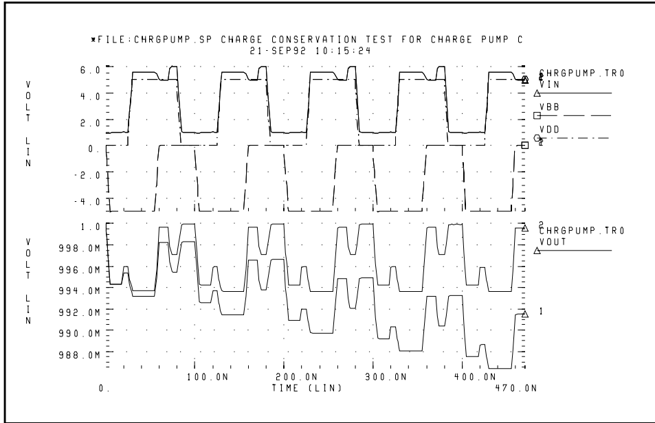
Figure 19-25: Charge Conservation Test: CAPOP=2 or 9
