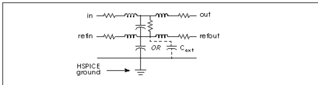
Figure B-10: Schematic of a U Element Lump when LLEV=1
