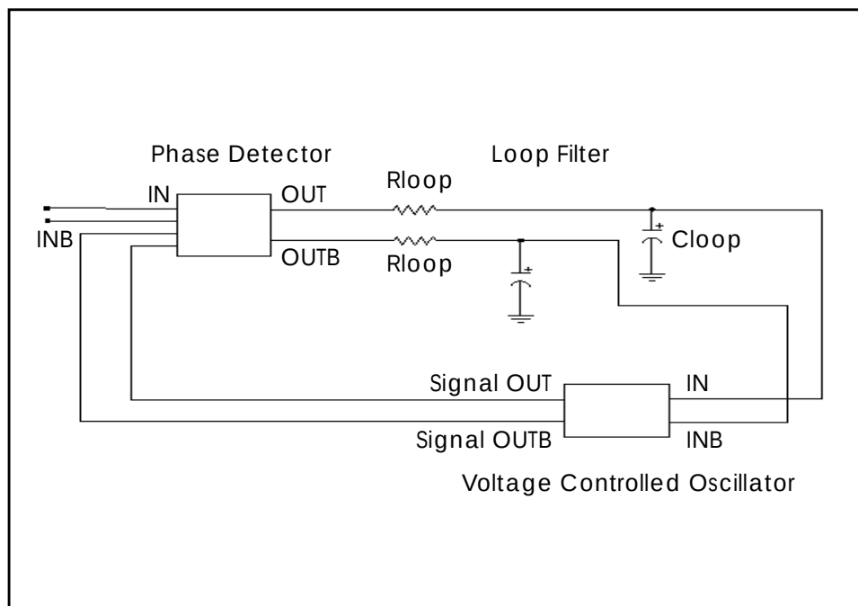
Figure 24-34: PLL Schematic
