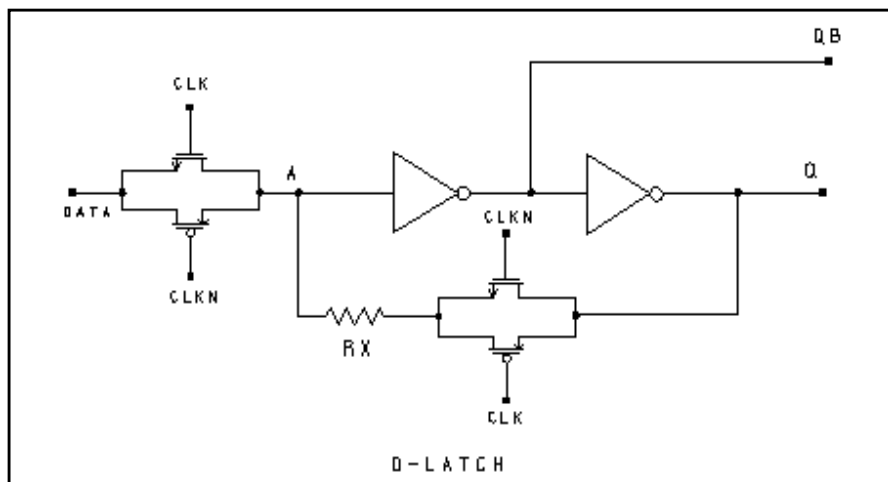
Figure 24-3: D-Latch Circuit
