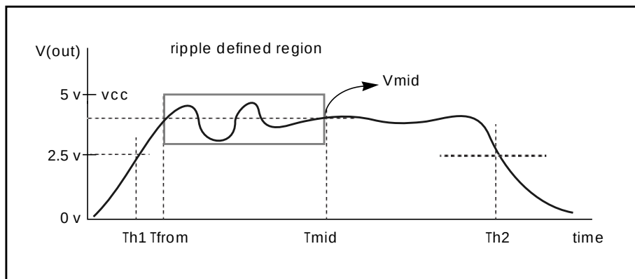
Figure 22-2: Waveform to Demonstrate Ripple Calculation
