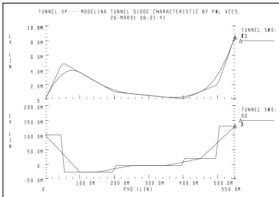
Figure 24-19: Tunnel Diode Characteristic
