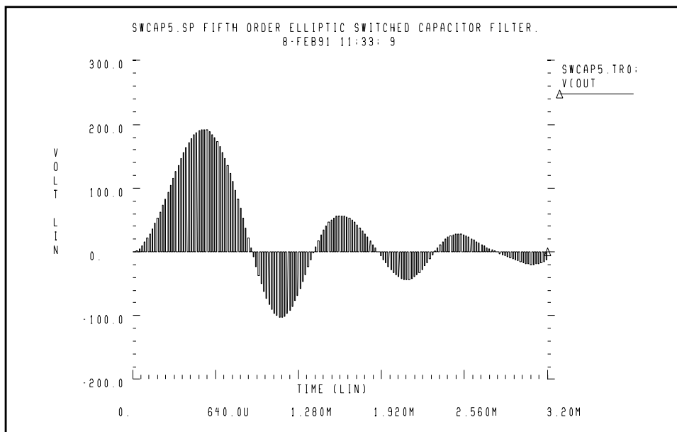
Figure 27-24: Response to 2-kHz Sinusoidal Input
