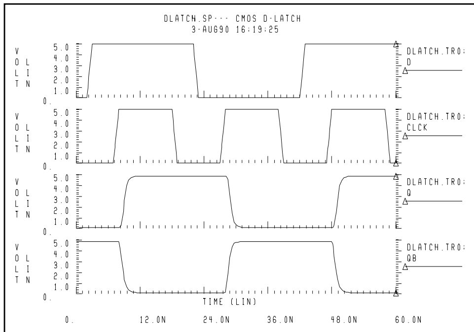
Figure 24-4: D-Latch Response
