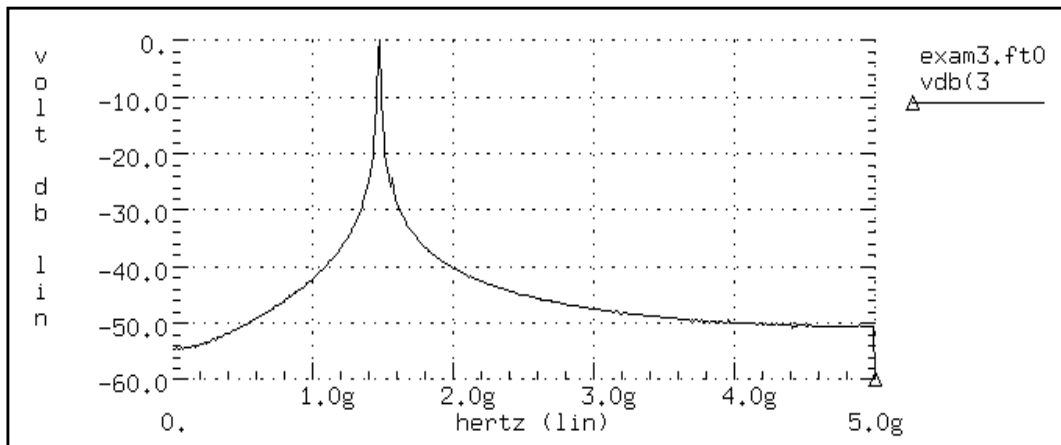
Figure 26-15: Mixer Output Spectrum, Rectangular Window
