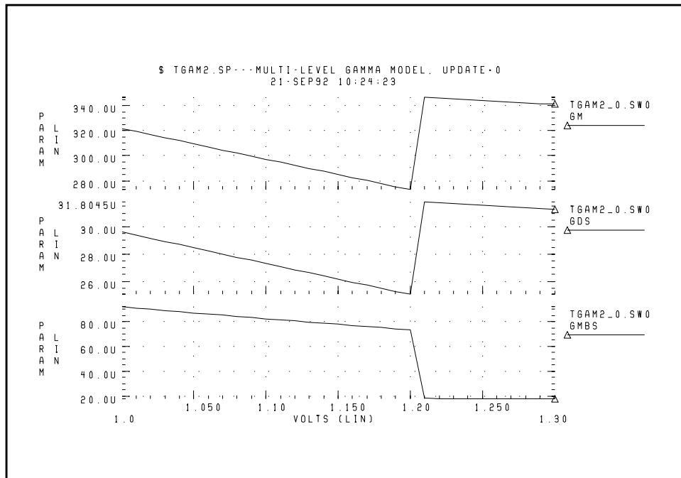
Figure 20-3: Variation of GM, GDS and GMBS for UPDATE=0
