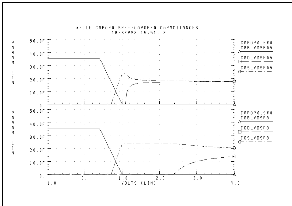
Figure 19-19: CAPOP=0 Capacitances
