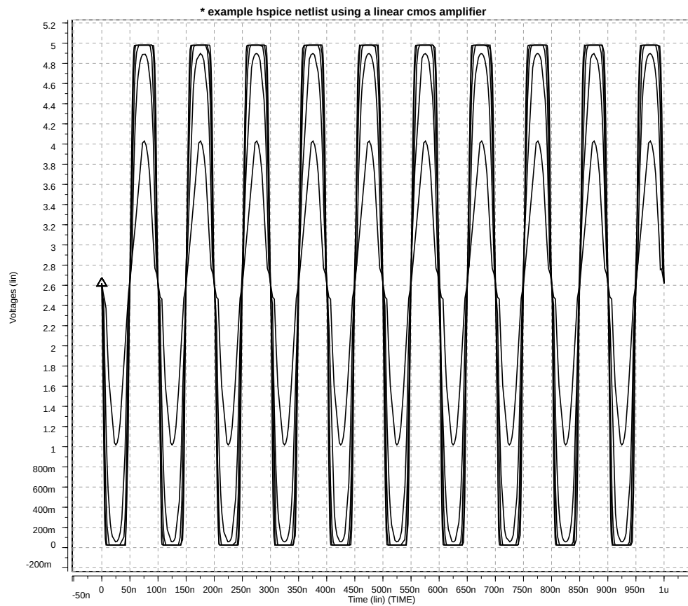
Figure E-4: Plot of Voltage on Node inv1out vs.Time
