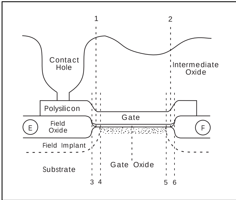
Figure 19-6: Isoplanar MOSFET, Width Cut
