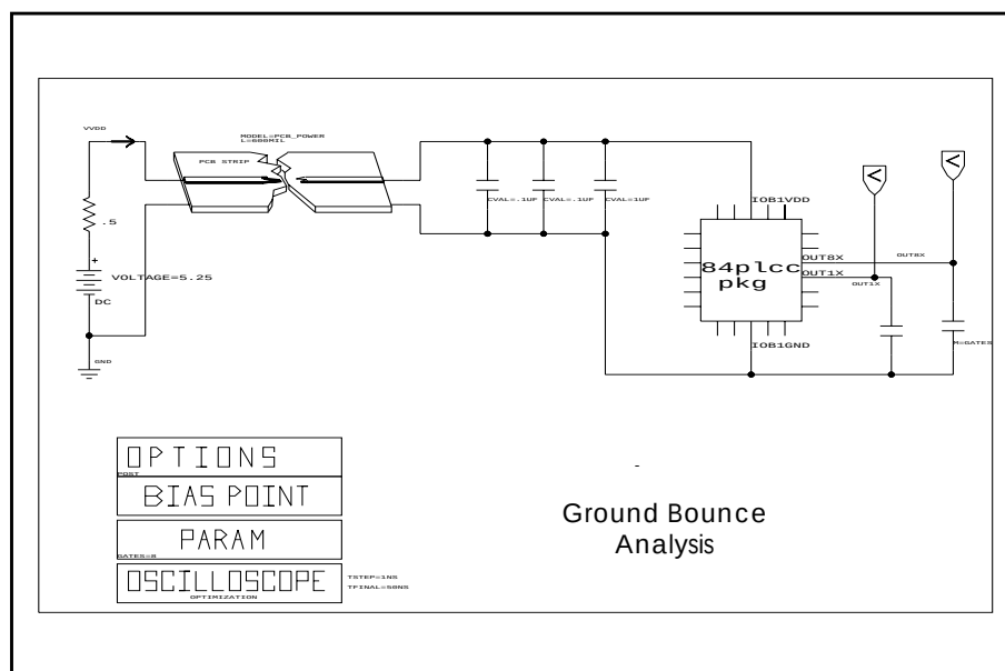
Figure 23-13: Ground Bounce Simulation
