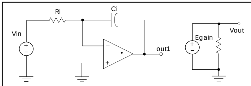
Figure 24-14: Integrator Circuit
