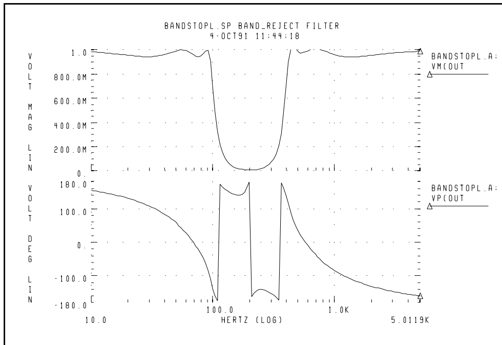
Figure 27-2: Frequency Response of the Band-Reject Filter
