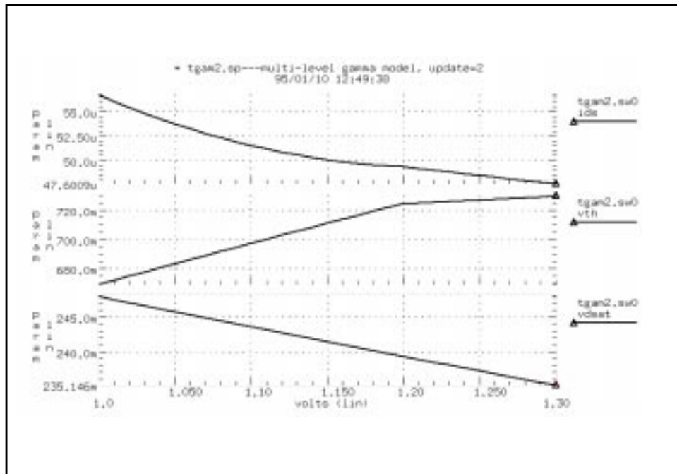
Figure 20-4: Variation of IDS, VTH and VDSAT for UPDATE=2
