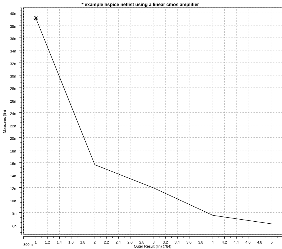
Figure E-7: Plot of User-defined Measured Variable falltime vs. Amplifier Input Voltage
