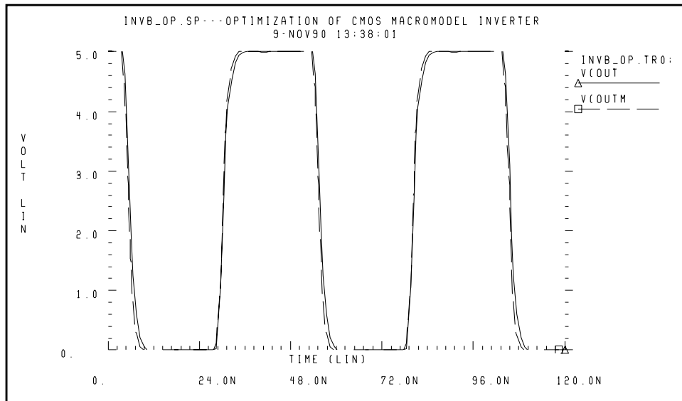
Figure 24-12: CMOS Inverter Response
