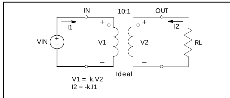
Figure 24-18: Ideal Transformer Example
