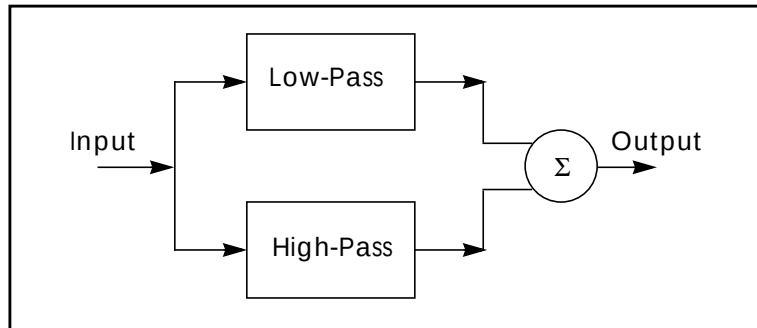
Figure 27-1: Band-Reject Filter
