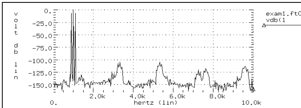
Figure 26-5: AM Modulation Spectrum
