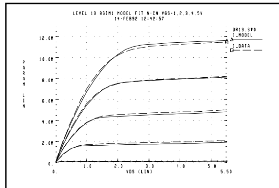
Figure 20-16: Level 13 Ids vs. Vds Curves
