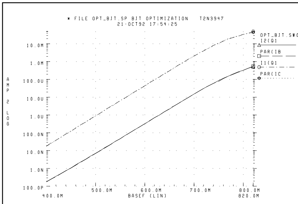
Figure 12-28: BJT Optimization Forward Gummel Plots
