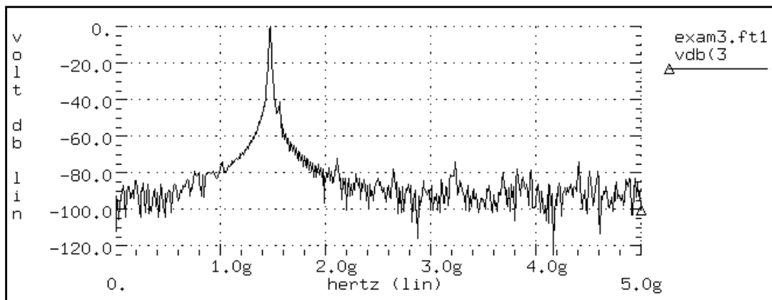
Figure 26-16: Mixer Output Spectrum, Bartlett Window
