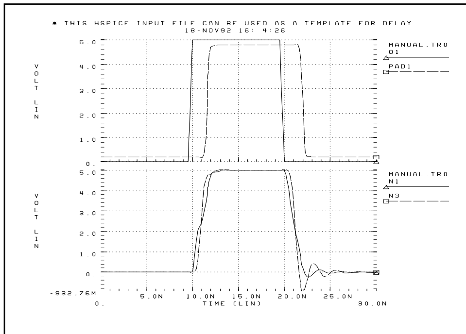
Figure 23-21: Delay Template Output
