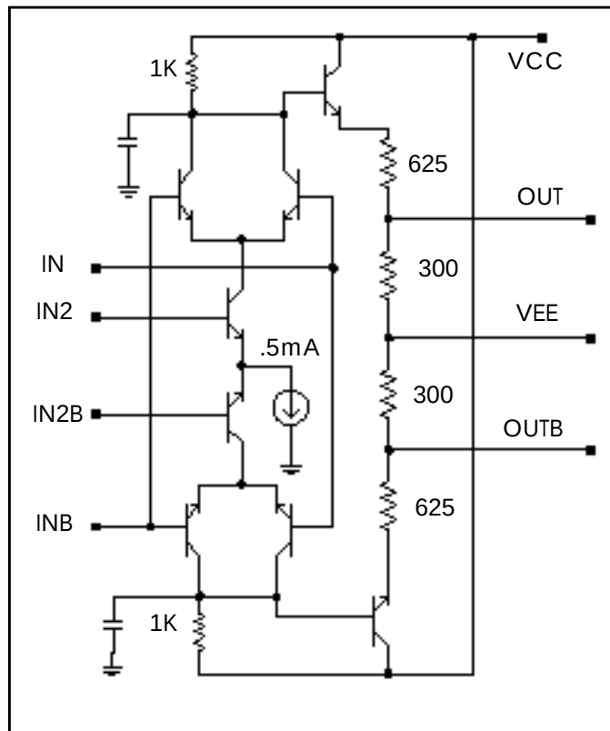
Figure 24-37: Phase Detector Circuit
