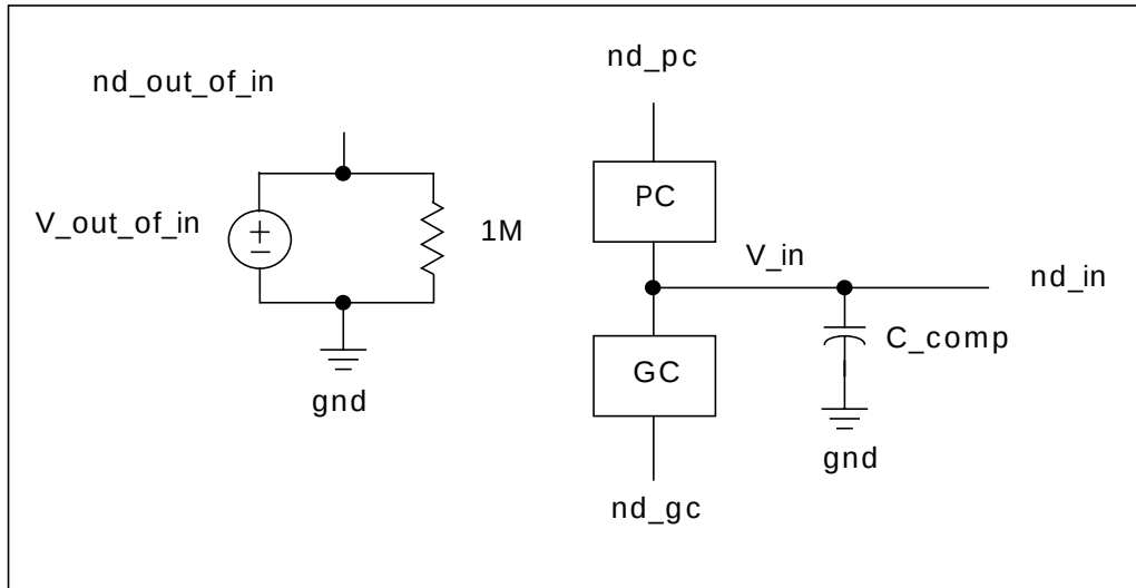
Figure 18-2: Input Buffer
