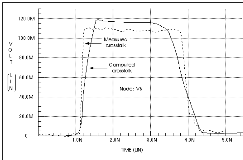
Figure B-25: Measured Versus Computed Backward Crosstalk Response
