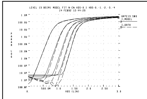
Figure 20-28: Level 13 Ids vs. Vgs Curves
