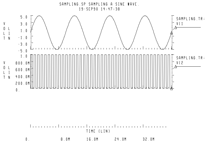
Figure 24-23: Sampled Data
