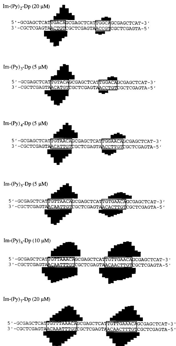
FIG. 5. Histograms of cleavage protection from MPE-Fe(II) for Im-(Py) 2 -Dp, Im-(Py) 3 -Dp, Im-(Py) 4 -Dp, Im-(Py) 5 -Dp, Im-(Py) 6 -Dp, and Im-(Py) 7 -Dp binding to the Eco RI/ Pvu II restriction fragments from plasmids pJK5, pJK6, pJK7, pJK8, pJK9, and pJK10, respectively. The individual bar heights are proportional to the protection from MPE-Fe(II) cleavage at each nucleotide. The match and mismatch sites are indicated by boxes.
