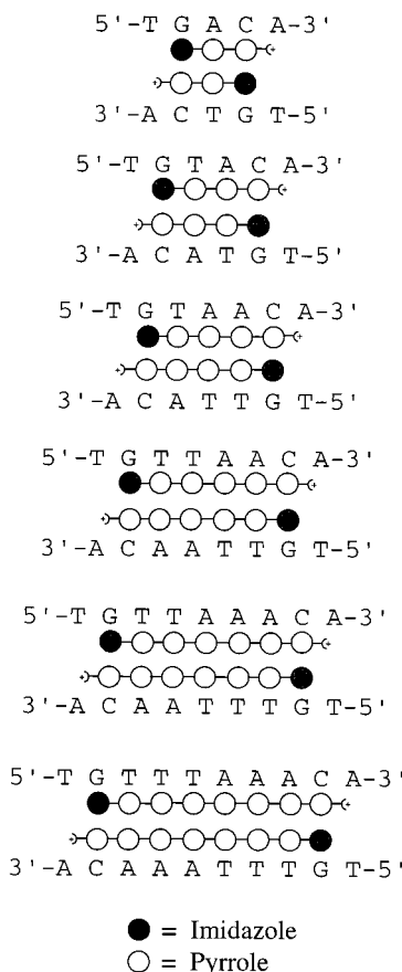
FIG. 2. Proposed 2:1 binding models of Im-(Py) 2 -Dp, Im-(Py) 3 -Dp, Im-(Py) 4 -Dp, Im-(Py) 5 -Dp, Im-(Py) 6 -Dp, and Im-(Py) 7 -Dp binding to 5-, 6-, 7-, 8-, 9-, and 10-bp match sites, respectively. The imidazole and pyrrole rings are represented as shaded and unshaded spheres, respectively.
