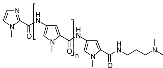
Im-(Py) 2 -Dp, 1 , n = 1 Im-(Py) 3 -Dp, 2 , n = 2 Im-(Py) 4 -Dp, 3 , n = 3 Im-(Py) 5 -Dp, 4 , n = 4 Im-(Py) 6 -Dp, 5 , n = 5 Im-(Py) 7 -Dp, 6 , n = 6
