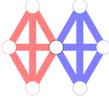
Figure 3.1: The parts of G corresponding to the two cliques from Corollary 3.10.
