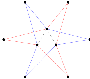
Figure 3.4: Applying Theorem 3.8 gives many copies of H \odot_2 (H, h) in which the central copy of H is green-forced.
