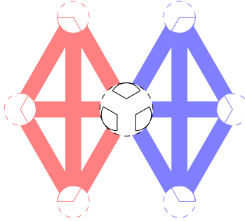
Figure 3.2: We divide the central part into v(H) subsets and shrink the other parts accordingly.
