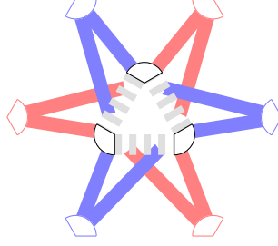
Figure 3.3: We imagine a copy of H between the subsets of the central part, with each edge supporting both a red and a blue copy of H \setminus h using the parts from the red and blue cliques.
