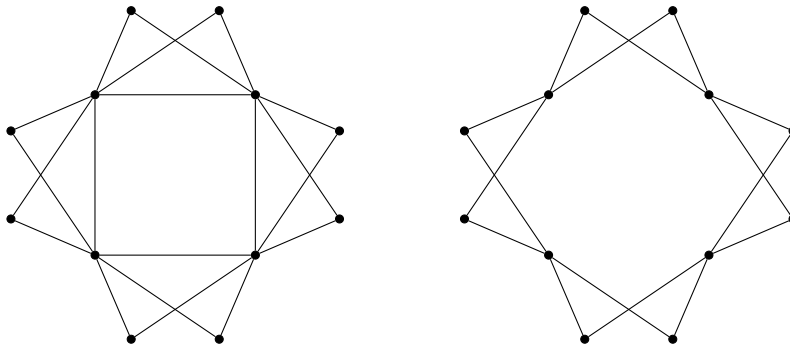
Figure 2.1: C_4 \ominus_2 K_3 (on the left) and C_4 \odot_2 K_3 (on the right).
