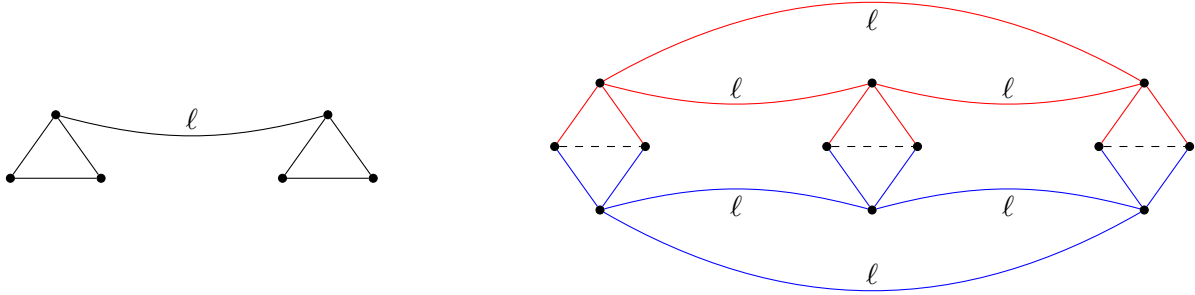
Figure 4.1: H , drawn on the left, consists of two triangles joined by a path of length \ell . On the right, F_{red} is drawn in red, F_{blue} in blue and the matching M is drawn with dashed lines.
