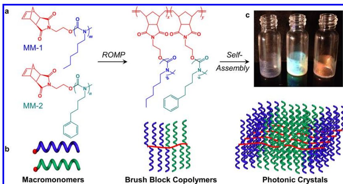
Figure 1. (a) Structures of isocyanate-based macromonomers and their ROMP to brush block copolymers. (b) Schematic representation of the synthesis of brush block copolymers from rigid-rod helical macromonomers and their self-assembly toward 1D photonic crystals. (c) Photograph of photonic crystals reflecting violet, green, and red light.
