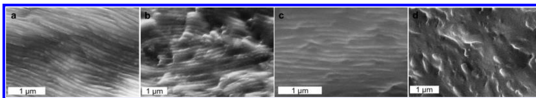
Figure 4. SEM images of cross sections of brush block copolymers with M_w = 1512 (a), 2918 (b), 4167 (c), and 5319 (d) kDa. The perspective places the glass substrate parallel with the text.
