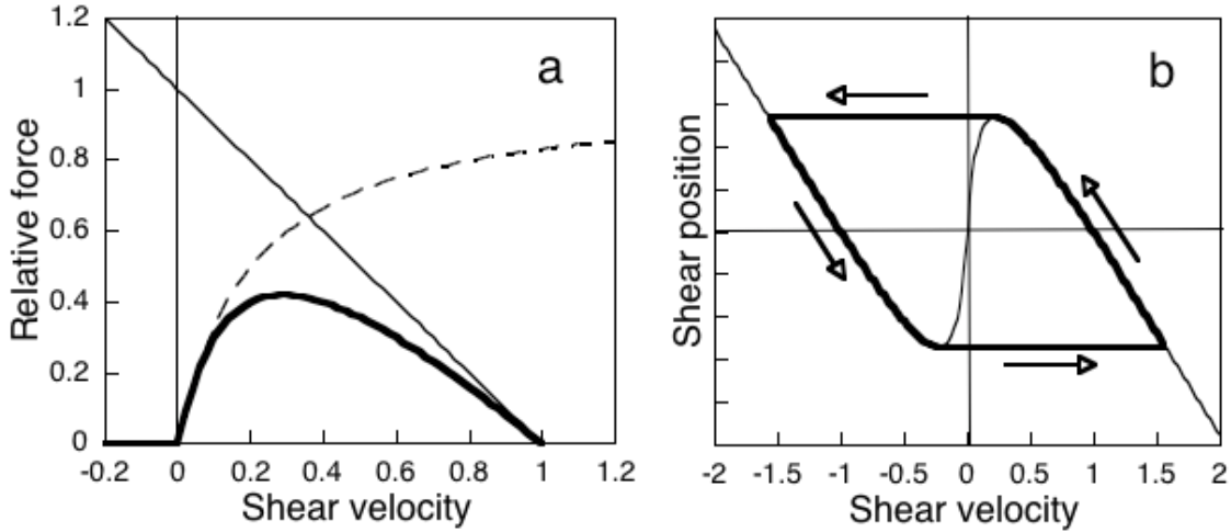
FIGURE 2. Steady-state behavior of a simple model for shear force generation. (a) The thin straight line is the force given by Equ. 1 and 2. The dashed line is the control function given by Equ. 3. The heavy solid line is the combination of the force function and the control function. (b) Two force generators, oriented in opposite directions, combined with a linear elastic shear resistance. With linear elastic resistance, force and shear displacement are proportional, giving a plot that is a phase diagram, showing limit cycle oscillation.
