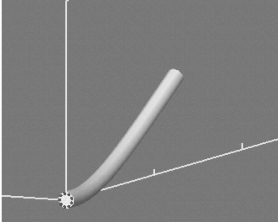
FIGURE 3. One position of a model nodal cilium that is clamped at the basal end and generating a counterclockwise circling motion. Ticks on the Z axis are at 2\ \mu\text{m} intervals, and the vertical, Y axis is 2\ \mu\text{m} tall. Length of the model is 2.6\ \mu\text{m} , circling frequency approx. 10/\text{sec} . Parameters used for this computation are the same as for the model in Fig. 2d of [14], except for E_B = 1.5 \times 10^8\ \text{pN nm}^2 and the elastic constant for non-linear shear elasticity is E_S = 44\ \text{pN} (Equ. 4). Computed with 13 length segments and 0.1\ \text{ms} time steps.
