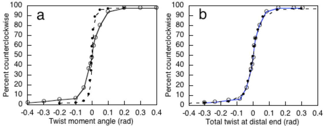
FIGURE 4. Results of computations with a nodal cilium model similar to the model shown in Fig. 3, except that the elastic shear resistance was linear, with E_s = 4 pN. The percentage of counterclockwise circling was determined from 400 computations for each point shown. Points on the solid line, from [14], were obtained with the standard twist resistance, and points on the dashed line were obtained with 25% of that twist resistance.
