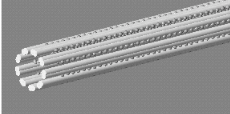
FIGURE 1. Basic elements of an axoneme, the common cytoskeleton of cilia and flagella. Nine outer microtubular doublets are arranged to form the surface of a cylinder. Dynein motor enzymes, represented here as spheres, are lined up in two rows on the A-tubule of each doublet, and produce sliding movements by interacting with the B-tubule of the adjacent doublet.
