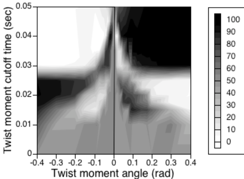
FIGURE 5. Results of computations with the nodal cilium model shown in Fig. 3. The intensity scale represents the percentage of counterclockwise circling, determined from 400 computations at each of 229 pairs of values of twist moment angle and twist moment cutoff time.
