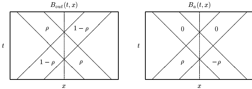
Figure 3. The total field B(t, x) can also be decomposed into an out field B_{out}(t, x) , which consists of pulses (1 - \rho(\delta)) f(t - x) and \rho(\delta) f(t + x) freely propagating to the right and left, and an advanced field B_a(t, x) , which consists of incoming pulses \rho(\delta) f(t - x) and -\rho(\delta) f(t + x) . The dotted line indicates the trajectory of the particle.
