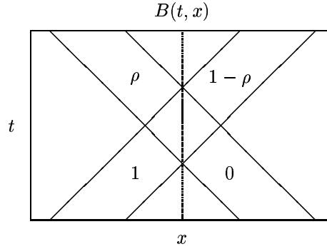
Figure 1. The total field B(t, x) : an incoming pulse f(t - x) approaches the particle from the left and scatters off it, resulting in outgoing pulses \rho(\delta) f(t + x) and (1 - \rho(\delta)) f(t - x) . The dotted line indicates the trajectory of the particle.
