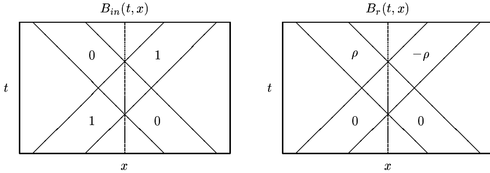
Figure 2. The total field B(t, x) can be decomposed into an in field B_{in}(t, x) , which consists of a pulse f(t - x) that freely propagates to the right, and a retarded field B_r(t, x) , which consists of outgoing pulses \rho(\delta) f(t + x) and -\rho(\delta) f(t - x) . The dotted line indicates the trajectory of the particle.
