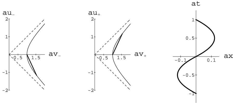
Figure 1. Test particle trajectory in the (u_-, v_-) , (u_+, v_+) , and (t, x) coordinate systems. The thick lines indicate the trajectory of the test particle; the thin lines in the (u_-, v_-) and (u_+, v_+) coordinate systems indicate the hyperbolas H_- and H_+ .
